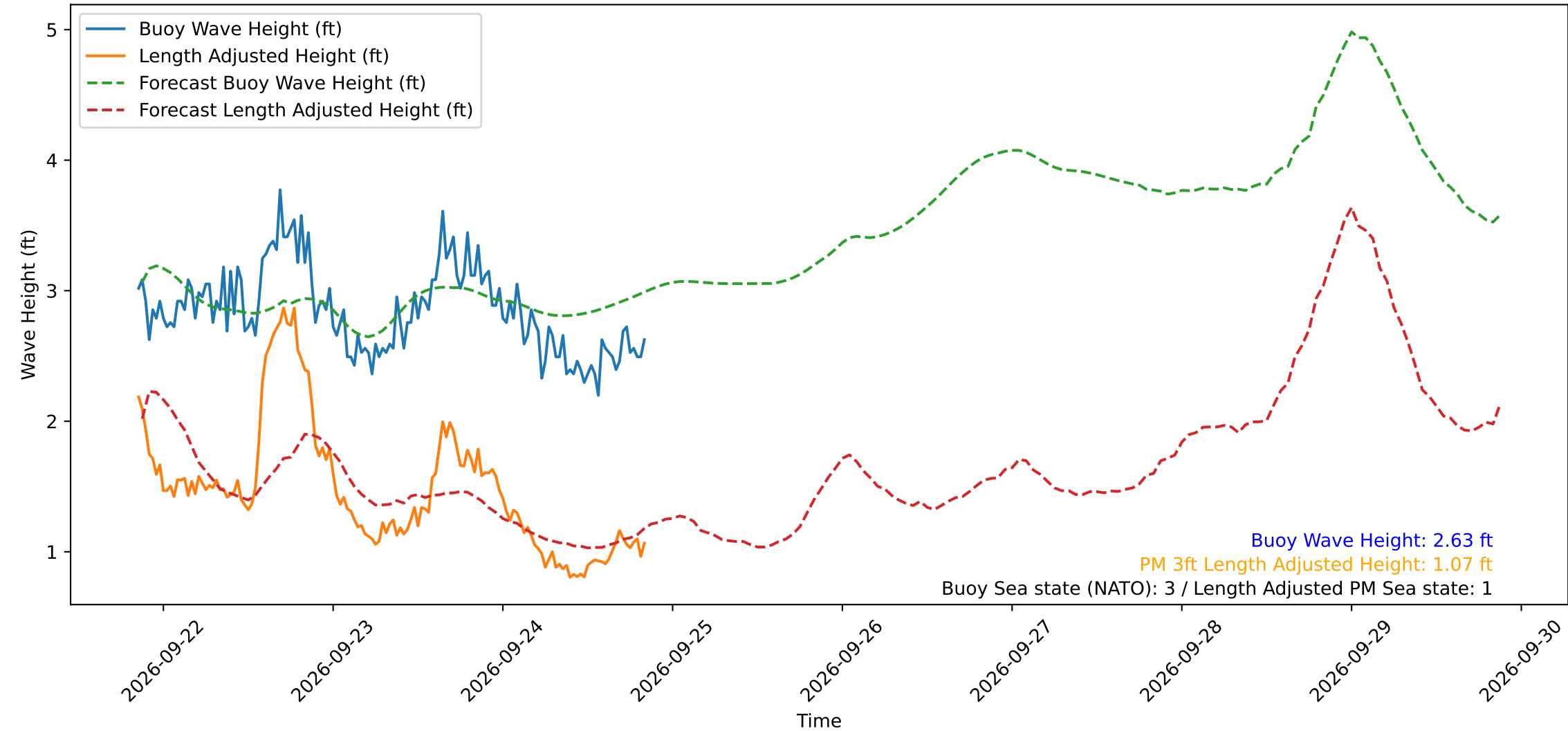
Wave Heights over Time for Oceanside Harbor at 2026-09-24 20:40:31
