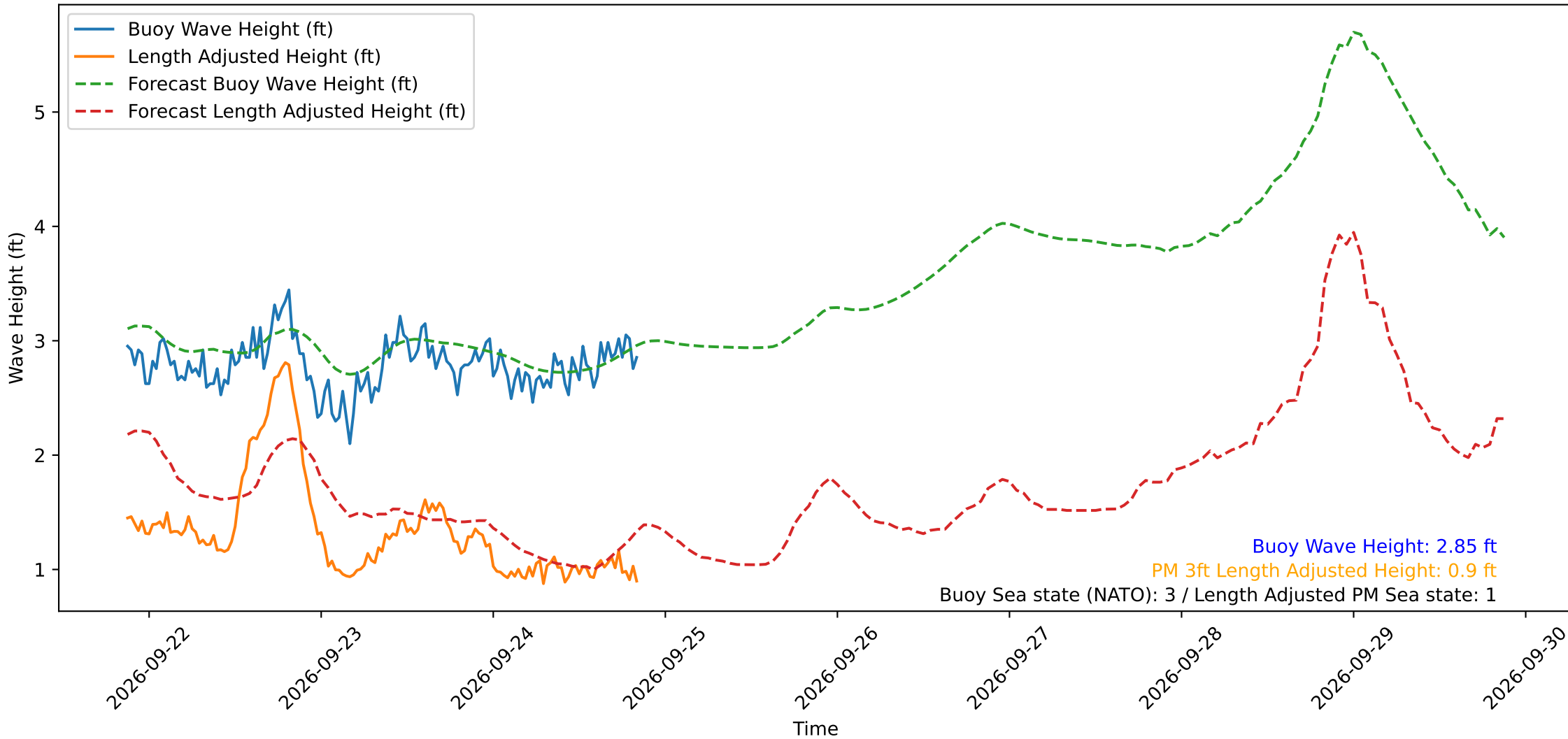
Wave Heights over Time for Green Beach at 2026-09-24 20:41:13
