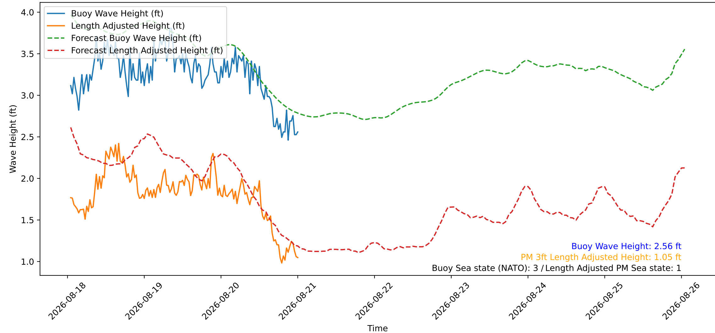
Wave Heights over Time for Oceanside Harbor at 2026-08-21 00:50:27
