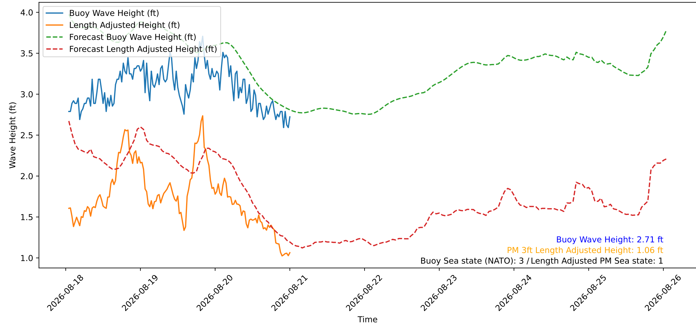
Wave Heights over Time for Green Beach at 2026-08-21 00:51:10
