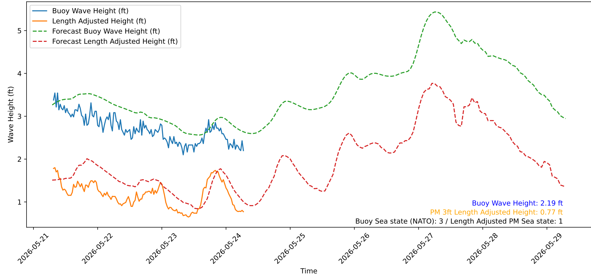
Wave Heights over Time for Green Beach at 2026-05-24 07:21:15
