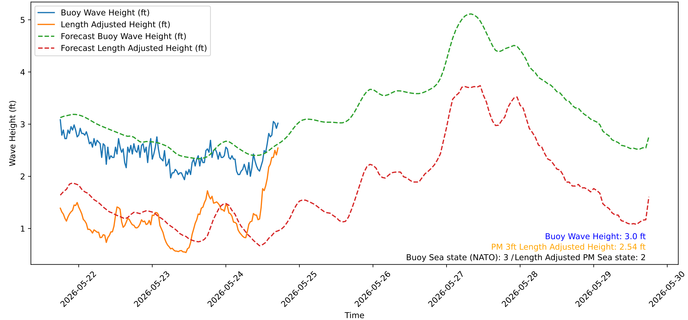
Wave Heights over Time for Red Beach at 2026-05-24 17:50:53
