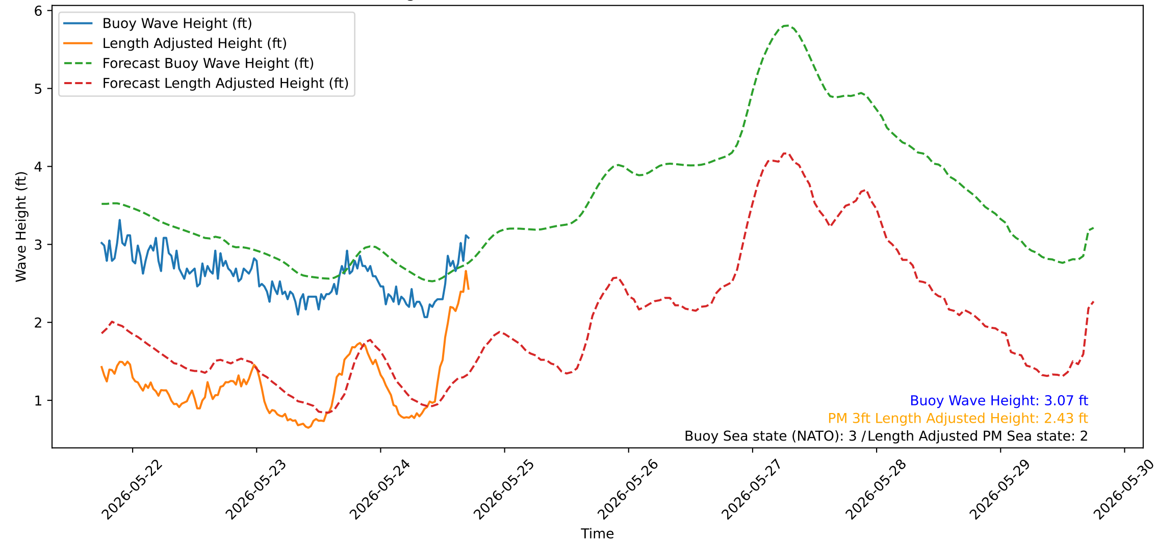
Wave Heights over Time for Green Beach at 2026-05-24 17:51:16
