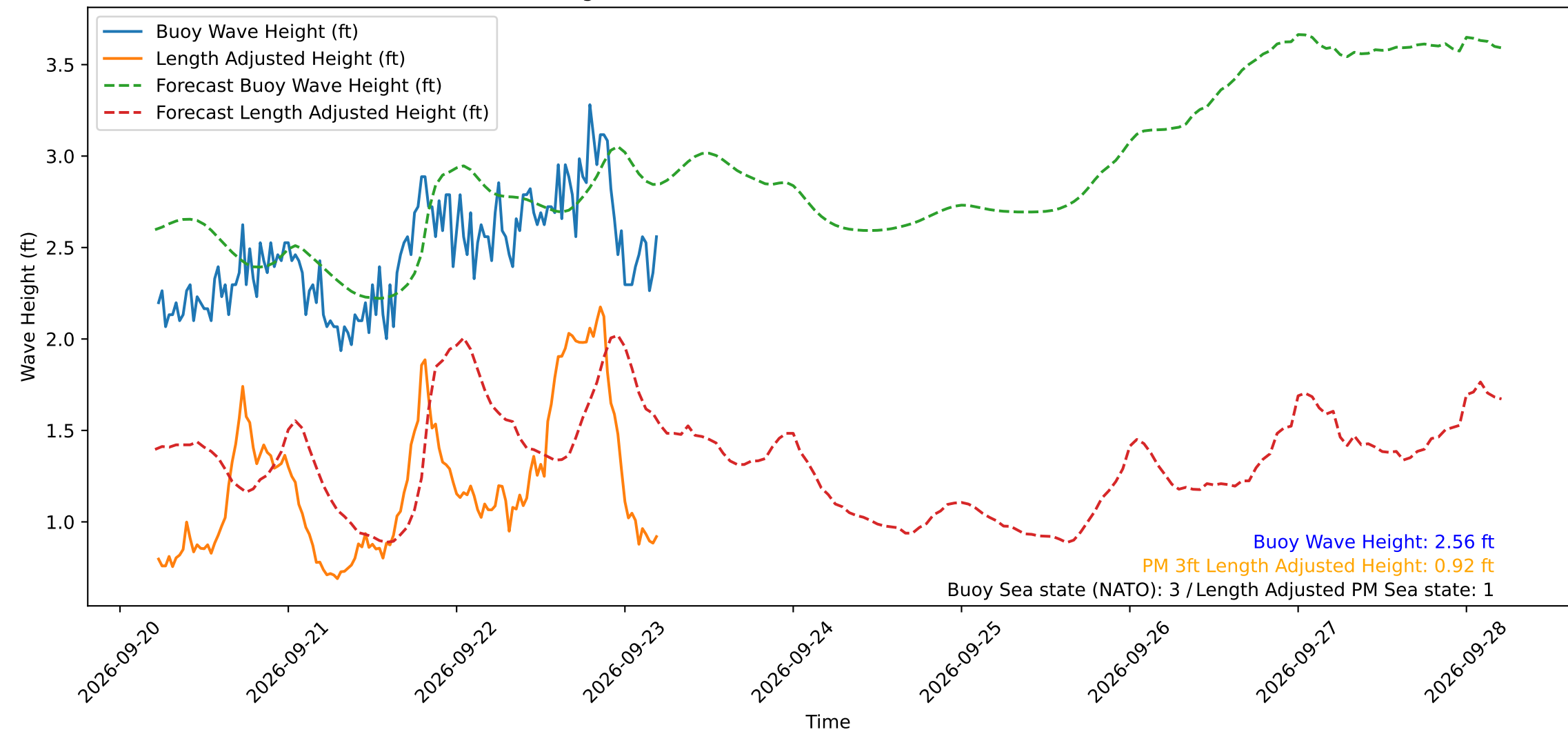
Wave Heights over Time for Red Beach at 2026-09-23 05:20:51
