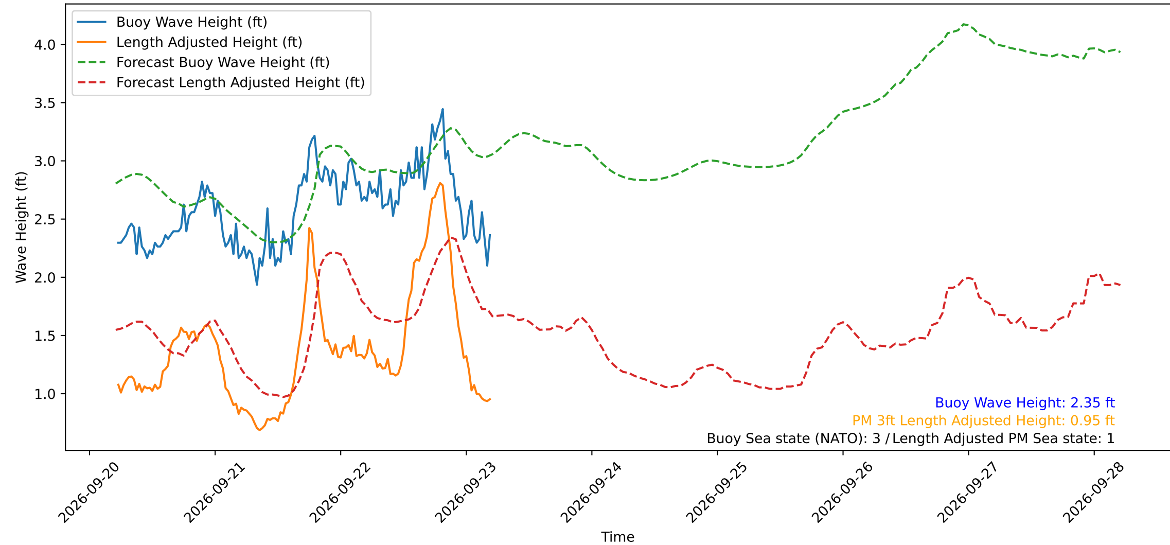
Wave Heights over Time for Green Beach at 2026-09-23 05:21:15
