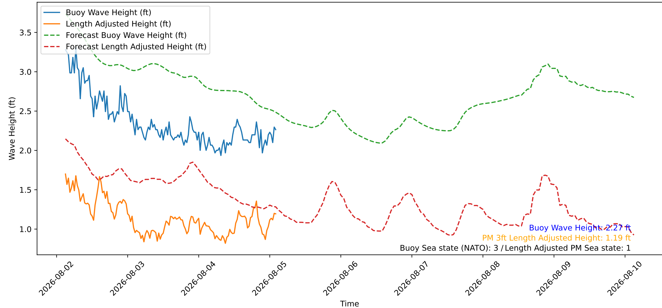
Wave Heights over Time for Green Beach at 2026-08-05 03:01:09
