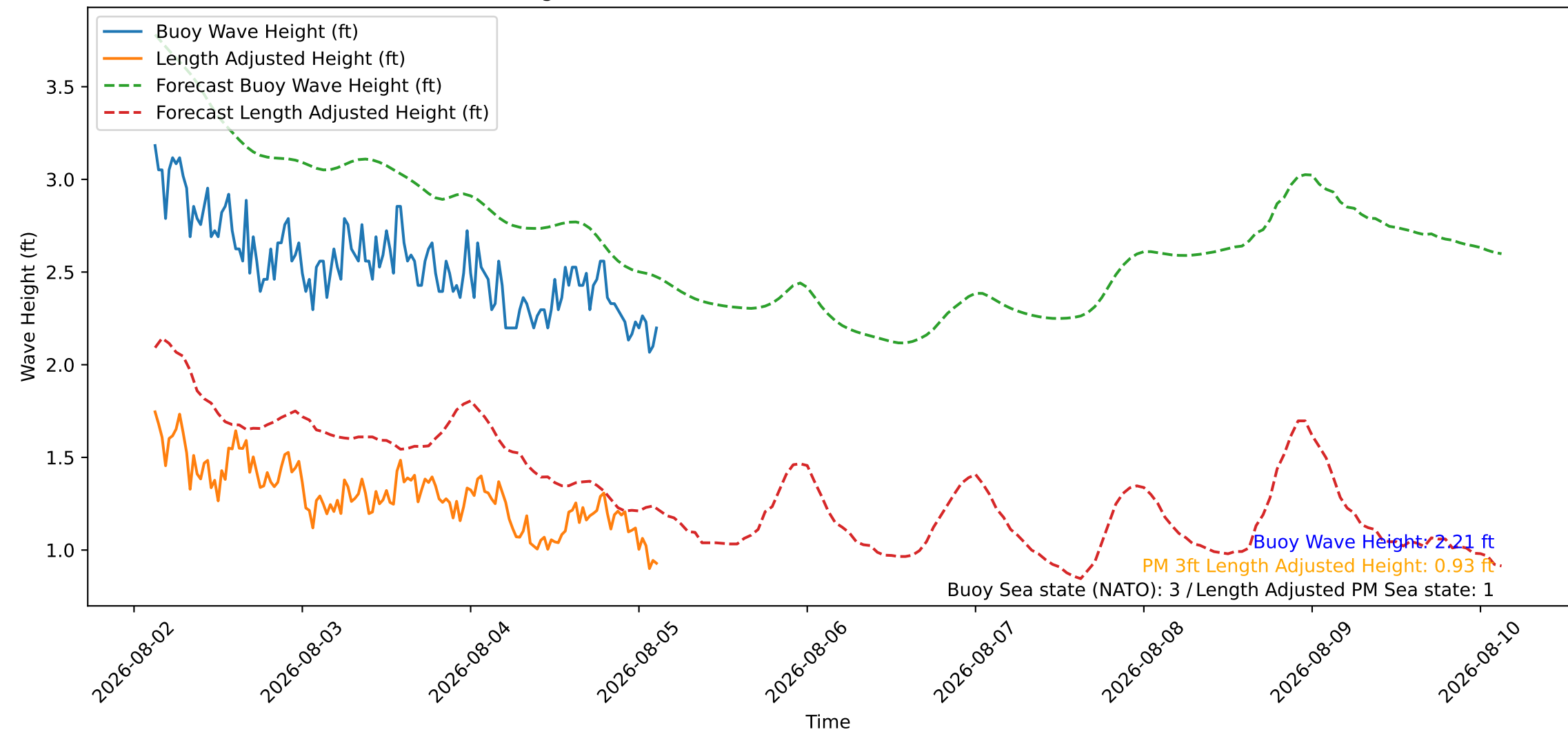
Wave Heights over Time for Oceanside Harbor at 2026-08-05 03:00:27
