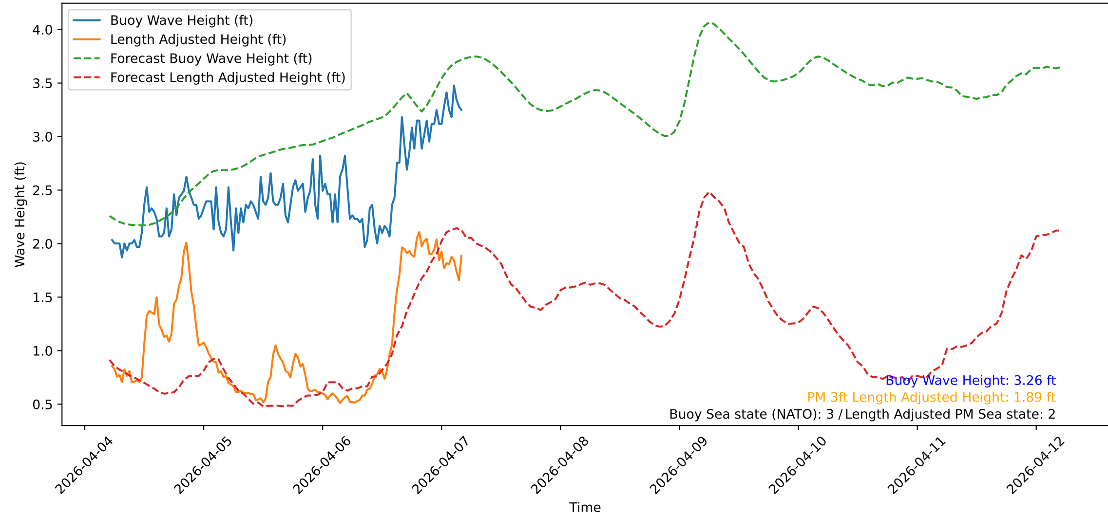
Wave Heights over Time for Red Beach at 2026-04-07 05:00:48
