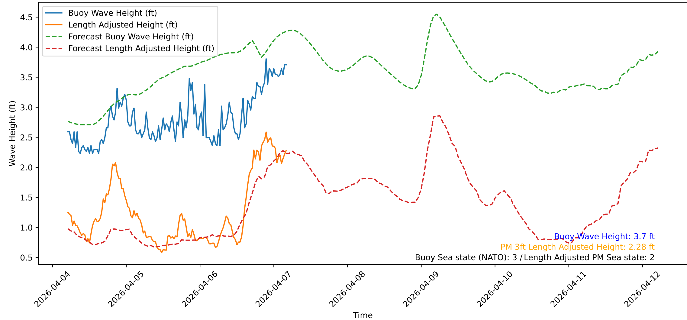
Wave Heights over Time for Green Beach at 2026-04-07 05:01:11
