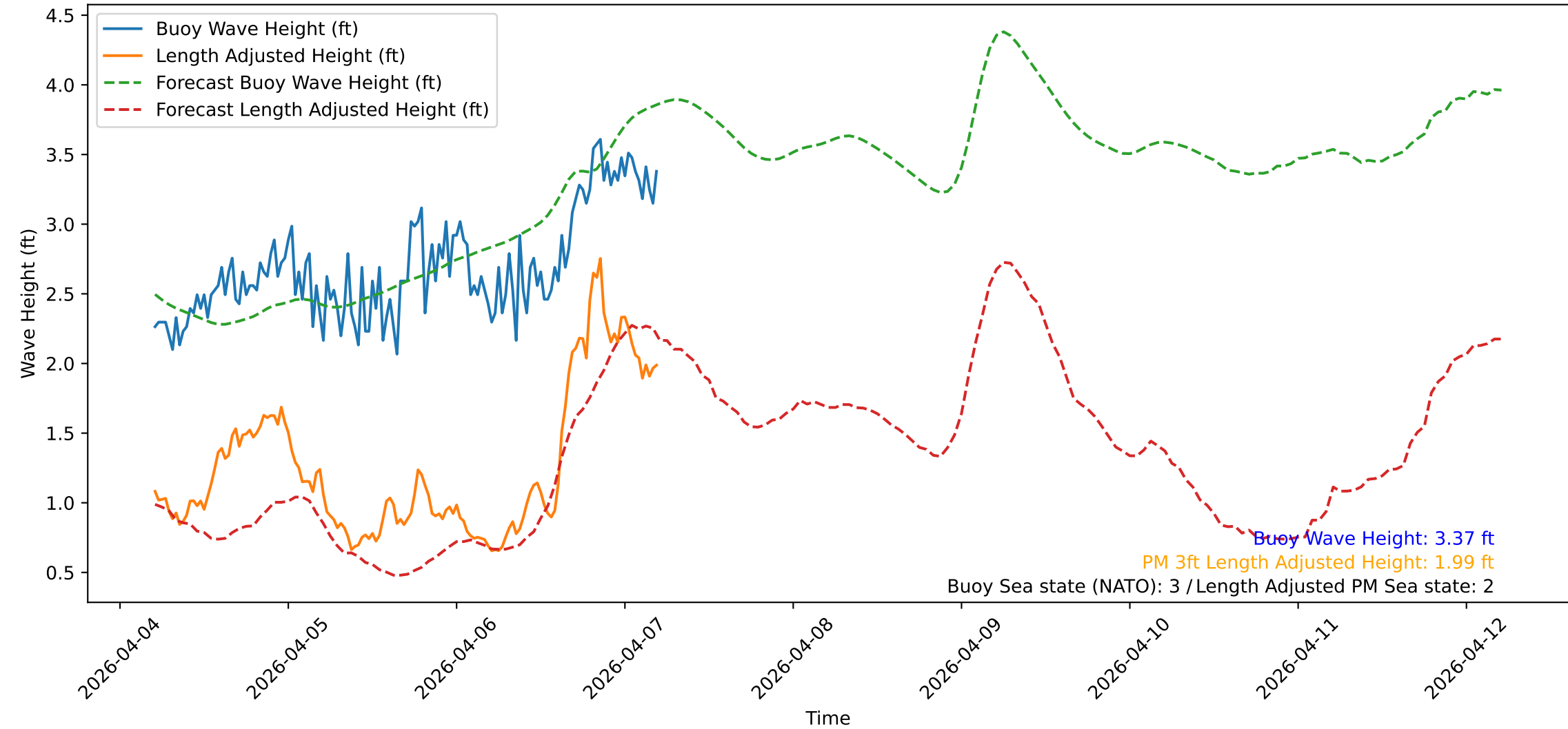
Wave Heights over Time for Oceanside Harbor at 2026-04-07 05:00:31
