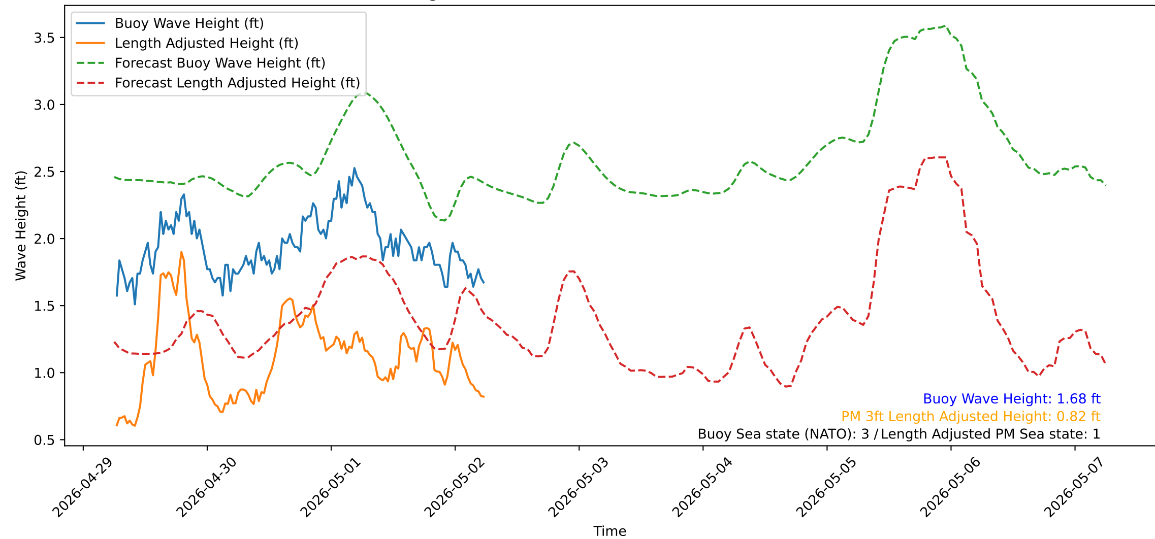
Wave Heights over Time for Red Beach at 2026-05-02 06:20:52
