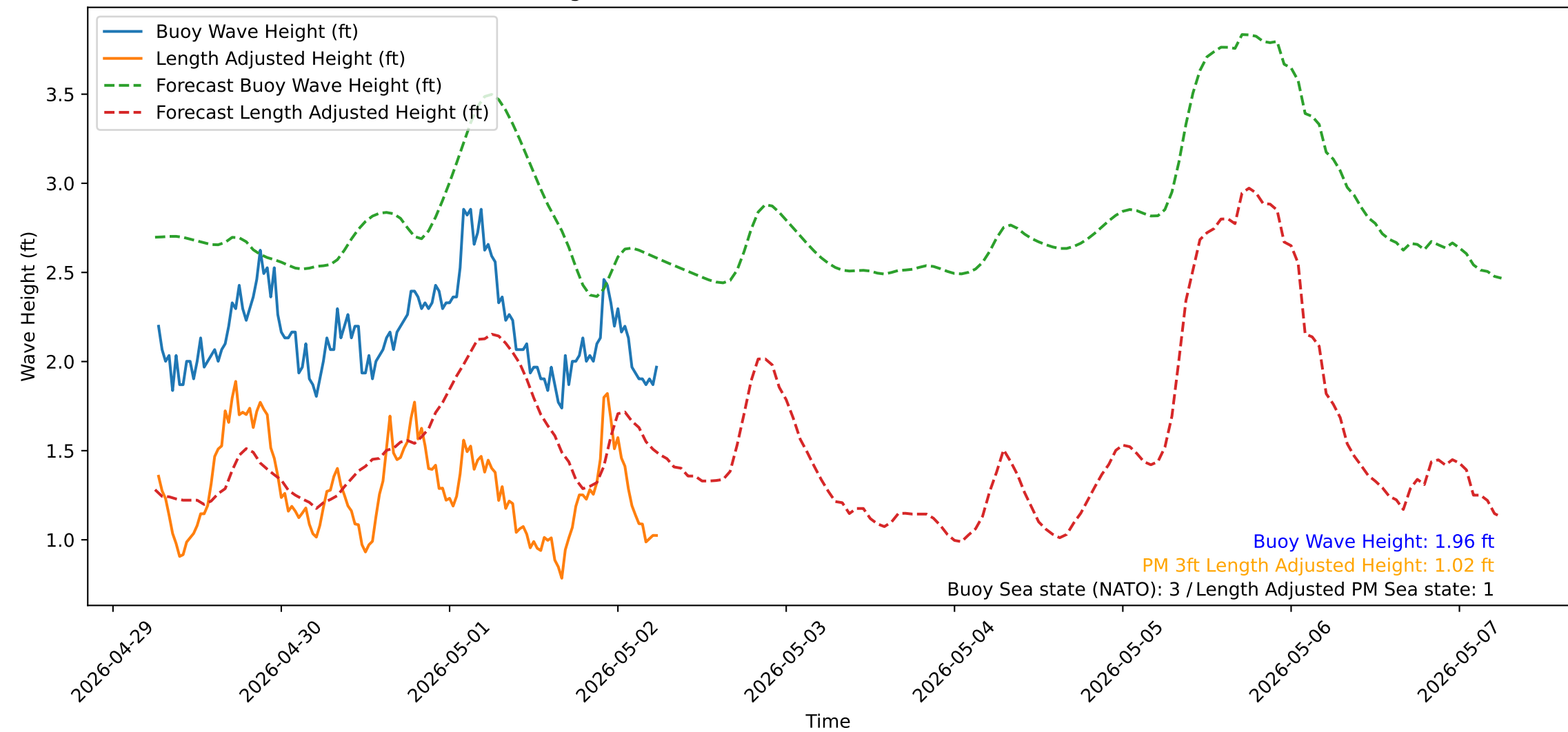
Wave Heights over Time for Green Beach at 2026-05-02 06:21:14
