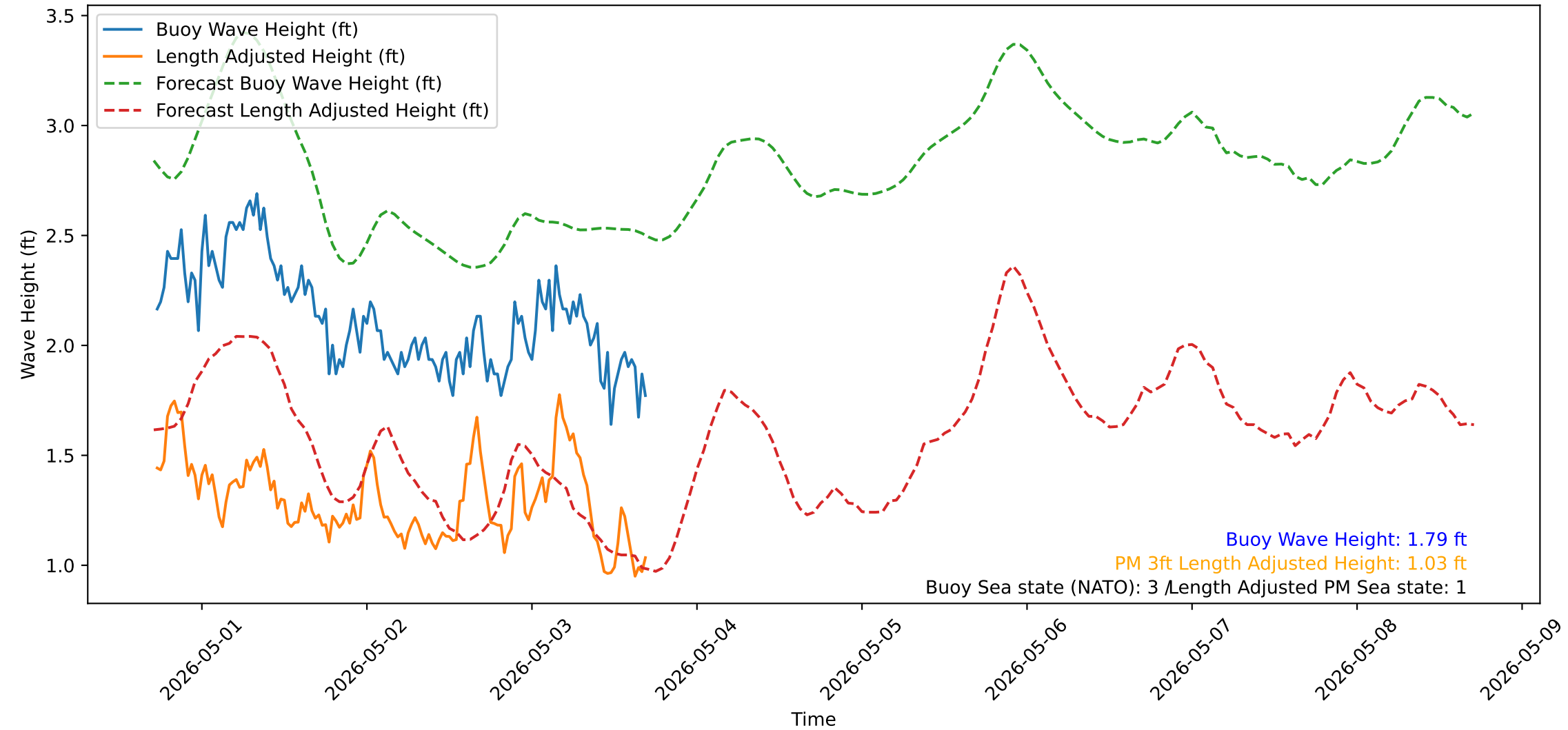
Wave Heights over Time for Oceanside Harbor at 2026-05-03 17:20:32
