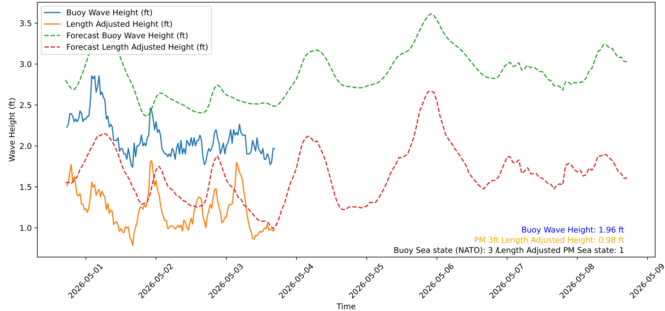
Wave Heights over Time for Green Beach at 2026-05-03 17:21:13
