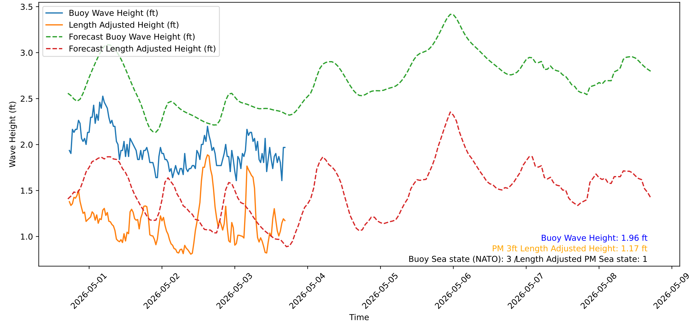
Wave Heights over Time for Red Beach at 2026-05-03 17:20:52
