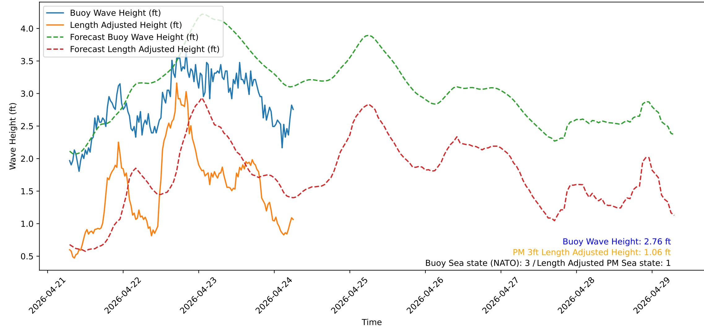
Wave Heights over Time for Red Beach at 2026-04-24 06:40:50
