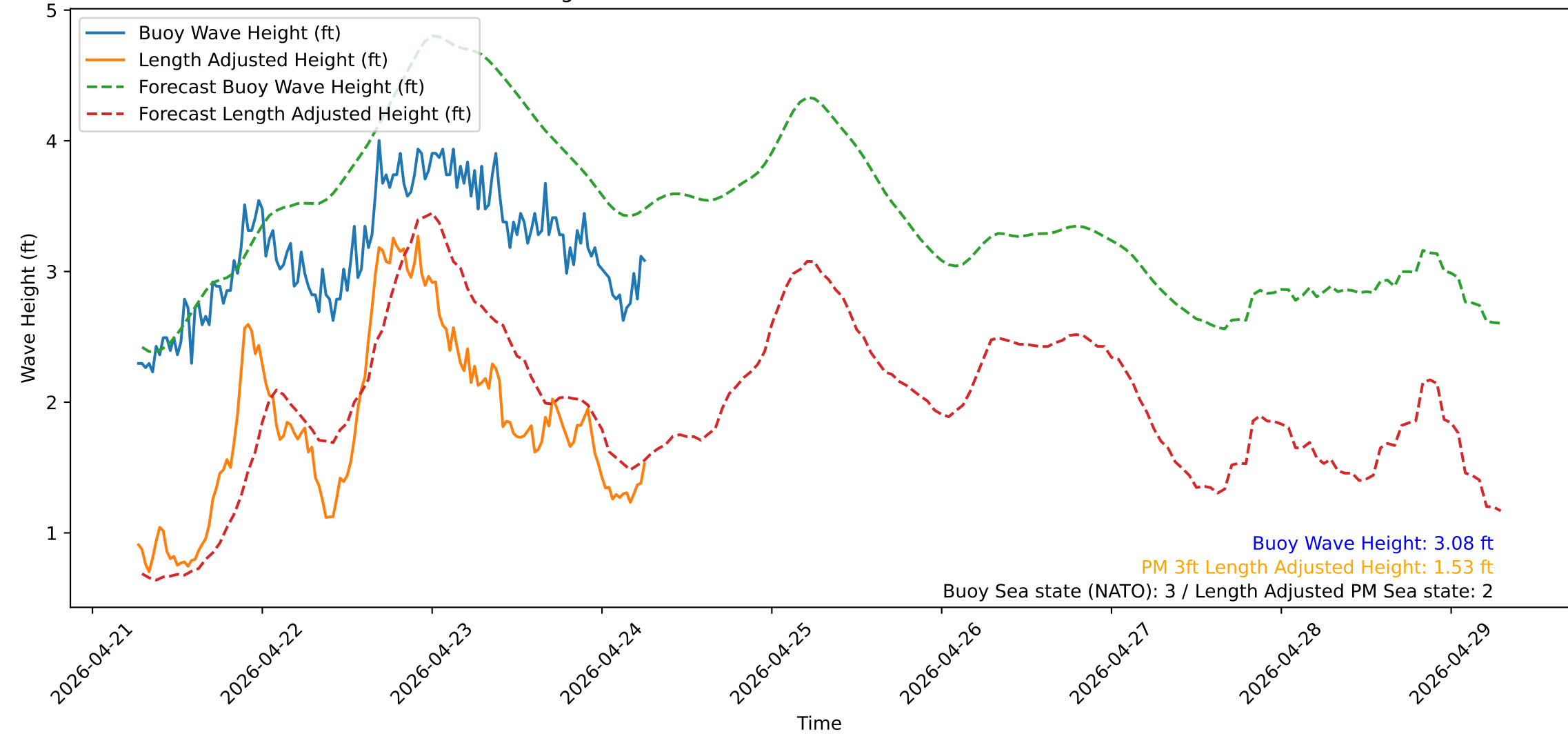
Wave Heights over Time for Green Beach at 2026-04-24 06:41:12
