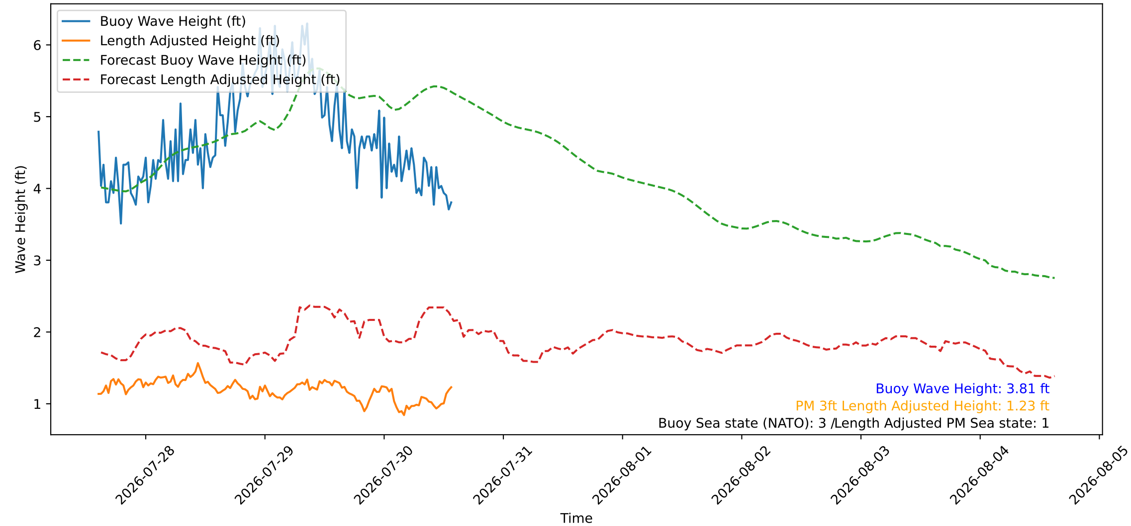
Wave Heights over Time for Green Beach at 2026-07-30 14:31:08
