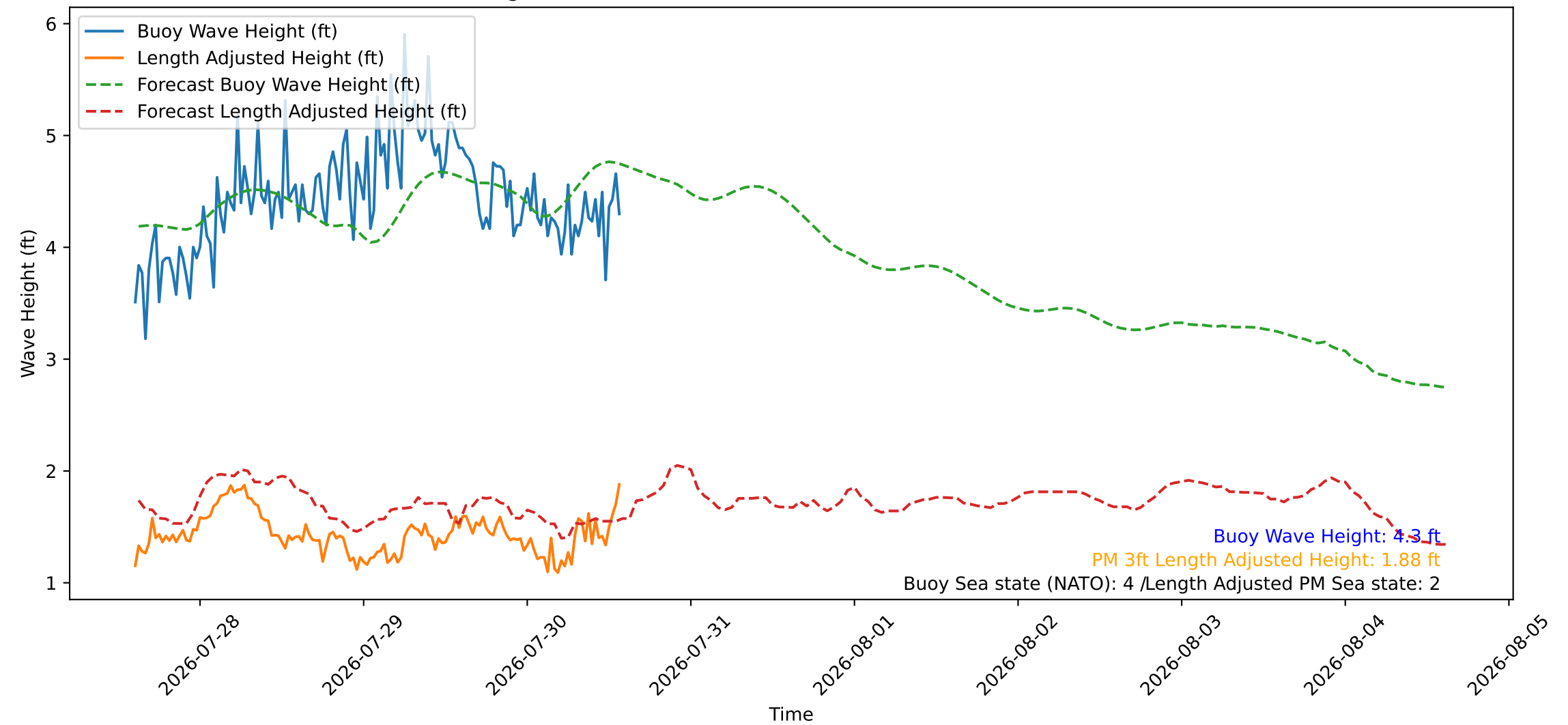
Wave Heights over Time for Oceanside Harbor at 2026-07-30 14:30:26
