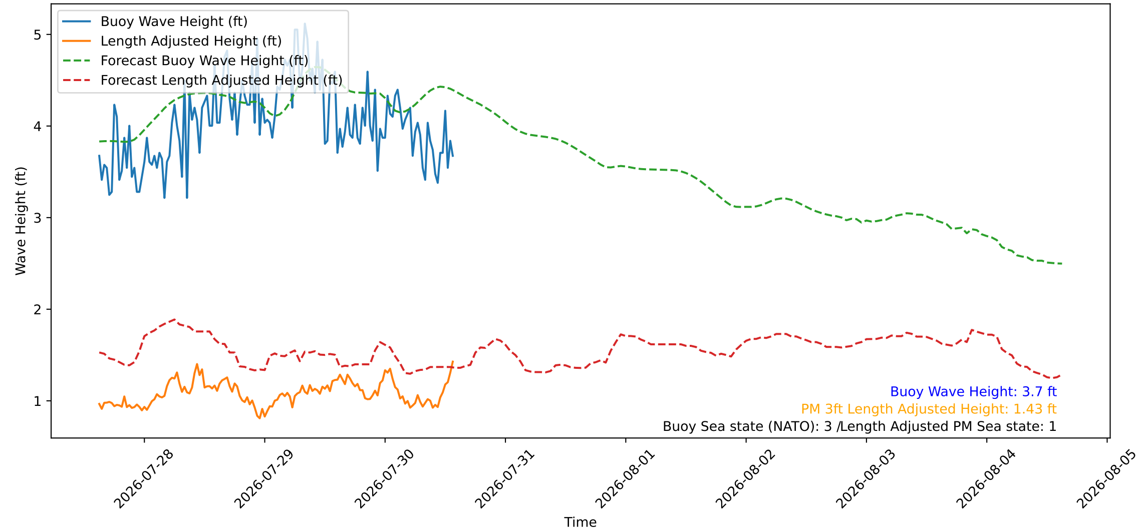
Wave Heights over Time for Red Beach at 2026-07-30 14:30:46
