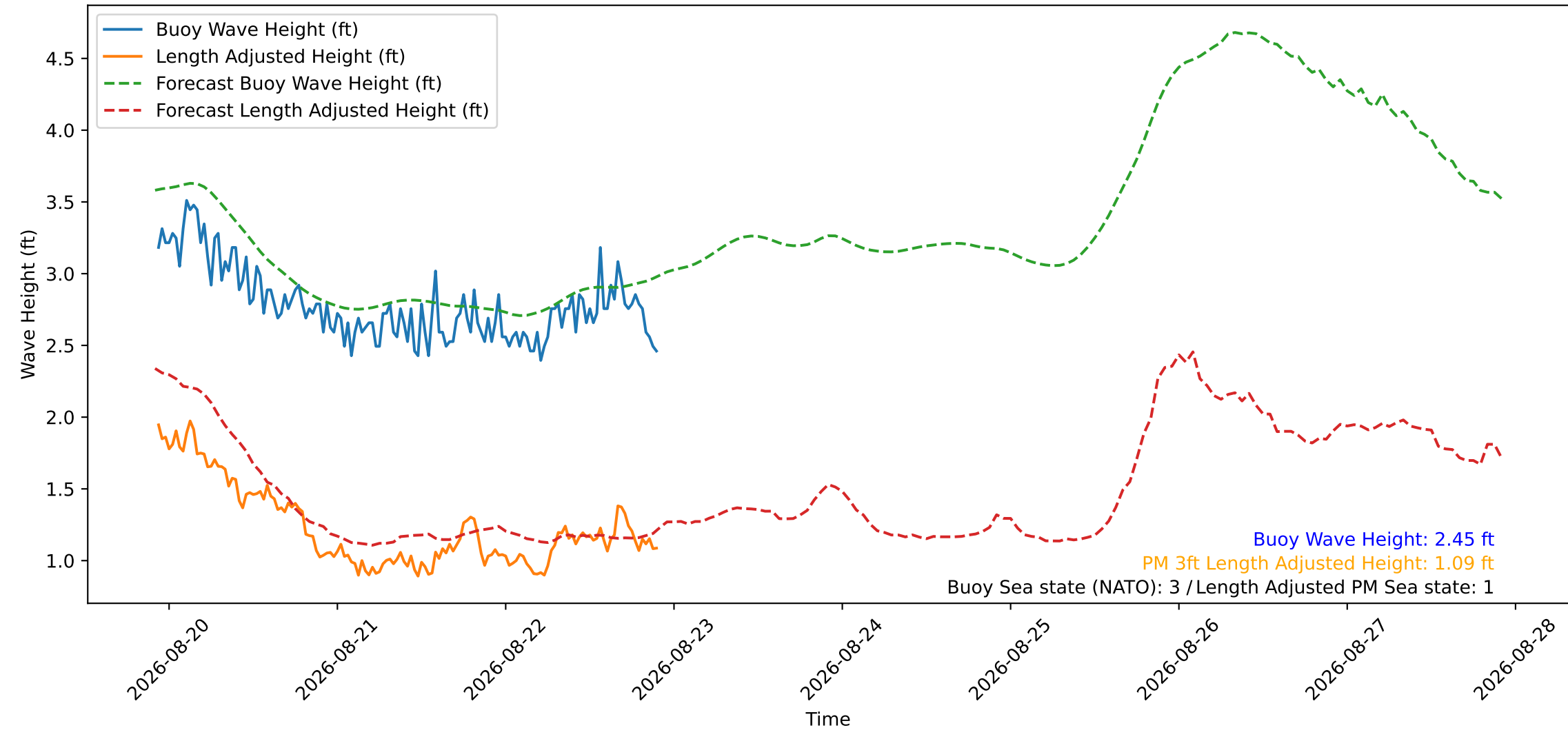
Wave Heights over Time for Green Beach at 2026-08-22 22:11:12
