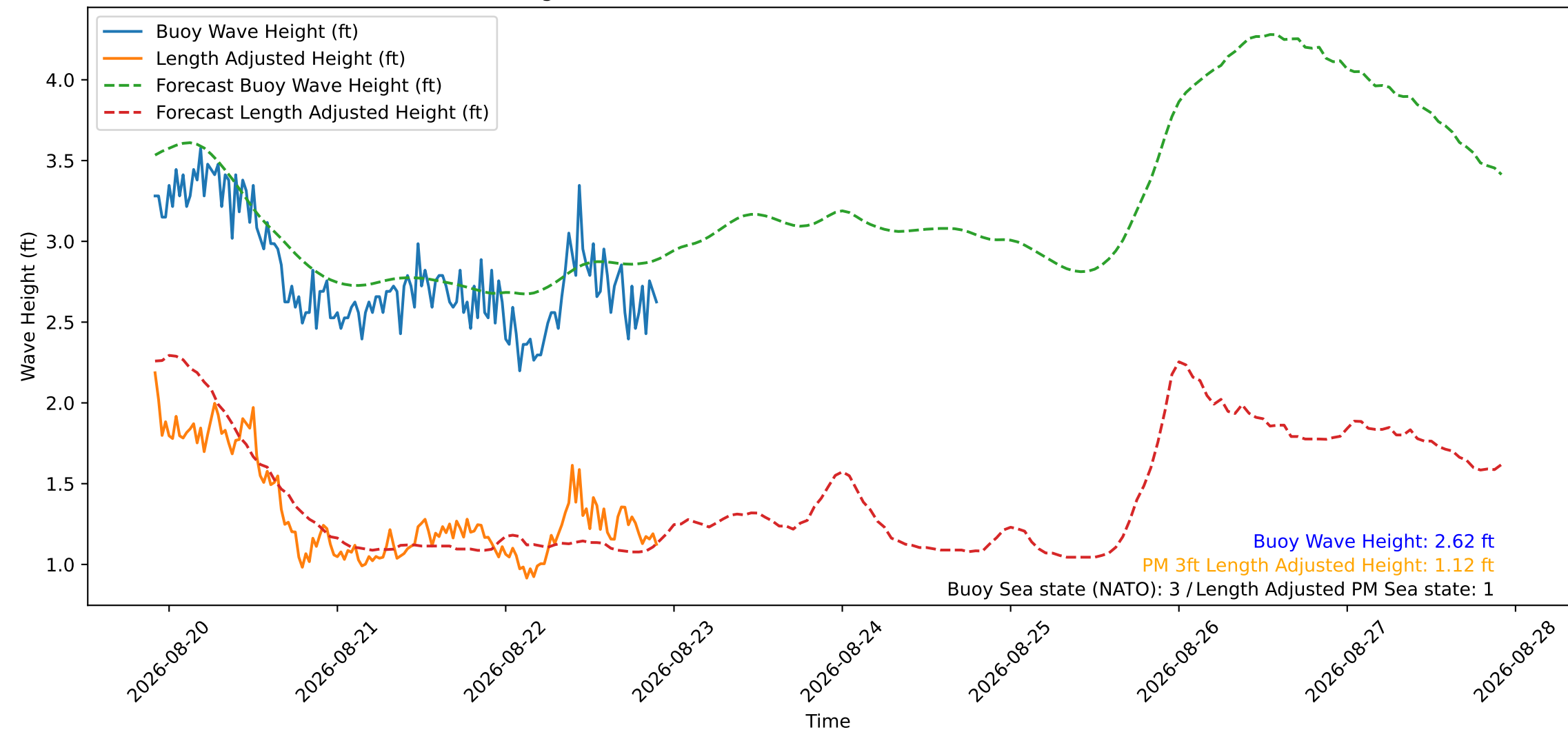
Wave Heights over Time for Oceanside Harbor at 2026-08-22 22:10:30
