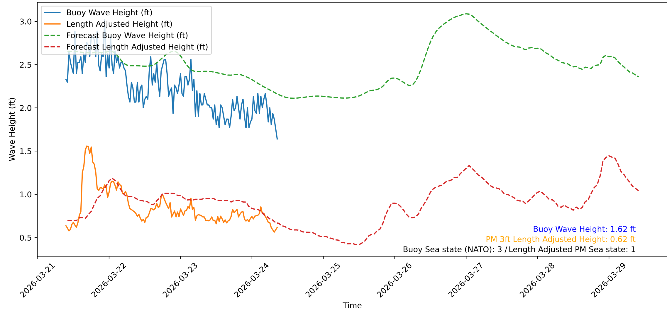
Wave Heights over Time for Oceanside Harbor at 2026-03-24 09:30:31
