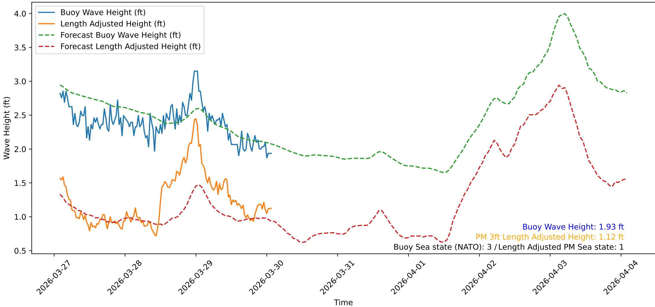
Wave Heights over Time for Oceanside Harbor at 2026-03-30 02:10:31
