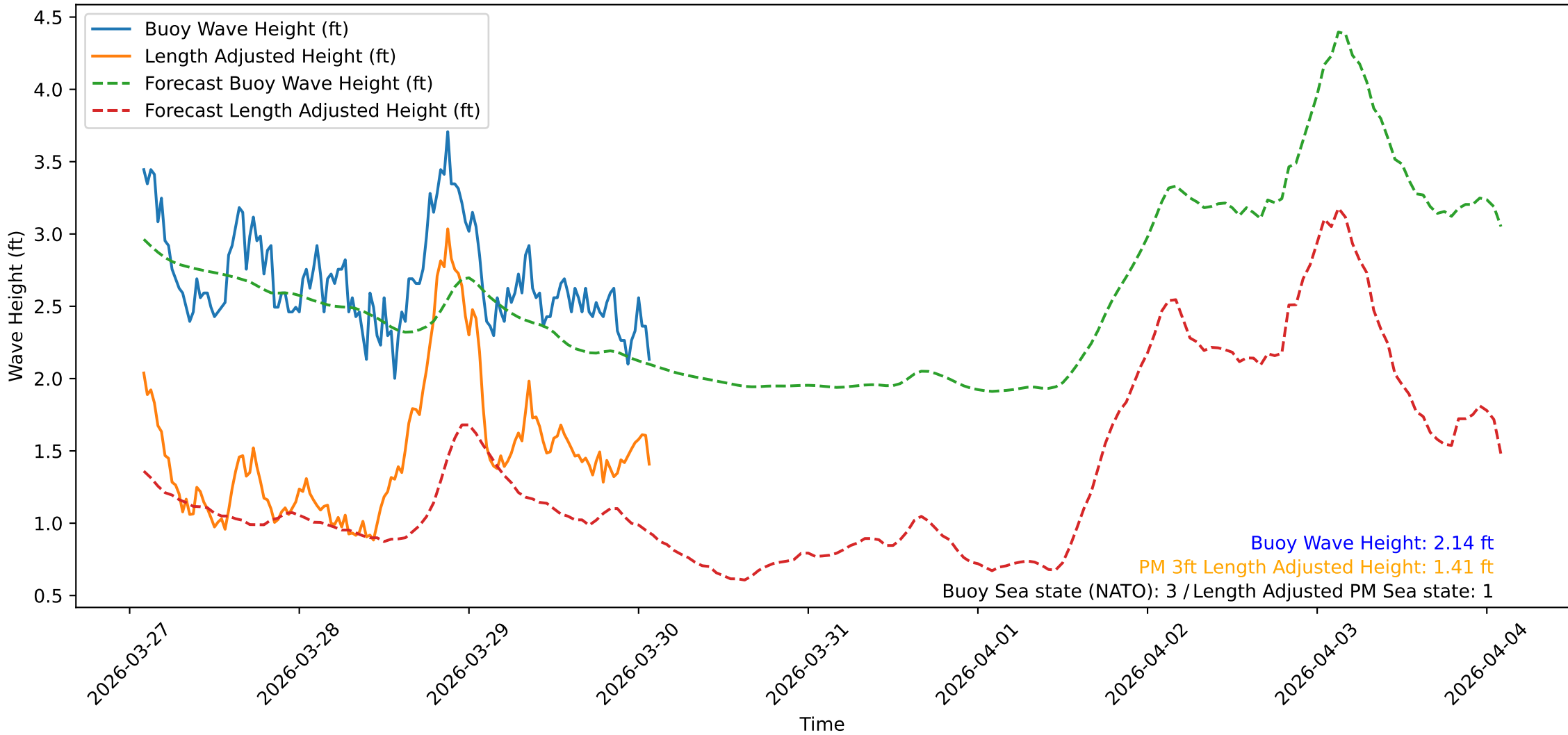
Wave Heights over Time for Green Beach at 2026-03-30 02:11:10
