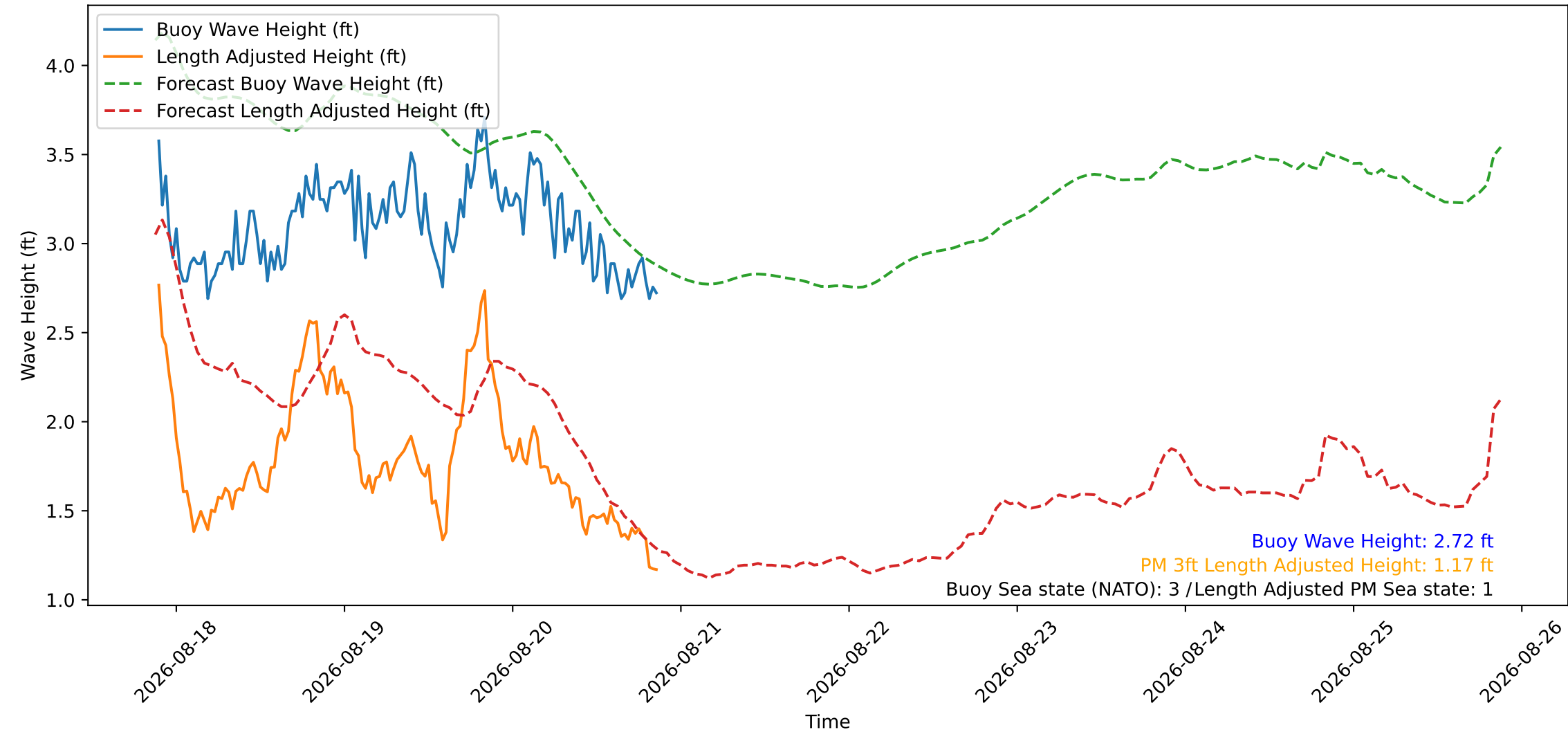
Wave Heights over Time for Green Beach at 2026-08-20 21:21:11
