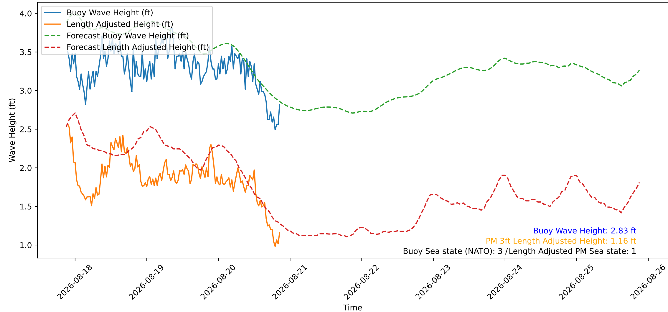
Wave Heights over Time for Oceanside Harbor at 2026-08-20 21:20:27
