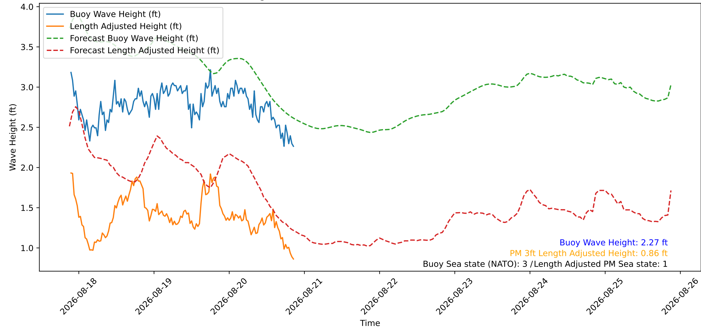
Wave Heights over Time for Red Beach at 2026-08-20 21:20:47
