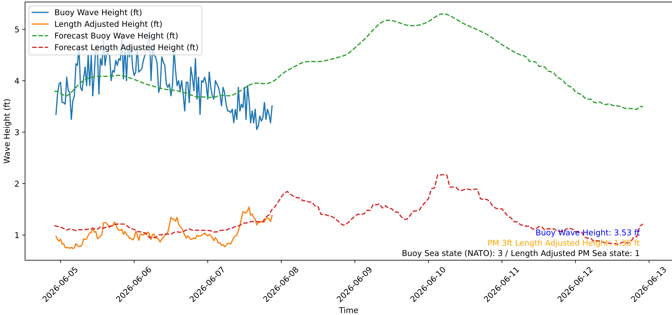
Wave Heights over Time for Red Beach at 2026-06-07 22:00:46
