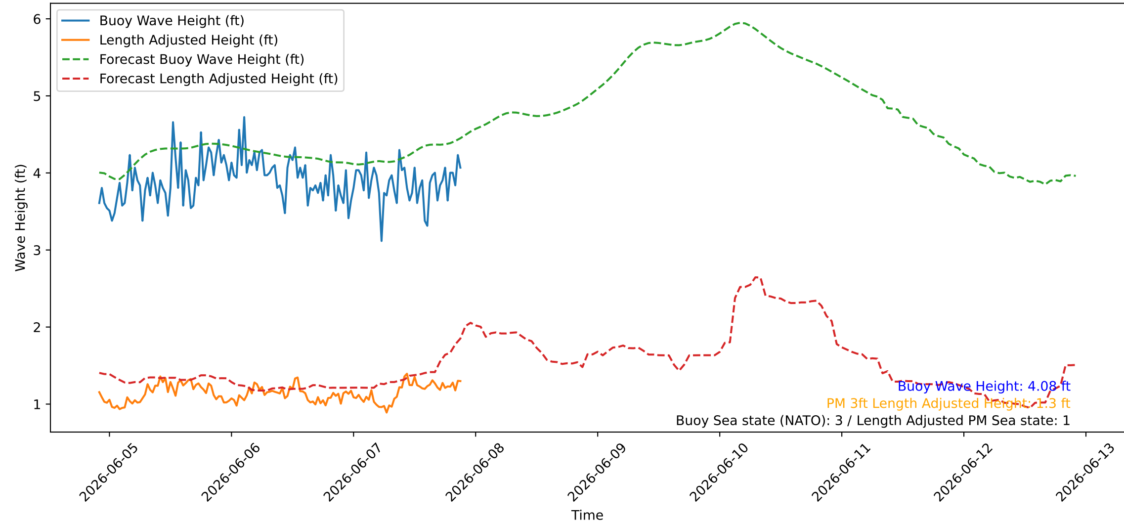
Wave Heights over Time for Green Beach at 2026-06-07 22:01:08
