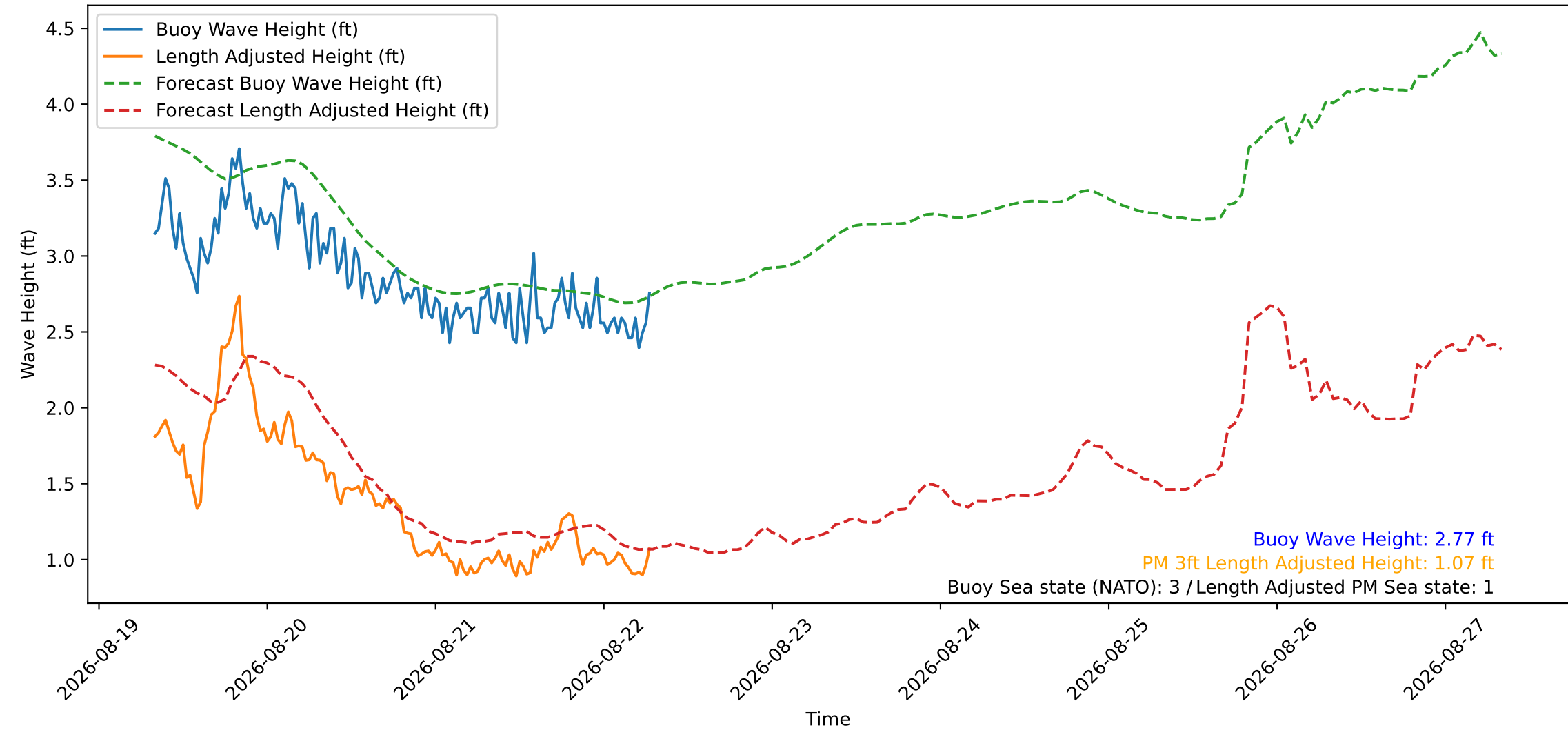
Wave Heights over Time for Green Beach at 2026-08-22 07:31:12
