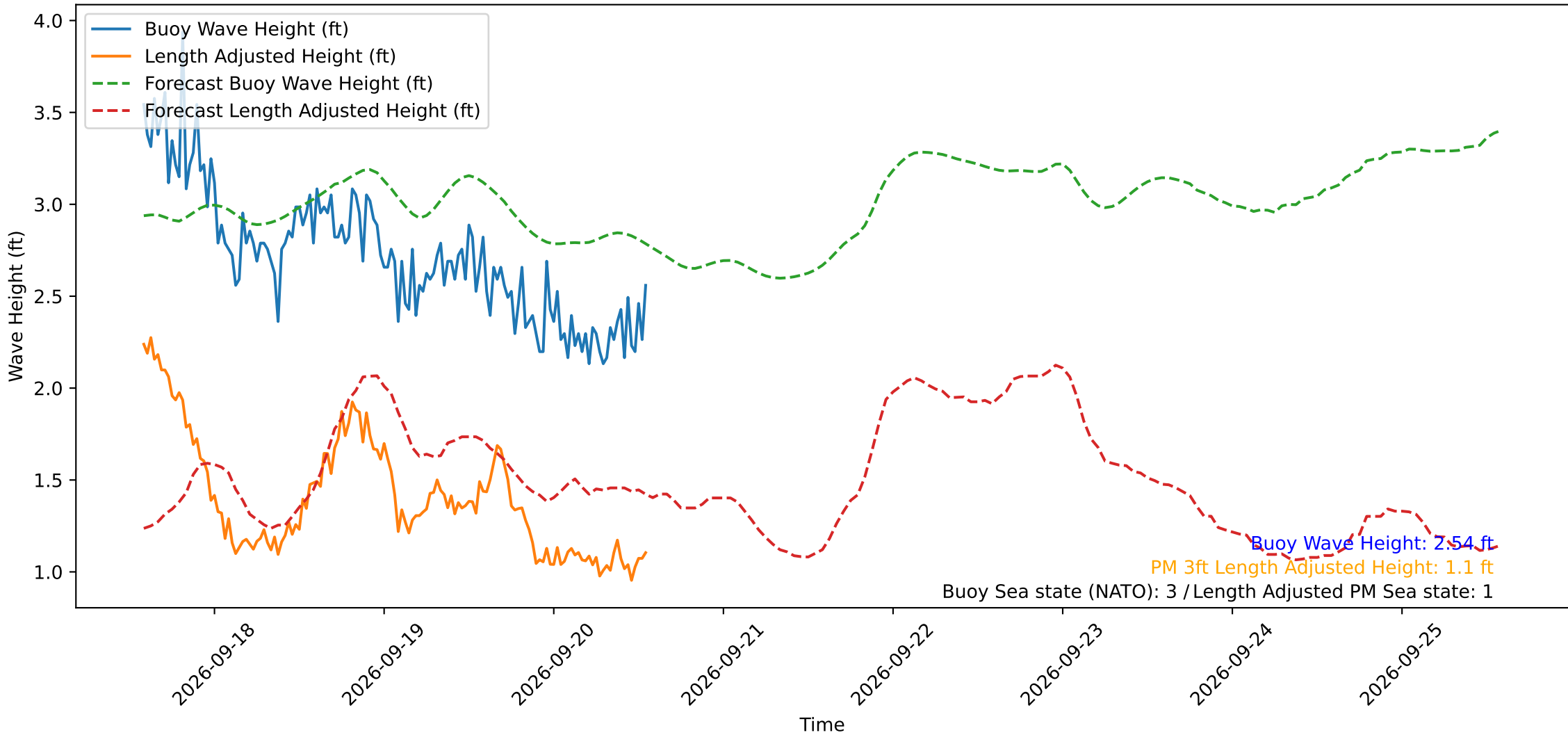
Wave Heights over Time for Oceanside Harbor at 2026-09-20 13:50:30
