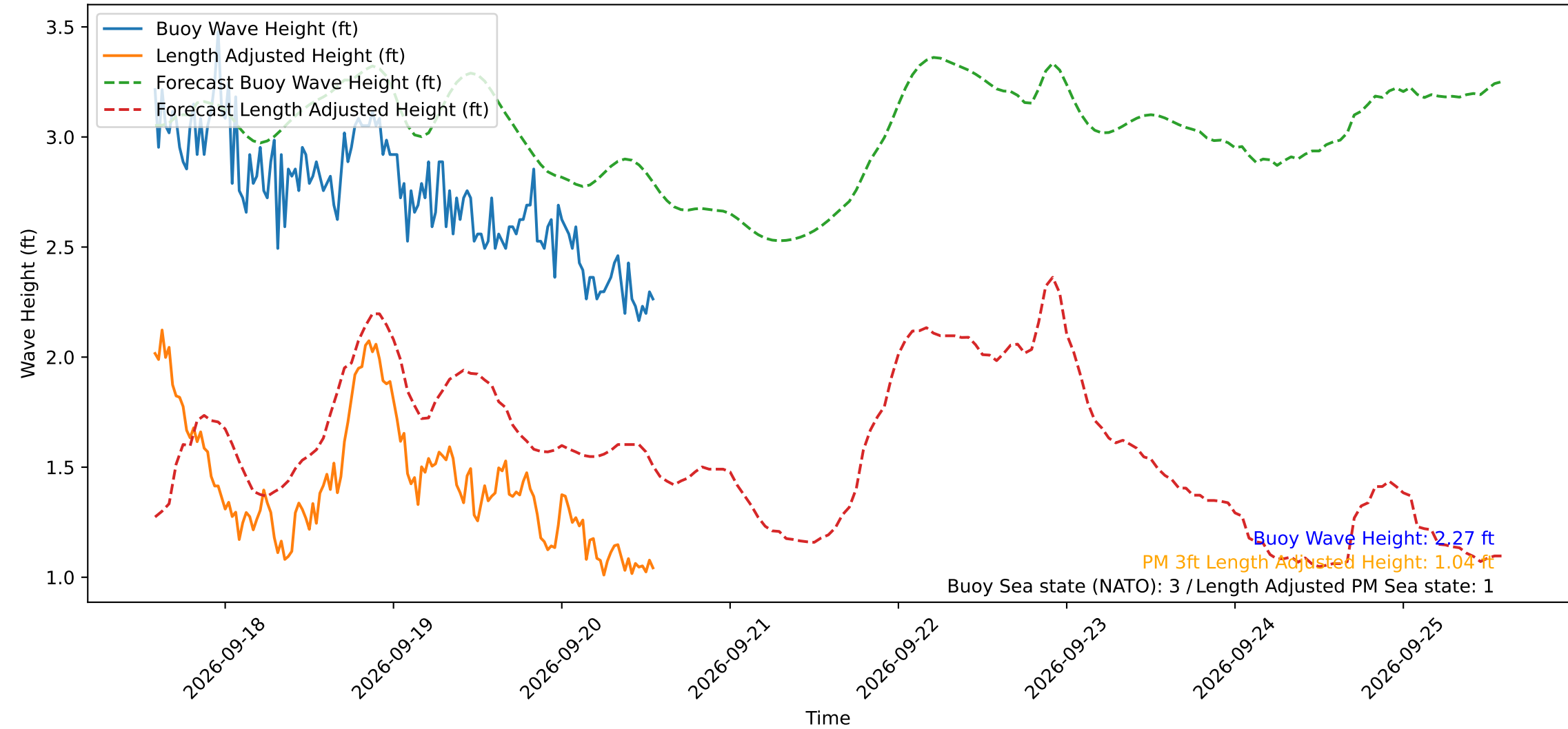
Wave Heights over Time for Green Beach at 2026-09-20 13:51:14
