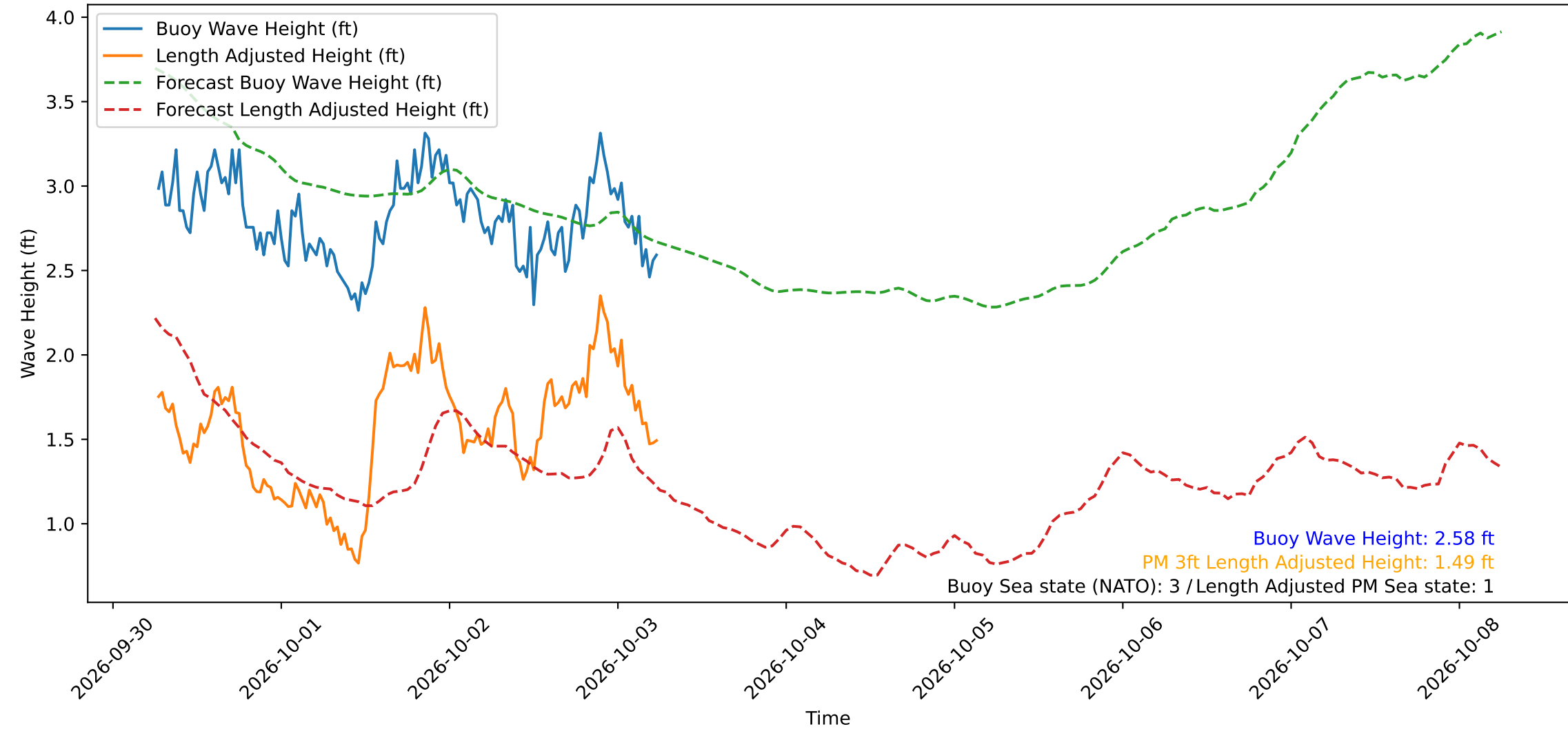
Wave Heights over Time for Oceanside Harbor at 2026-10-03 06:20:30
