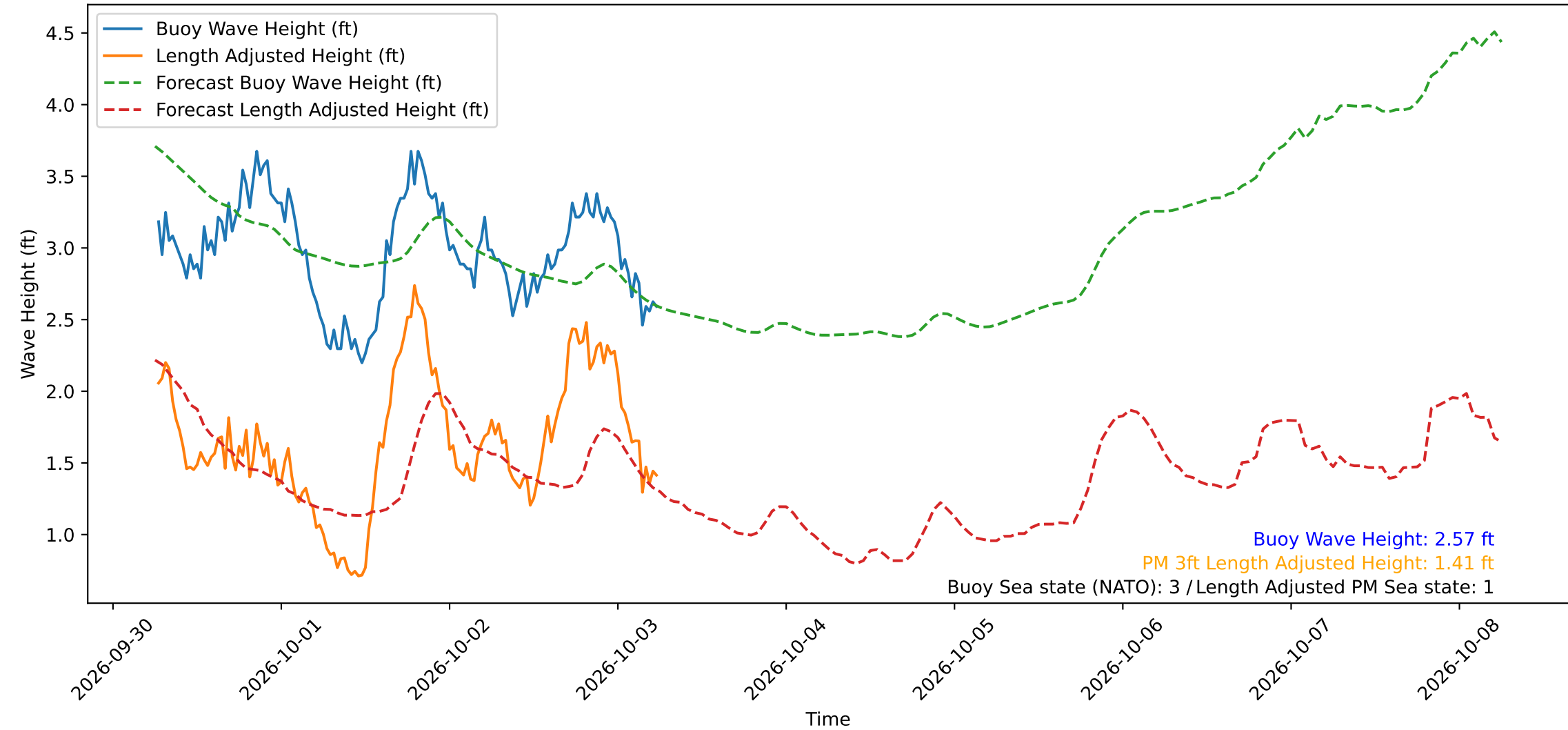
Wave Heights over Time for Green Beach at 2026-10-03 06:21:15
