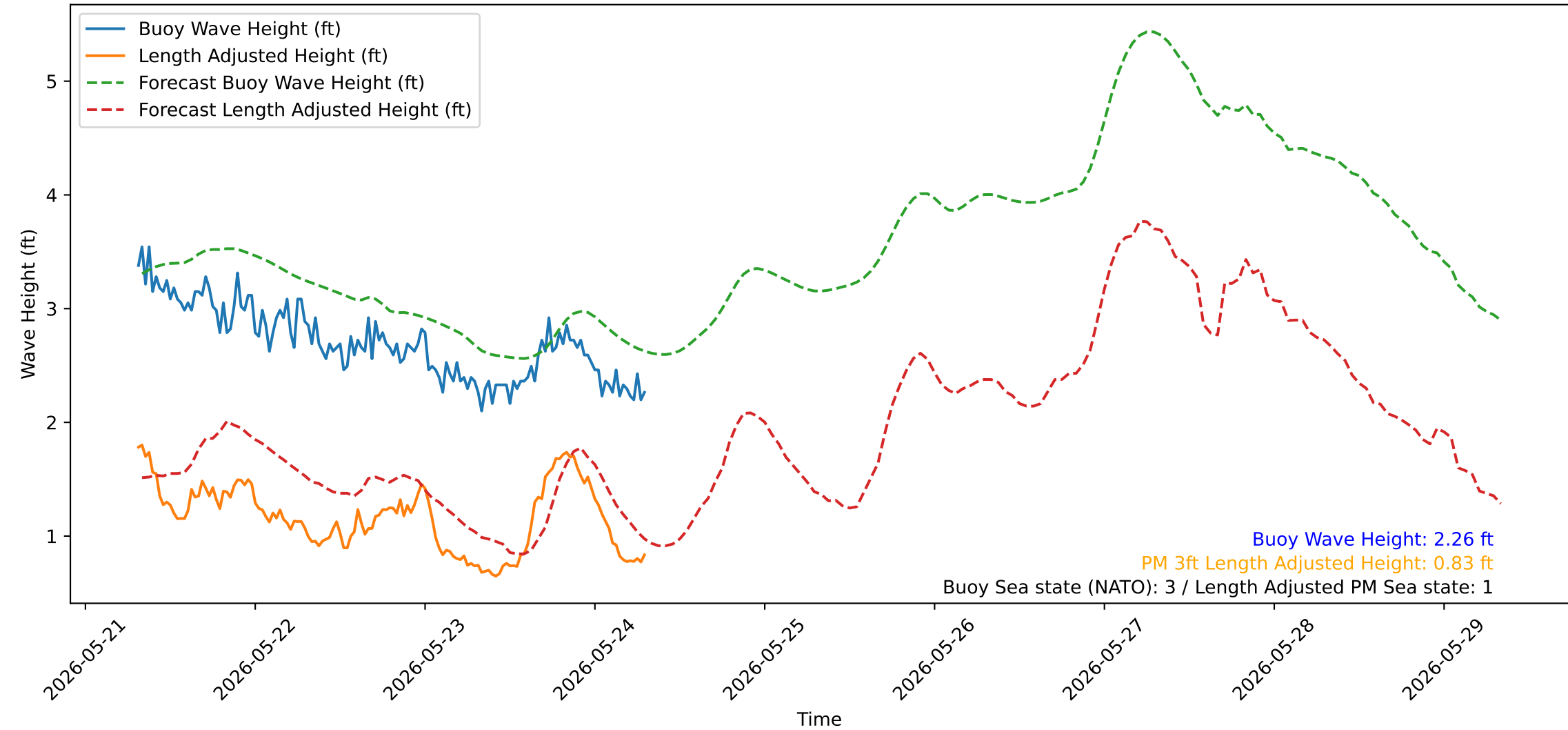
Wave Heights over Time for Green Beach at 2026-05-24 07:41:15
