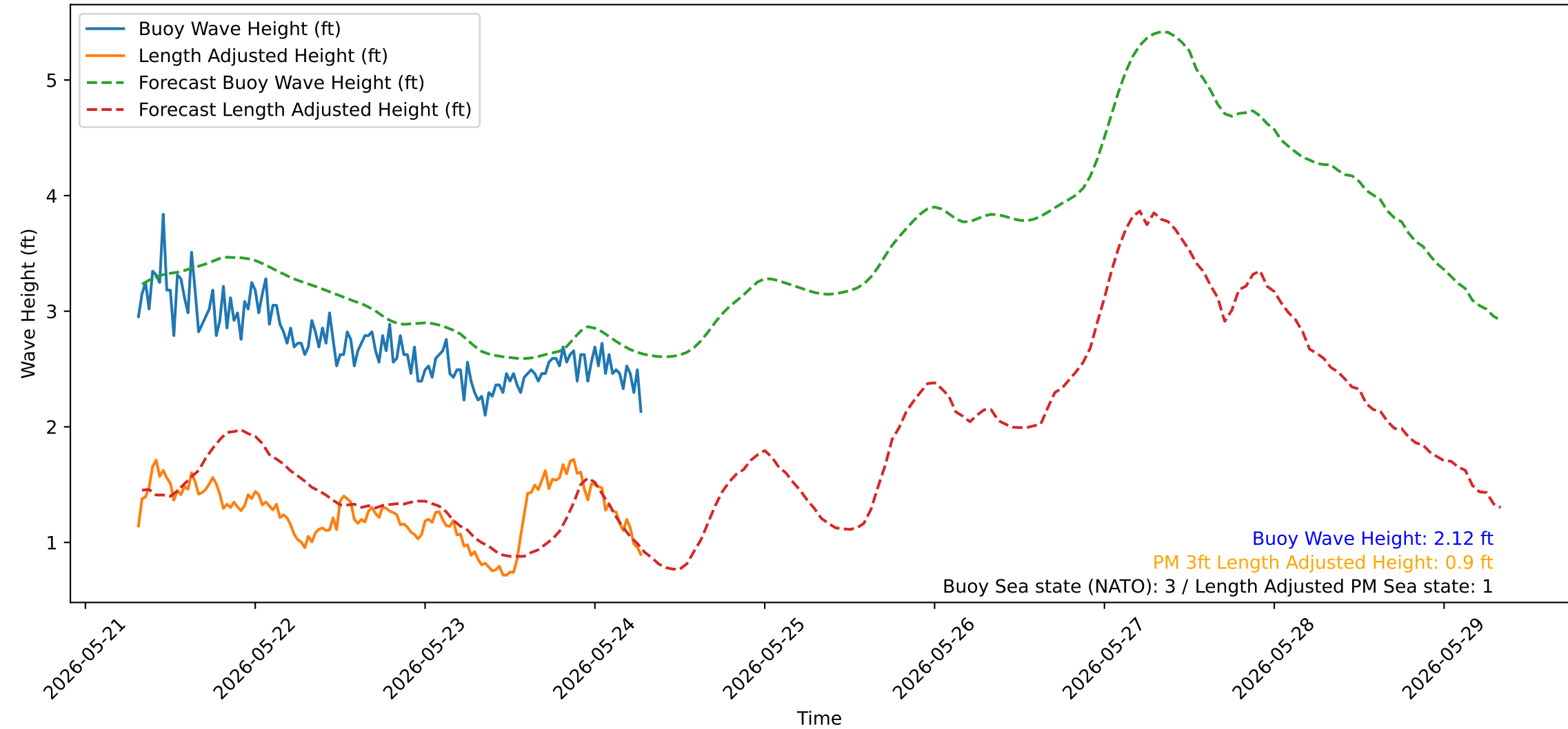
Wave Heights over Time for Oceanside Harbor at 2026-05-24 07:40:32
