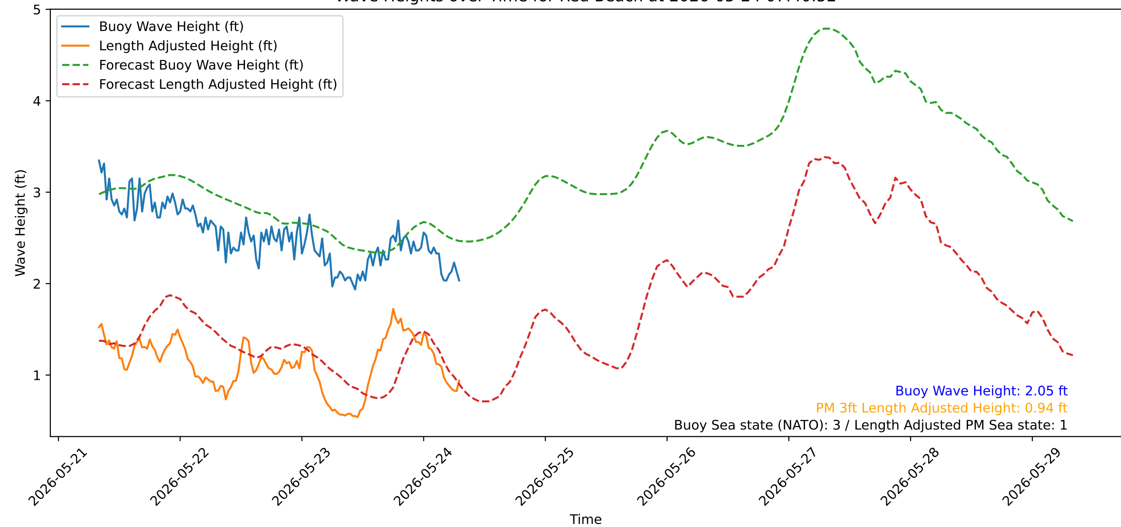
Wave Heights over Time for Red Beach at 2026-05-24 07:40:52
