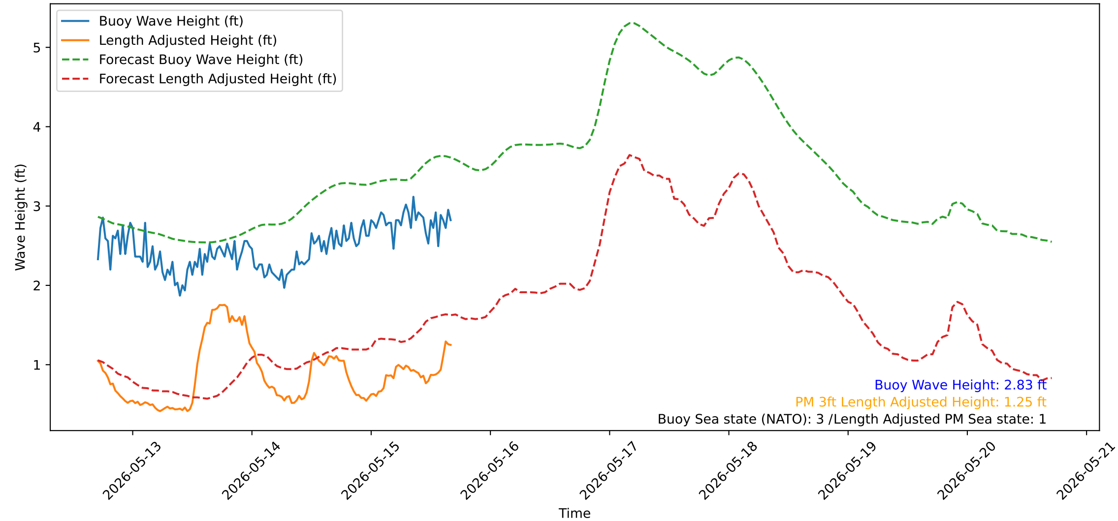
Wave Heights over Time for Red Beach at 2026-05-15 16:40:52
