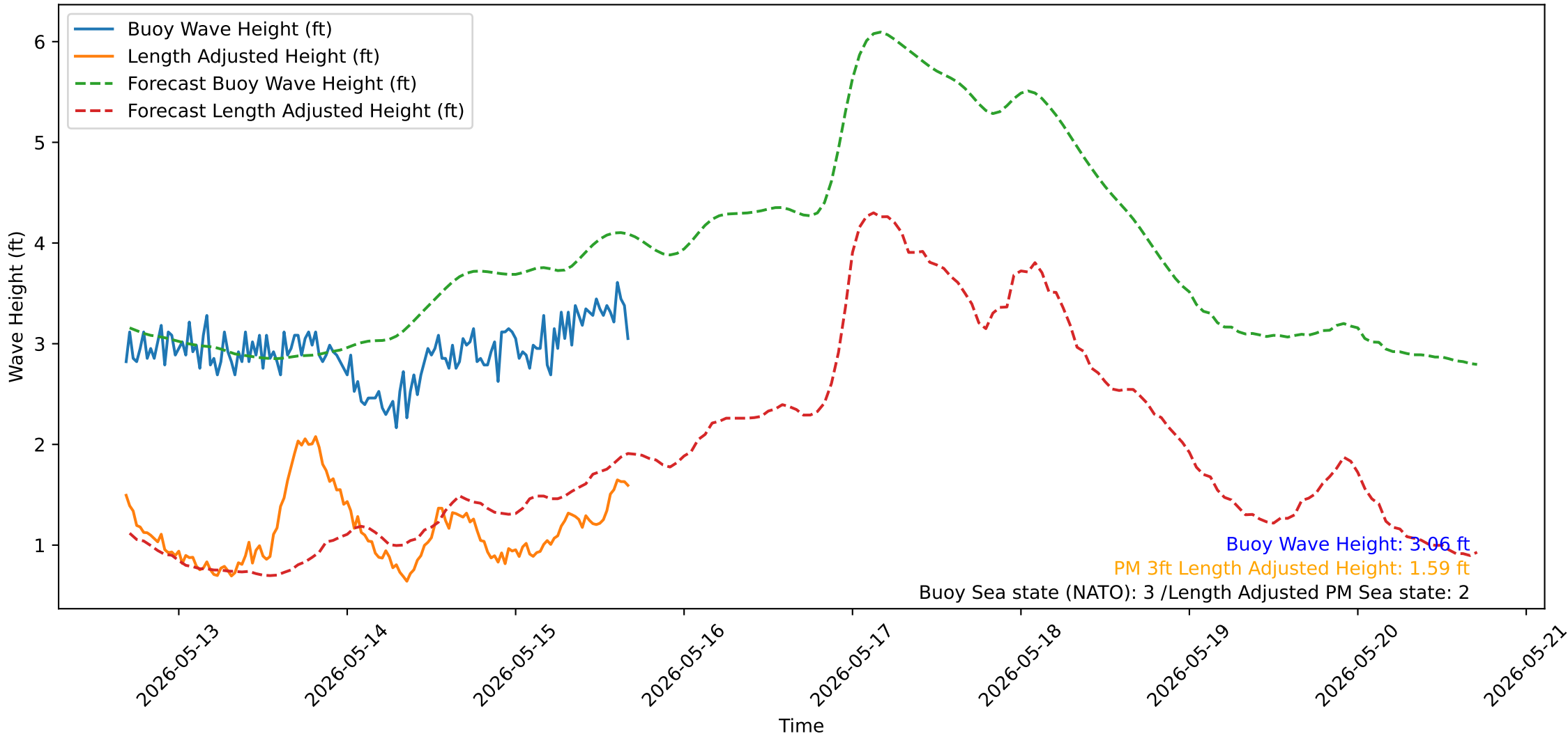
Wave Heights over Time for Oceanside Harbor at 2026-05-15 16:40:32
