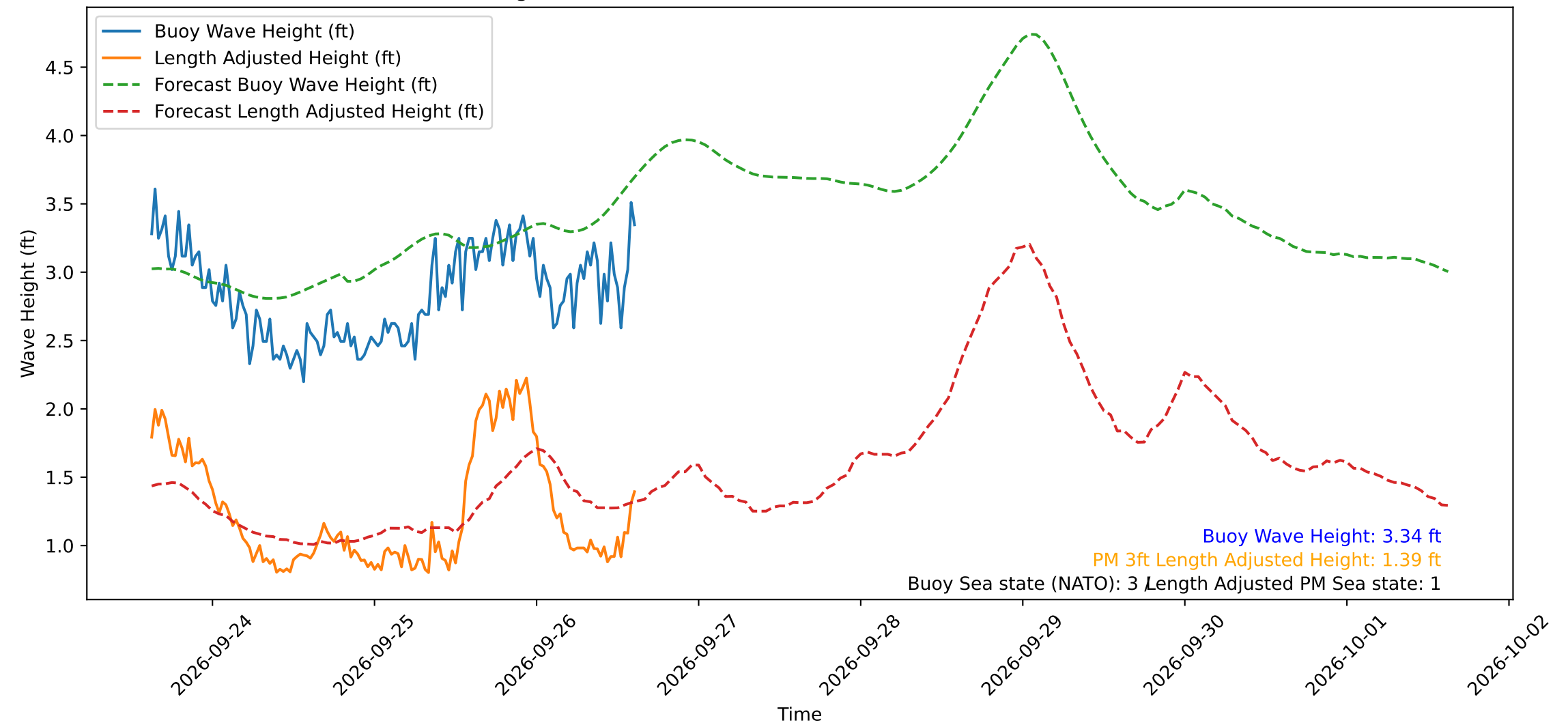
Wave Heights over Time for Oceanside Harbor at 2026-09-26 15:10:30
