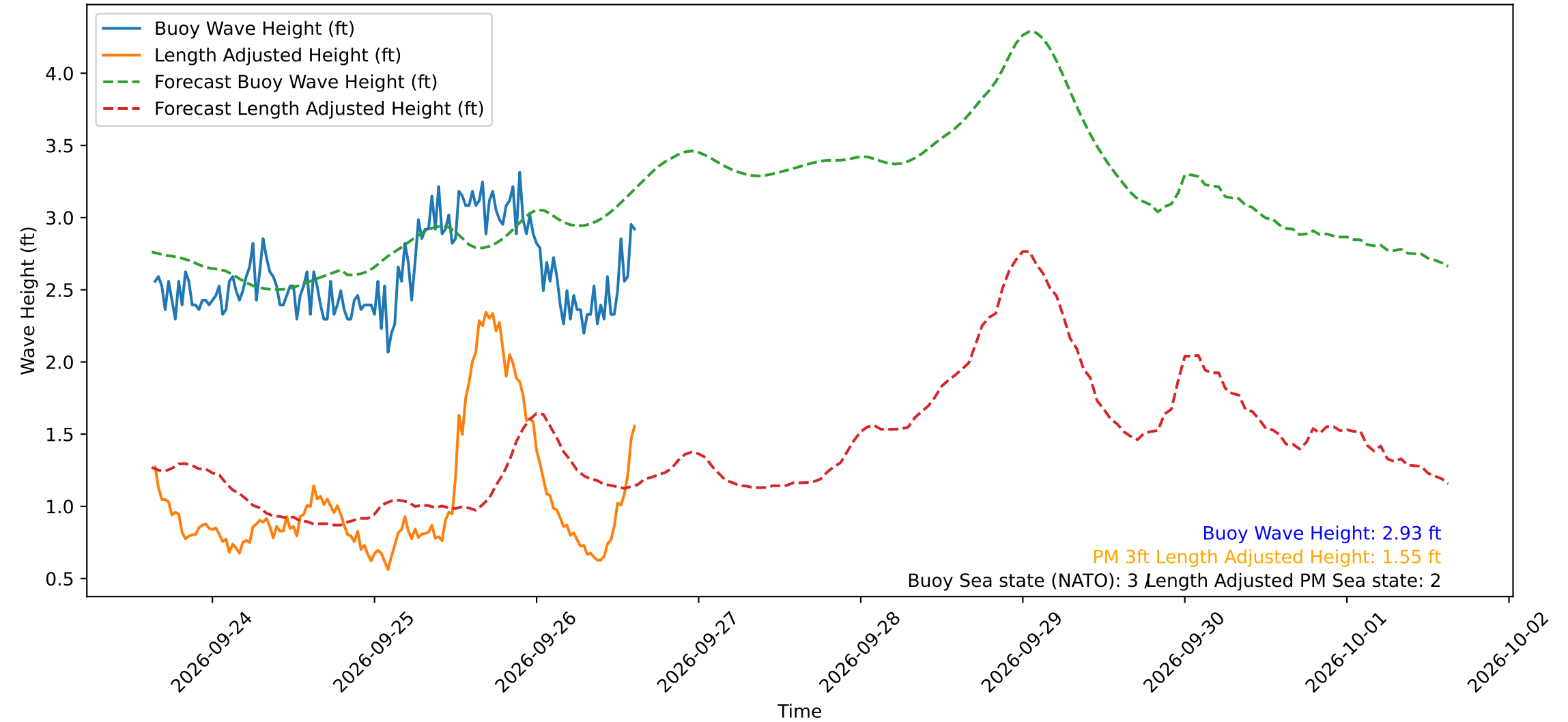
Wave Heights over Time for Red Beach at 2026-09-26 15:10:49
