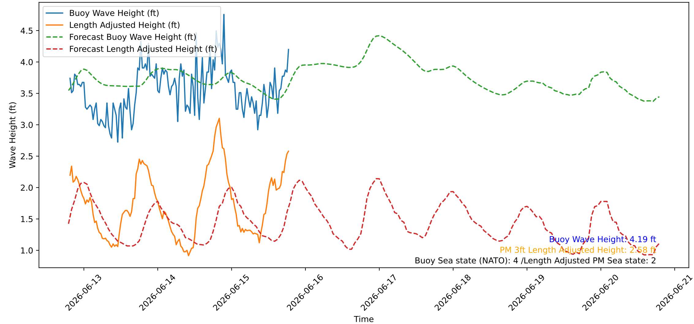
Wave Heights over Time for Red Beach at 2026-06-15 19:10:45
