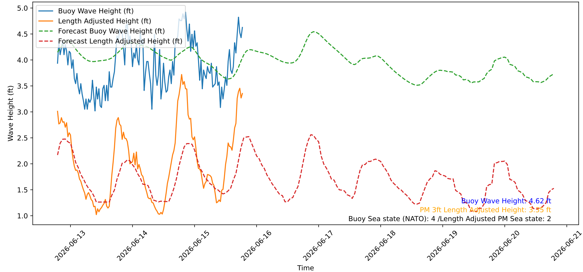
Wave Heights over Time for Green Beach at 2026-06-15 19:11:08
