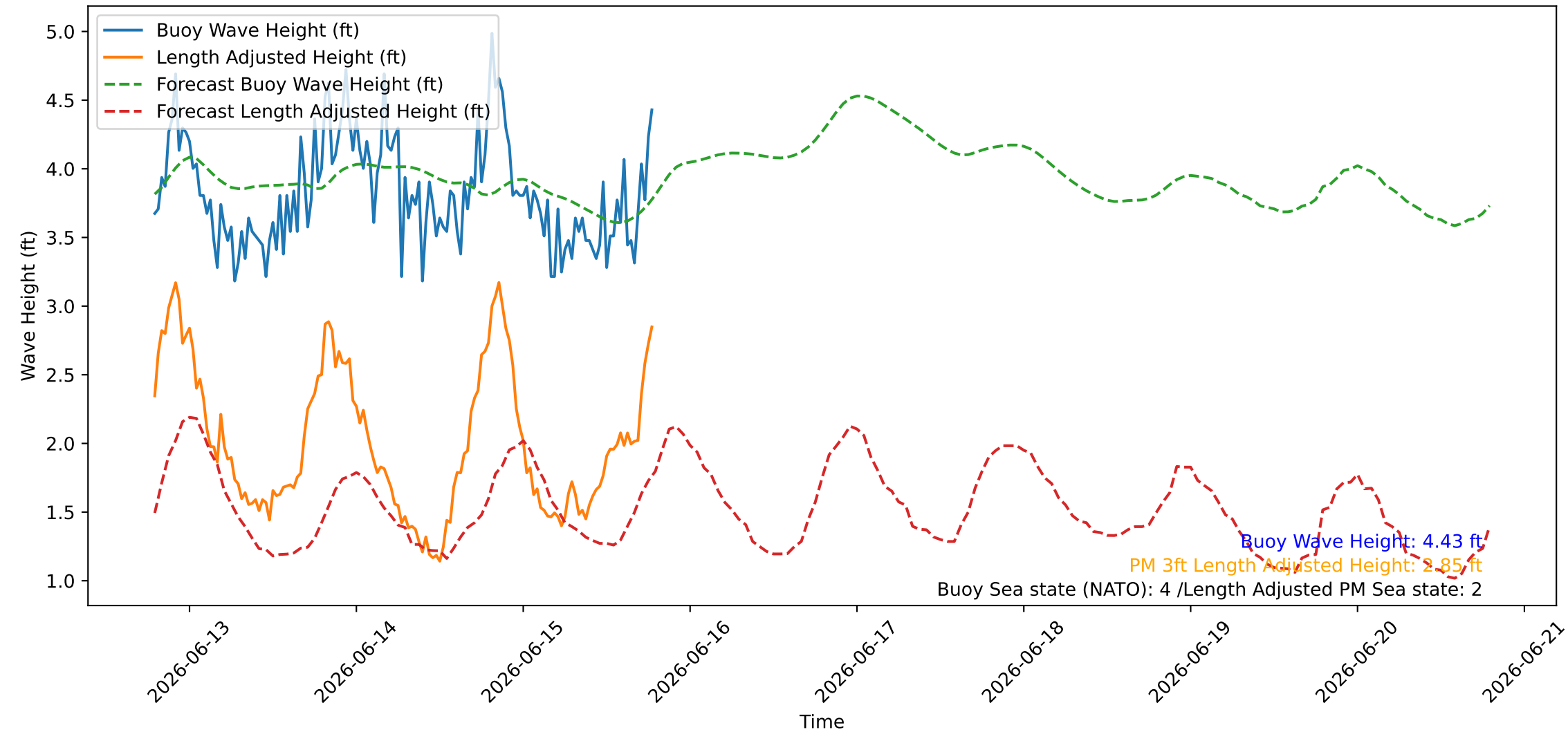
Wave Heights over Time for Oceanside Harbor at 2026-06-15 19:10:26
