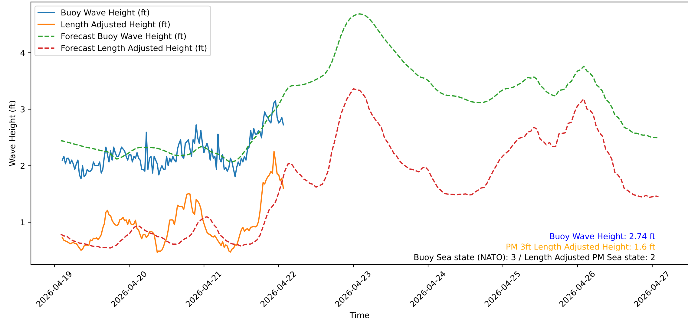
Wave Heights over Time for Red Beach at 2026-04-22 02:20:51
