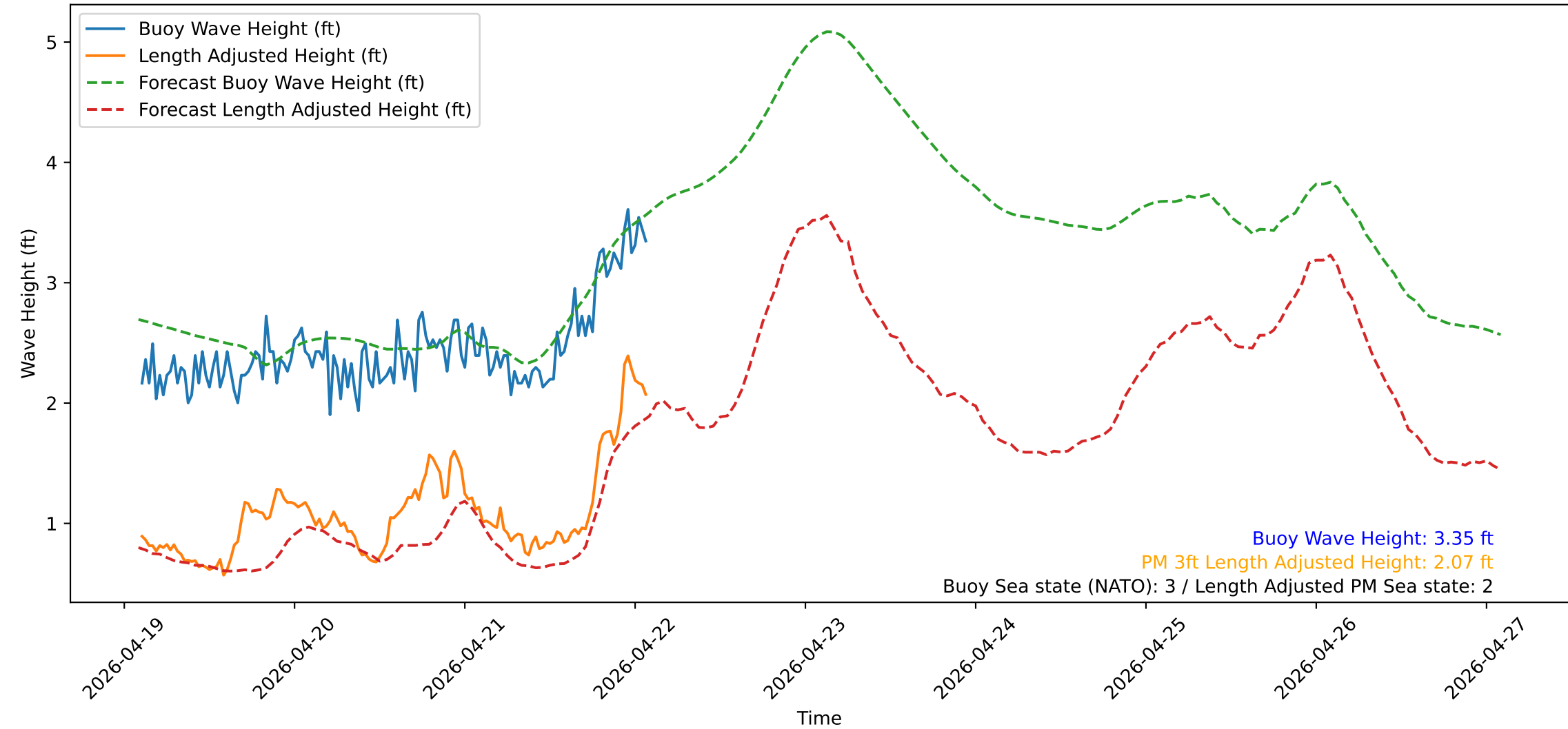
Wave Heights over Time for Oceanside Harbor at 2026-04-22 02:20:30
