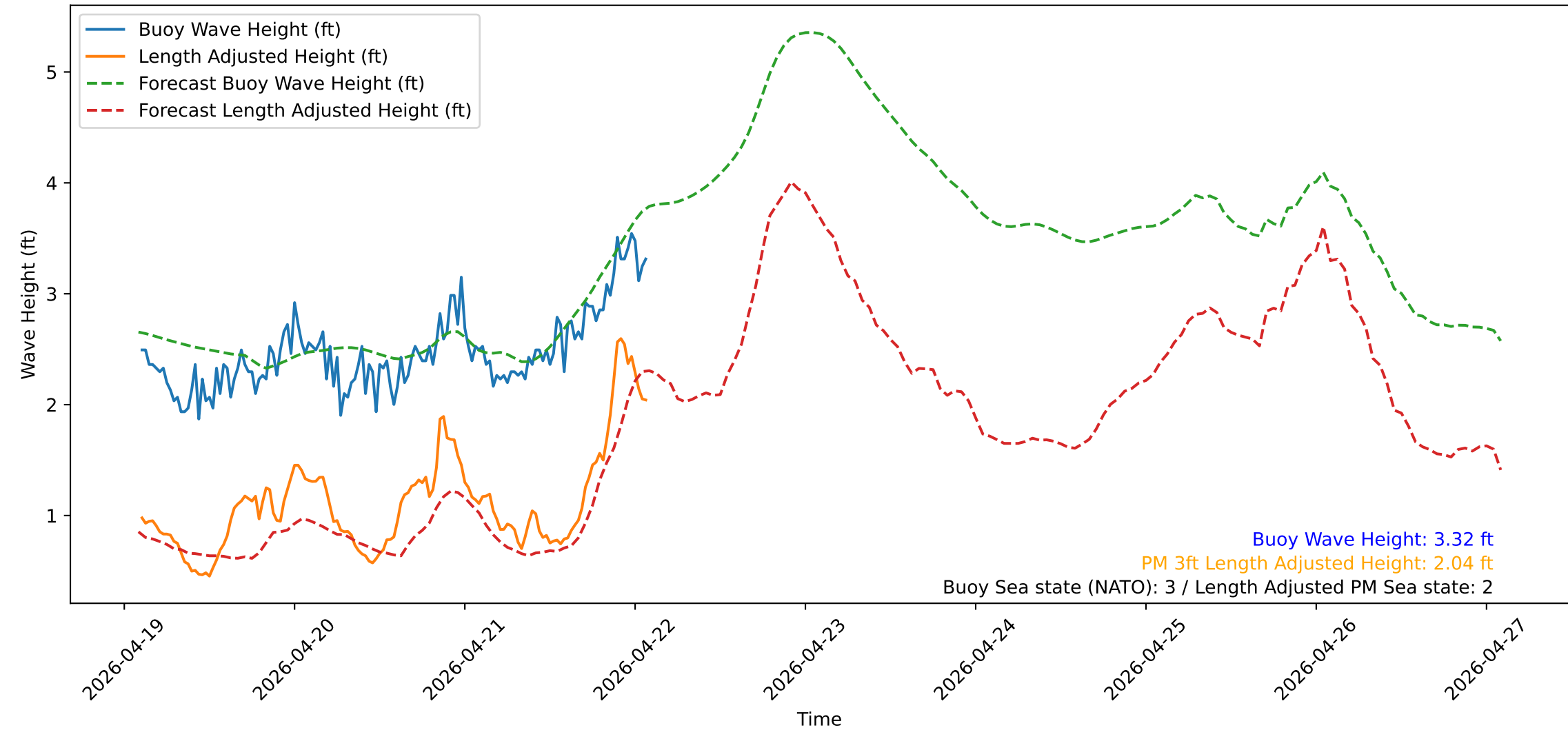
Wave Heights over Time for Green Beach at 2026-04-22 02:21:13
