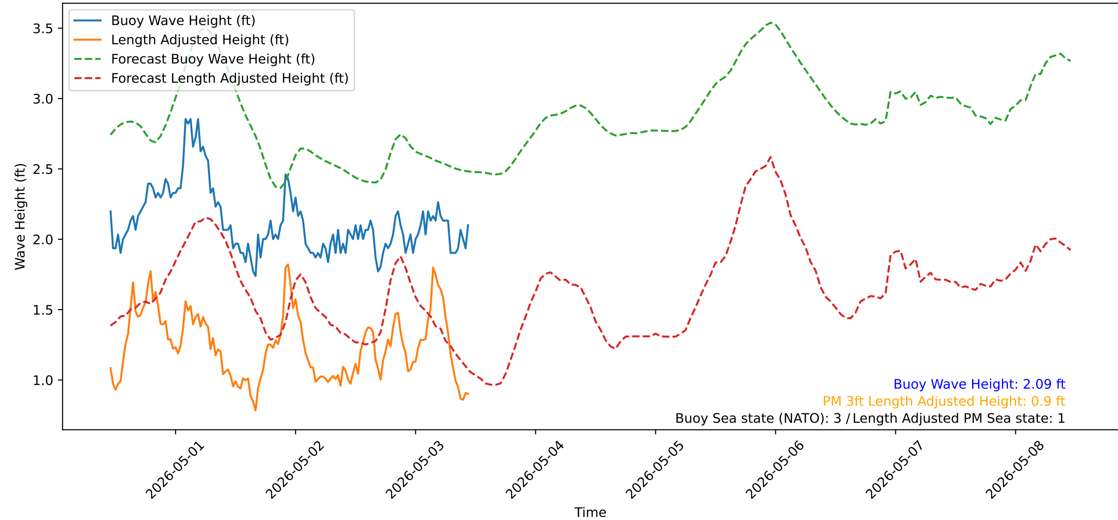
Wave Heights over Time for Green Beach at 2026-05-03 11:11:13
