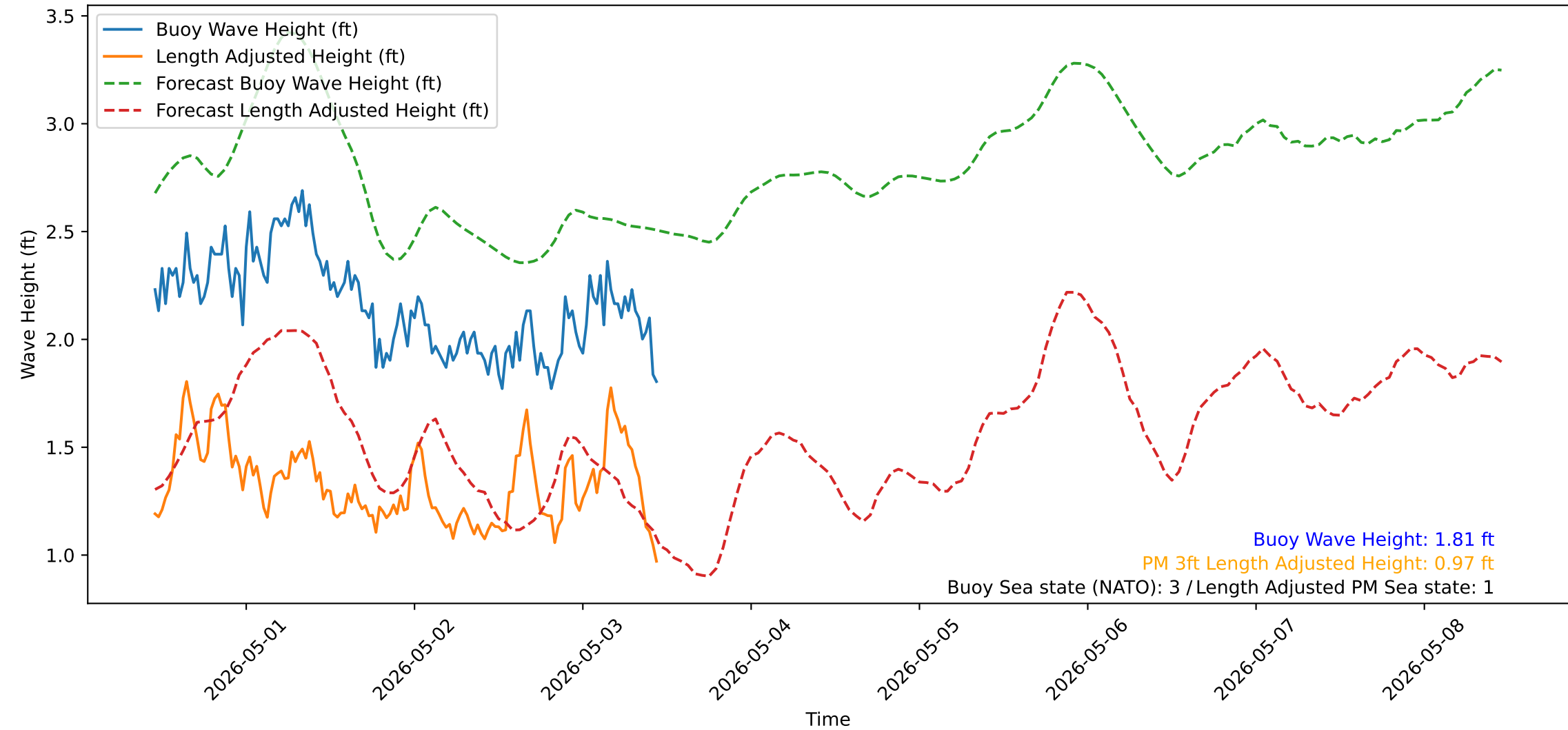
Wave Heights over Time for Oceanside Harbor at 2026-05-03 11:10:31
