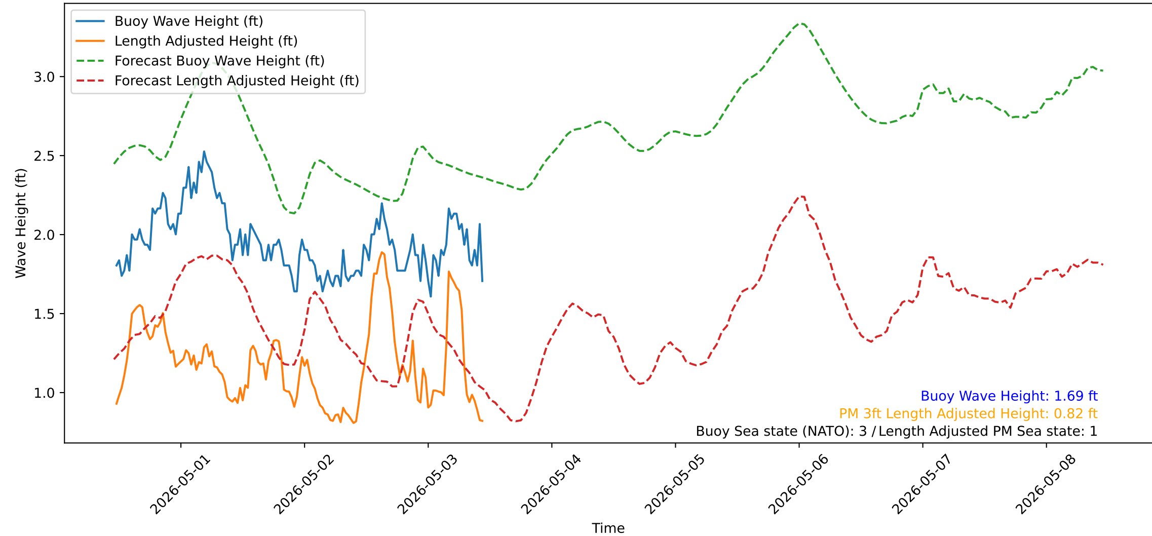
Wave Heights over Time for Red Beach at 2026-05-03 11:10:50
