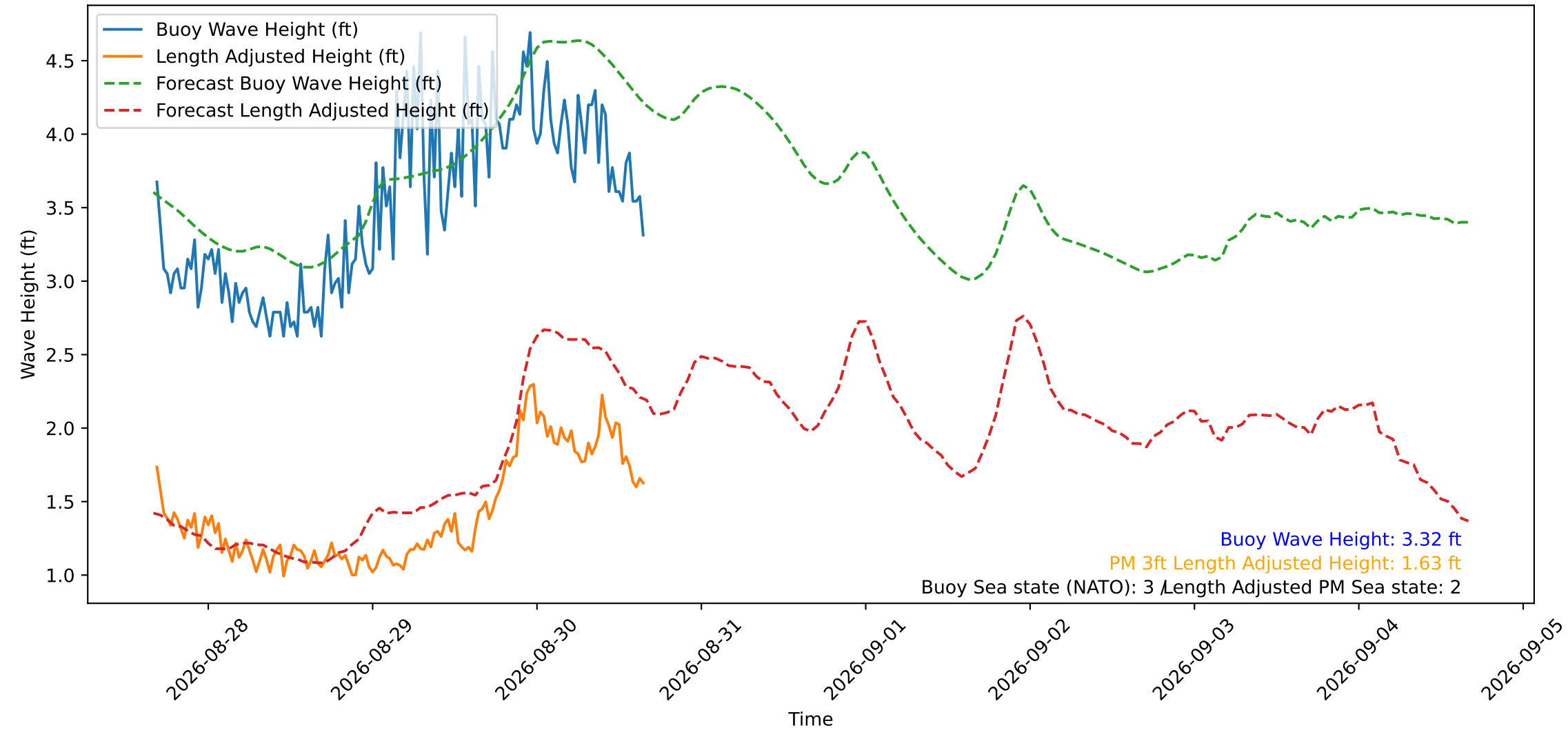
Wave Heights over Time for Red Beach at 2026-08-30 16:20:51
