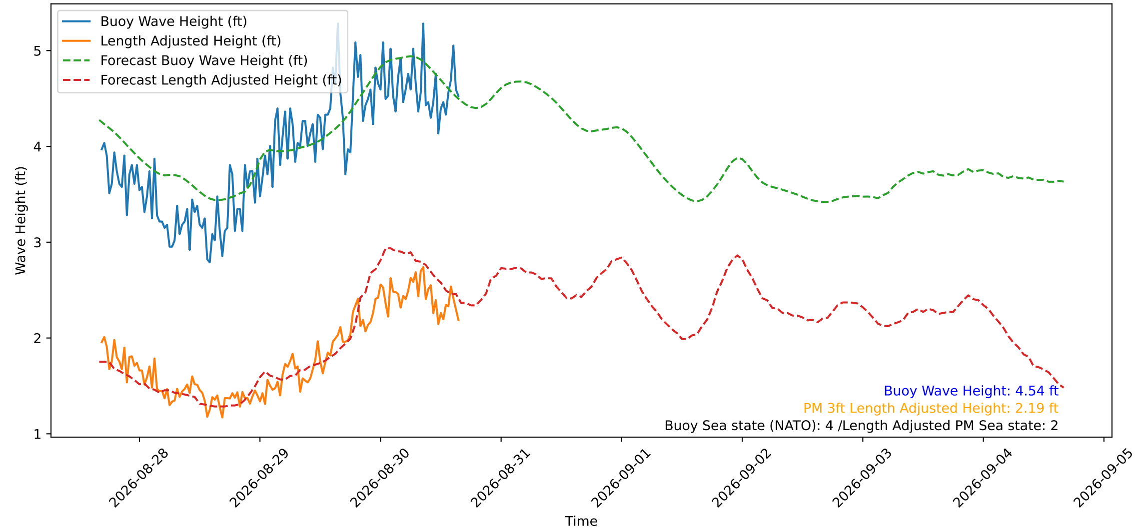
Wave Heights over Time for Oceanside Harbor at 2026-08-30 16:20:29
