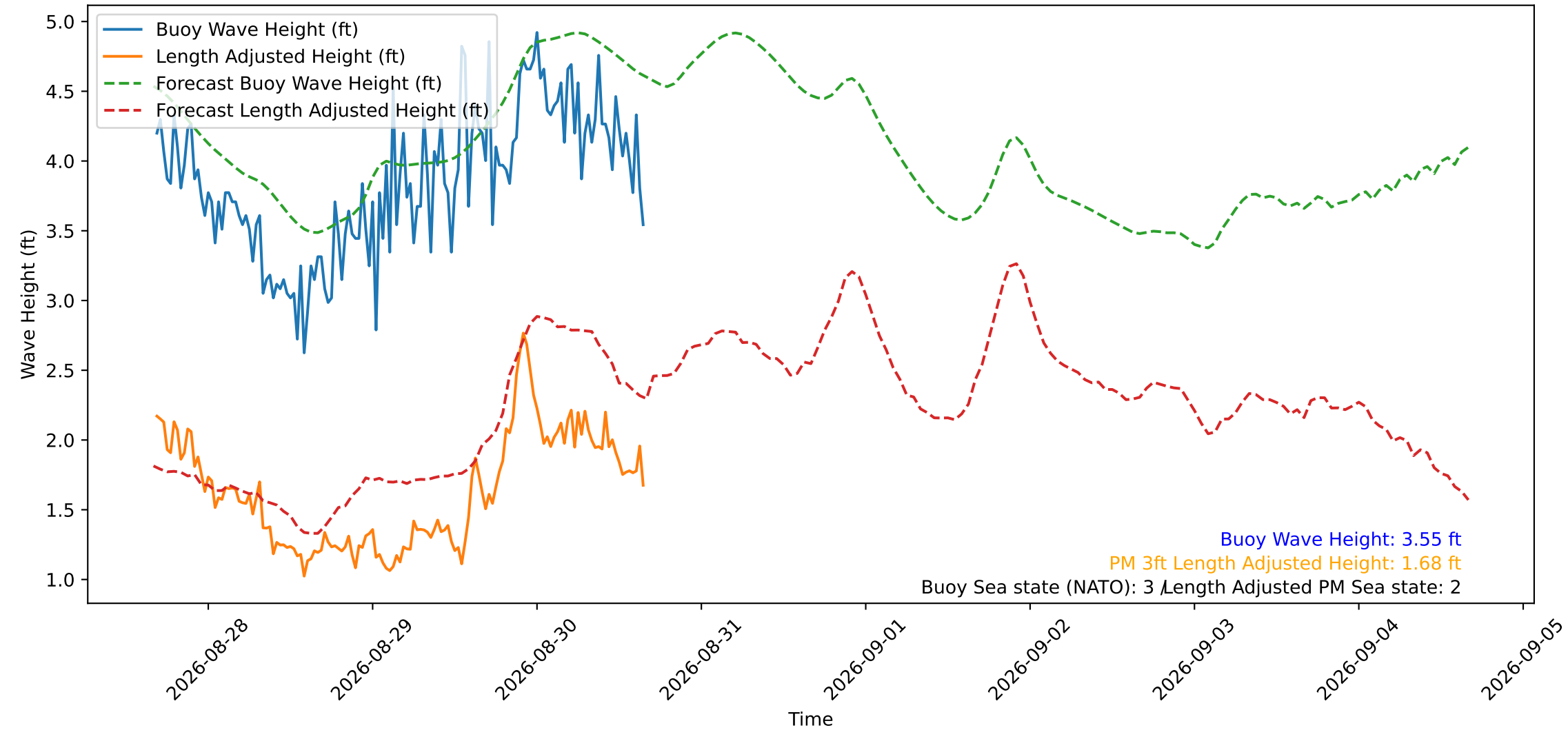
Wave Heights over Time for Green Beach at 2026-08-30 16:21:15
