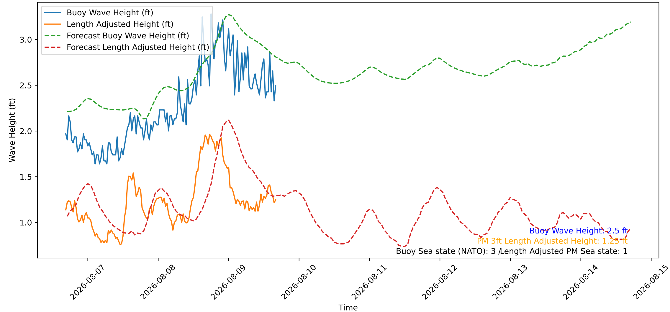
Wave Heights over Time for Oceanside Harbor at 2026-08-09 16:40:27
