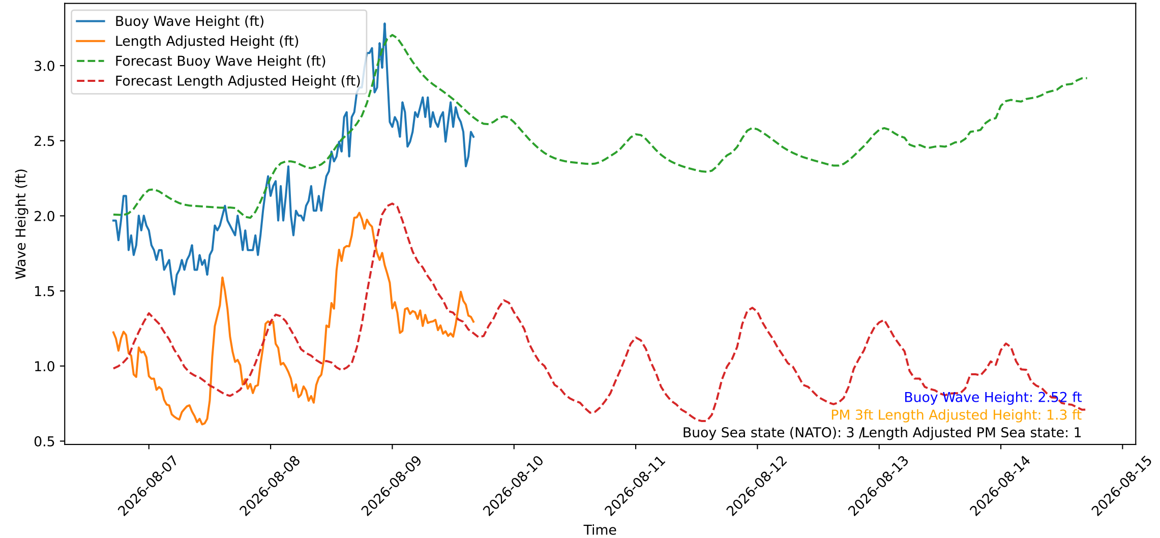
Wave Heights over Time for Red Beach at 2026-08-09 16:40:47
