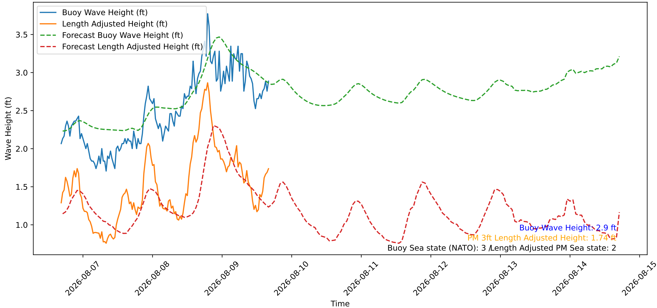
Wave Heights over Time for Green Beach at 2026-08-09 16:41:09
