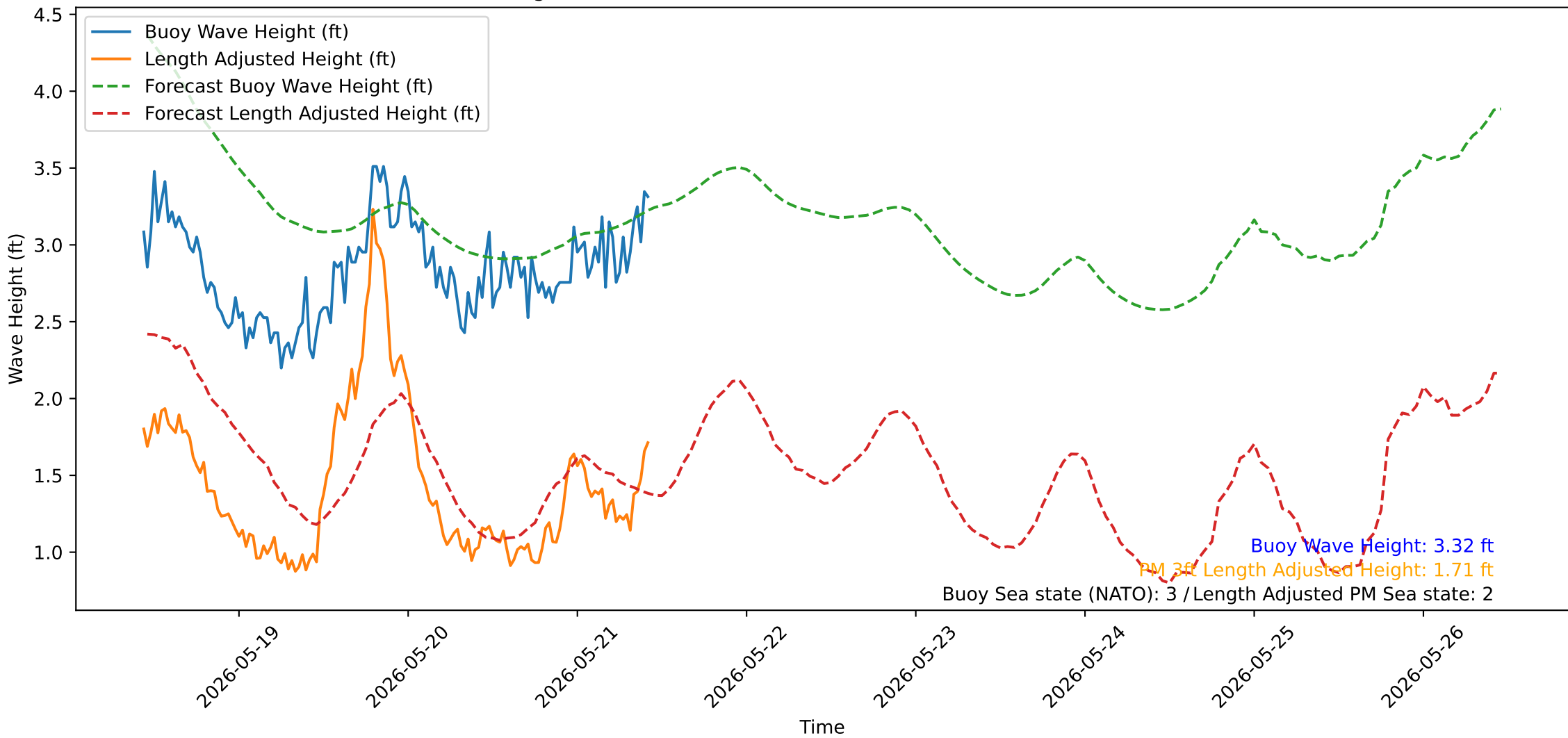
Wave Heights over Time for Oceanside Harbor at 2026-05-21 10:30:31
