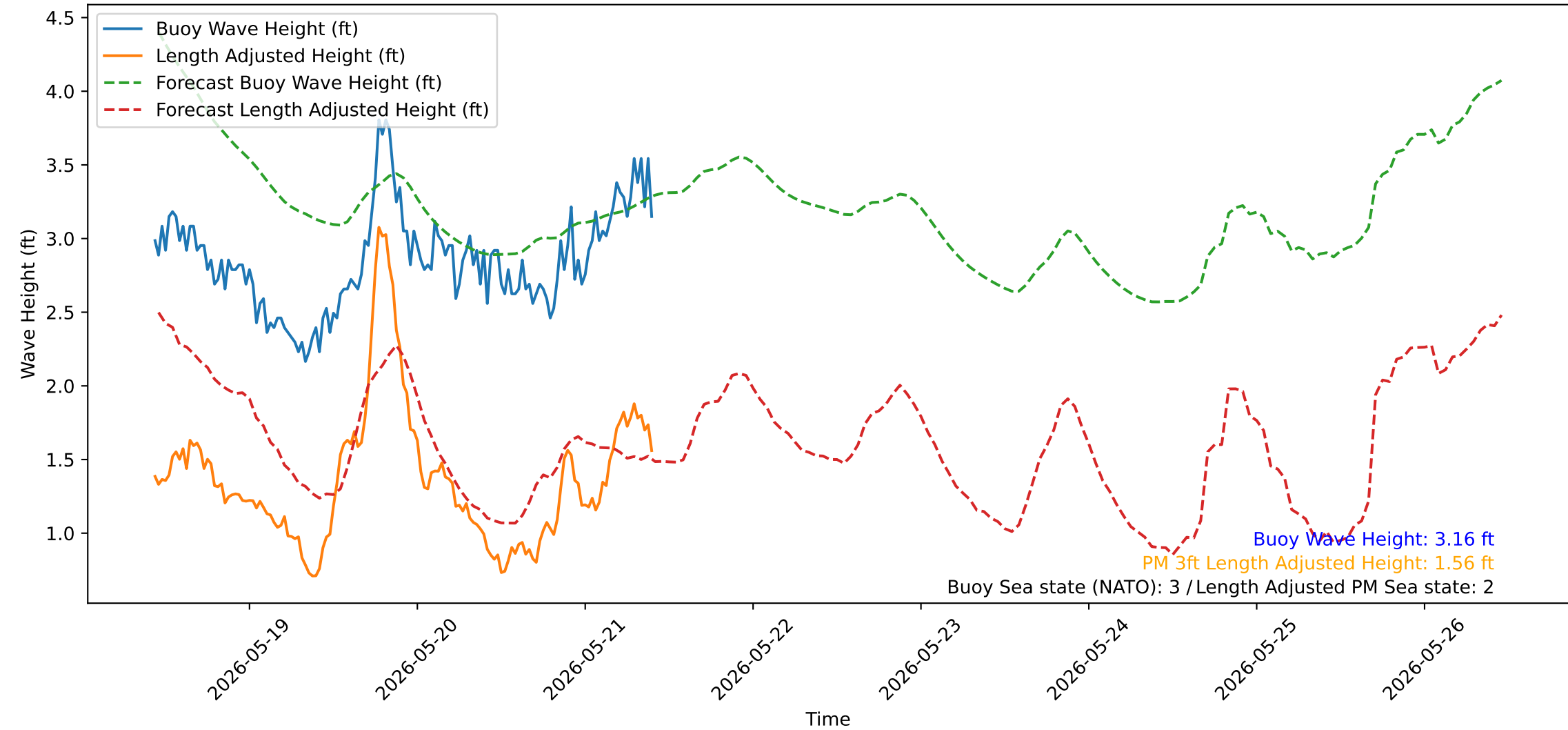
Wave Heights over Time for Green Beach at 2026-05-21 10:31:14
