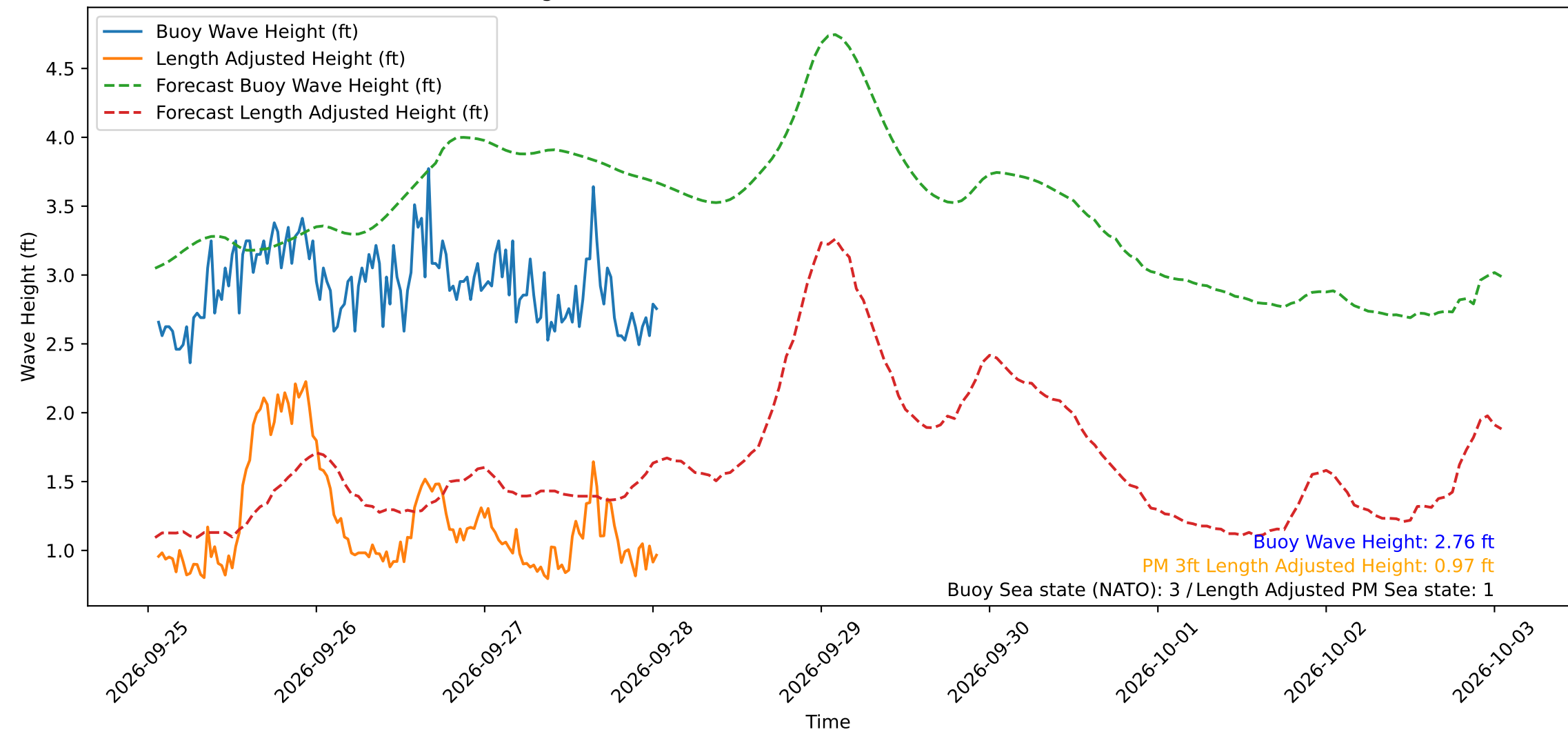
Wave Heights over Time for Oceanside Harbor at 2026-09-28 01:20:30
