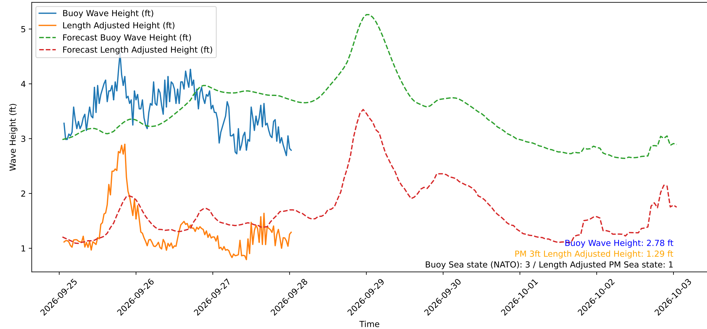
Wave Heights over Time for Green Beach at 2026-09-28 01:21:16
