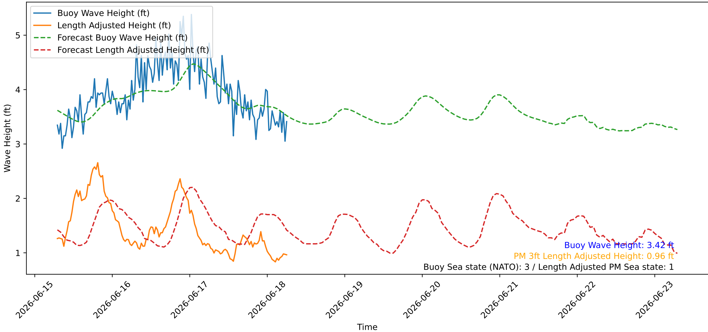
Wave Heights over Time for Red Beach at 2026-06-18 06:50:47
