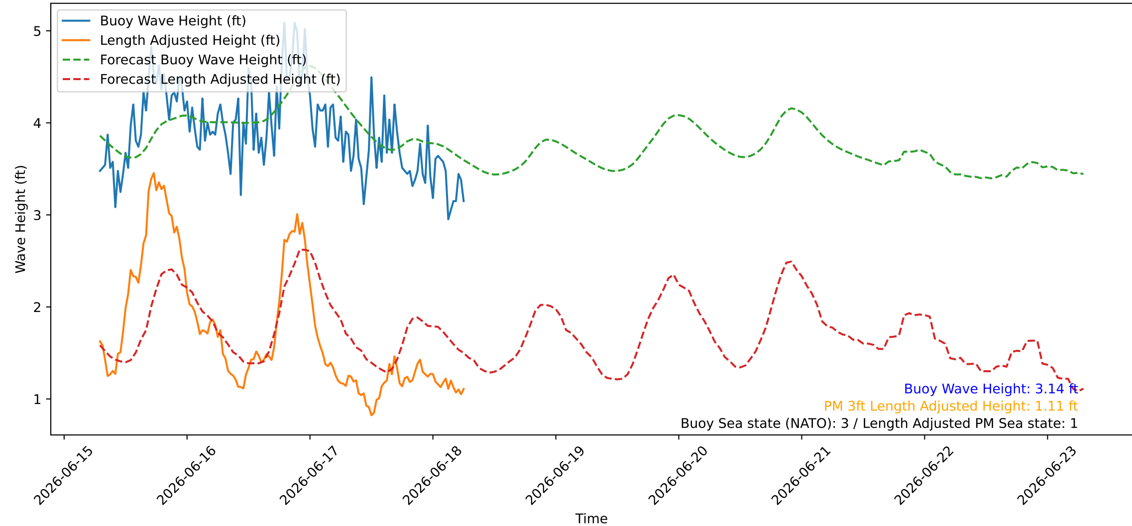
Wave Heights over Time for Green Beach at 2026-06-18 06:51:10
