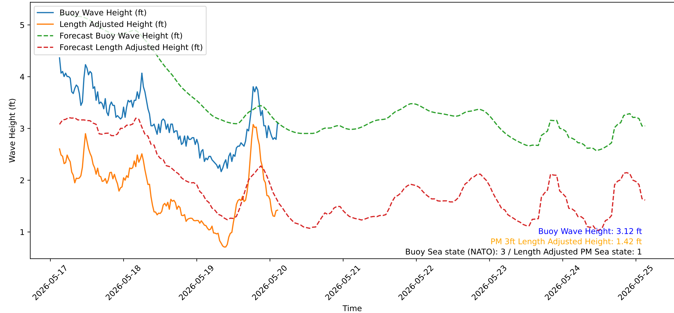
Wave Heights over Time for Green Beach at 2026-05-20 03:11:13
