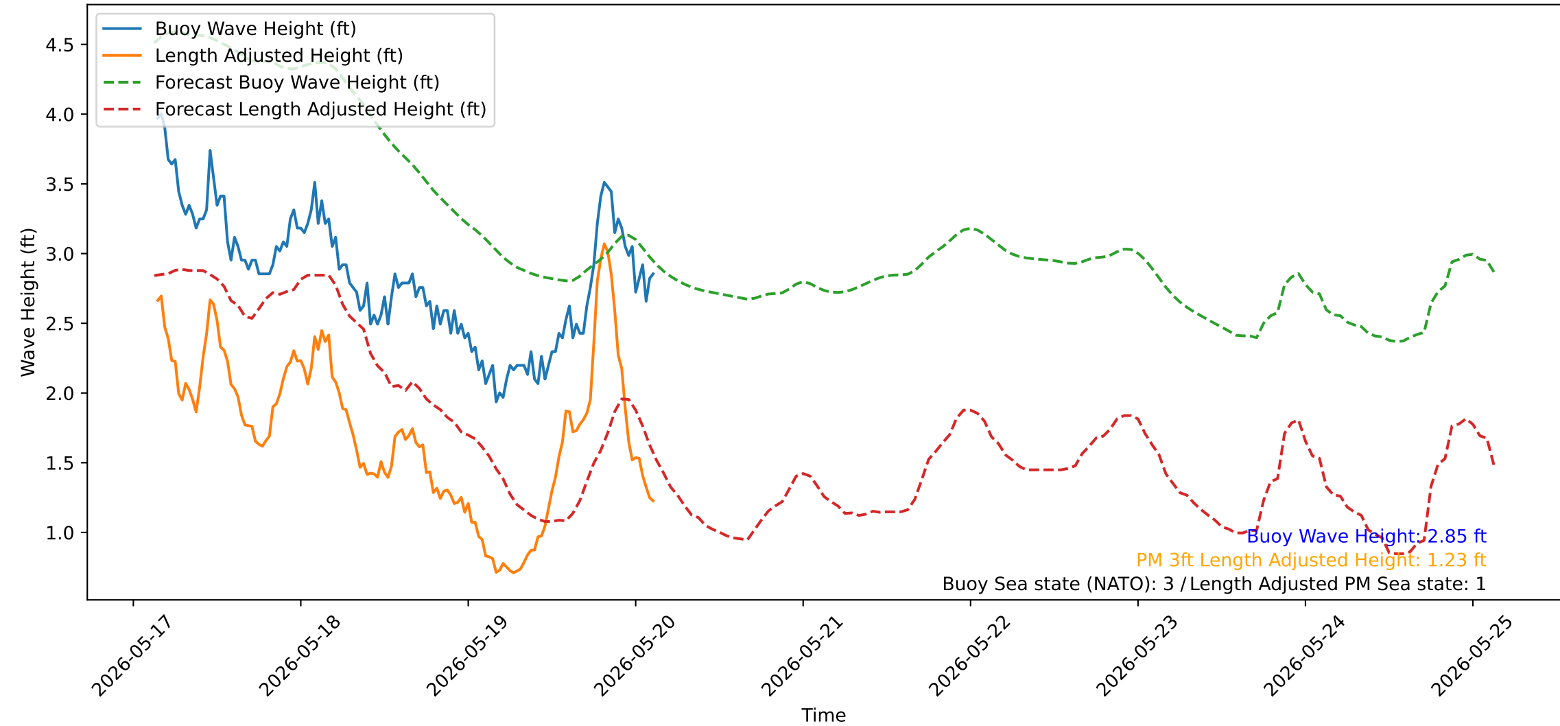
Wave Heights over Time for Red Beach at 2026-05-20 03:10:51
