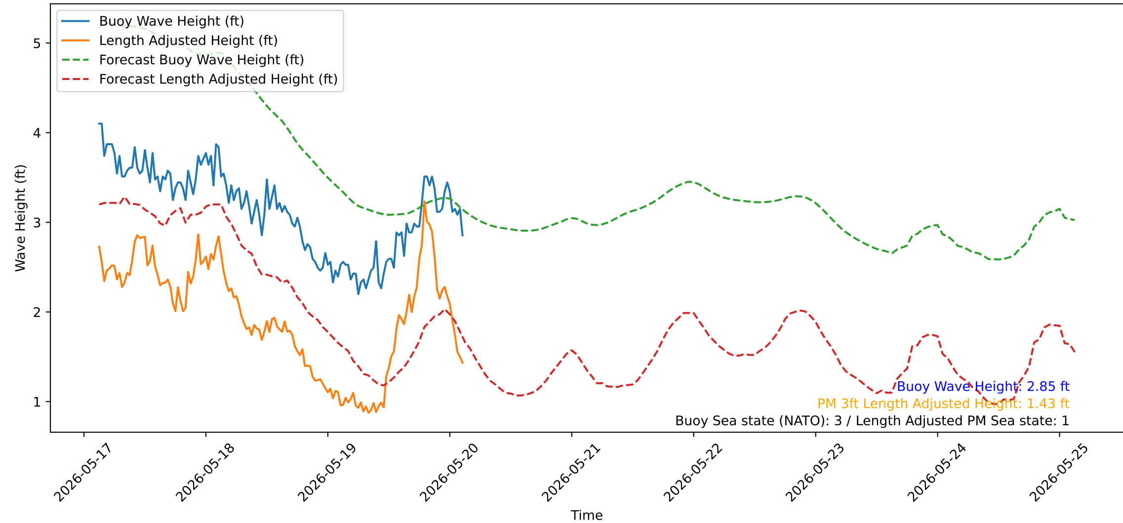
Wave Heights over Time for Oceanside Harbor at 2026-05-20 03:10:31
