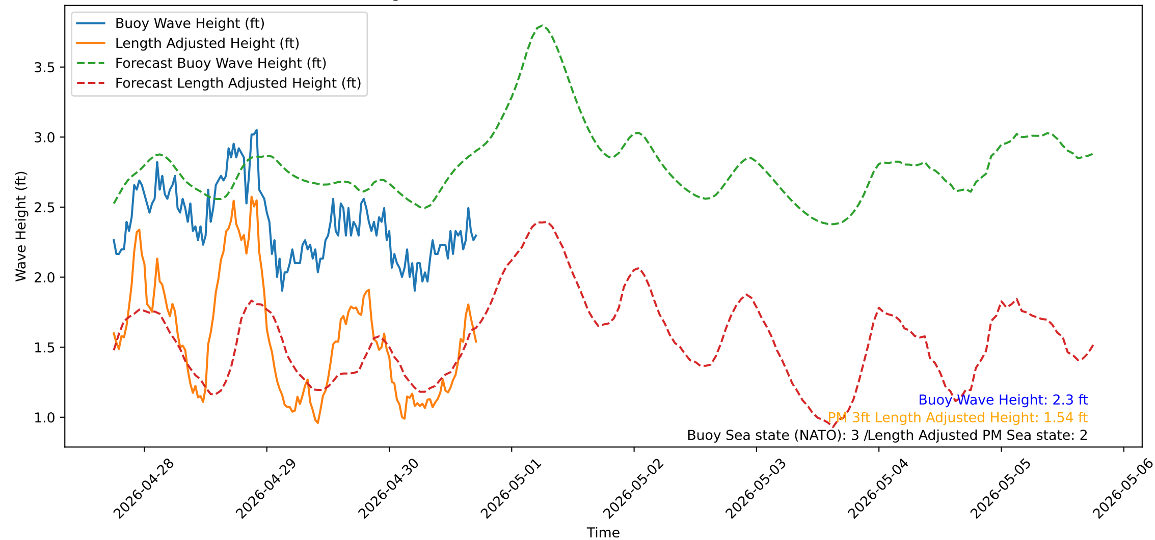
Wave Heights over Time for Oceanside Harbor at 2026-04-30 17:50:31
