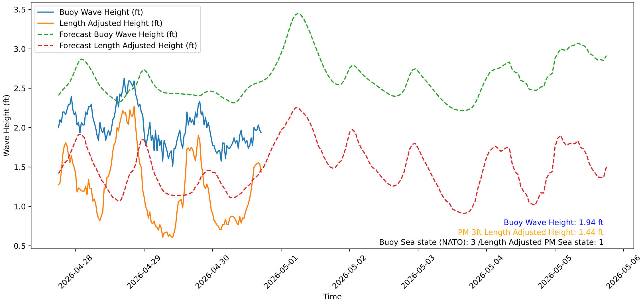
Wave Heights over Time for Red Beach at 2026-04-30 17:50:52
