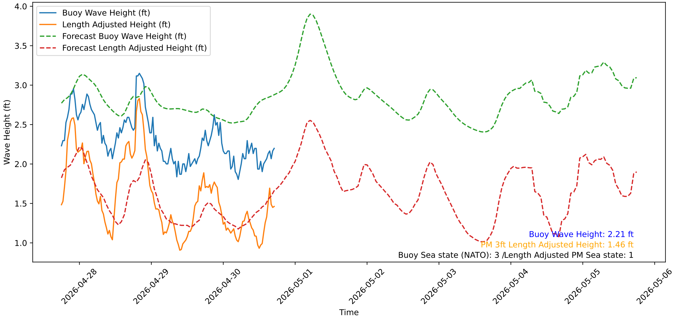
Wave Heights over Time for Green Beach at 2026-04-30 17:51:14
