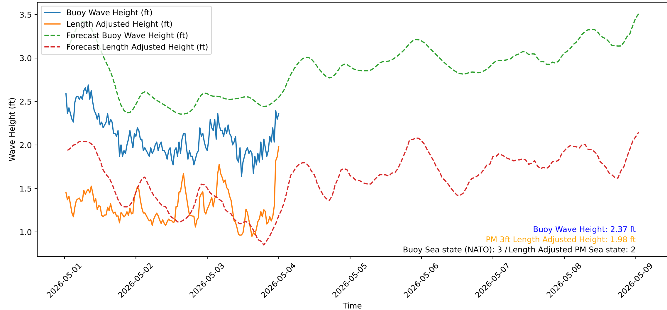
Wave Heights over Time for Oceanside Harbor at 2026-05-04 00:40:32
