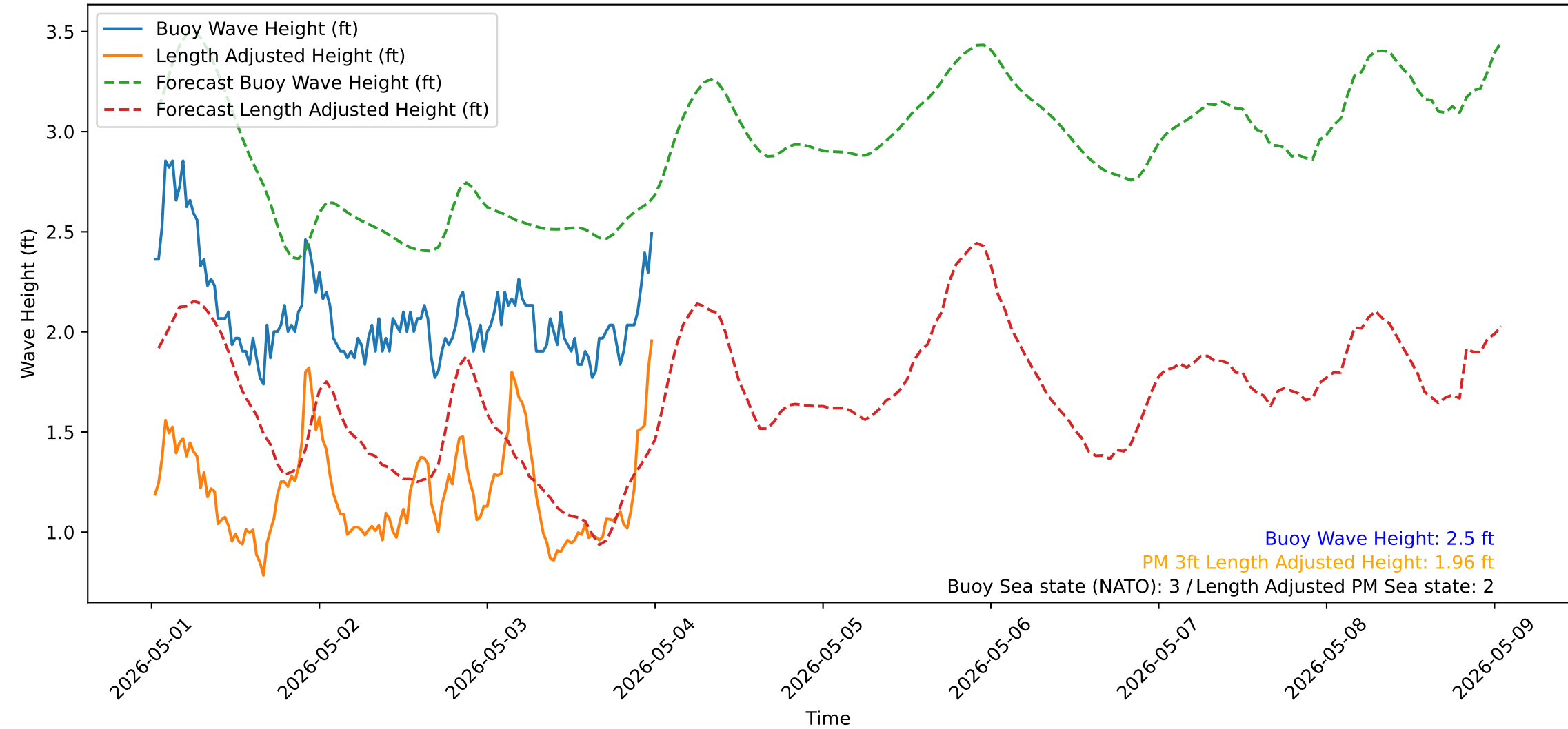
Wave Heights over Time for Green Beach at 2026-05-04 00:41:13
