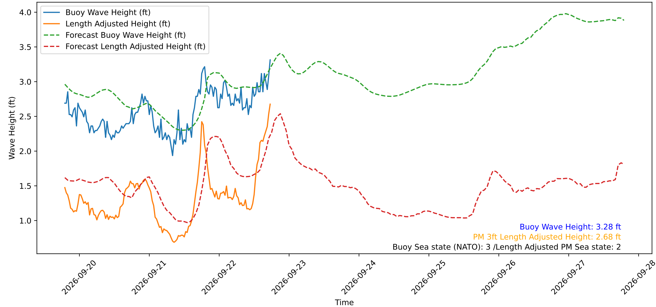
Wave Heights over Time for Green Beach at 2026-09-22 18:51:15
