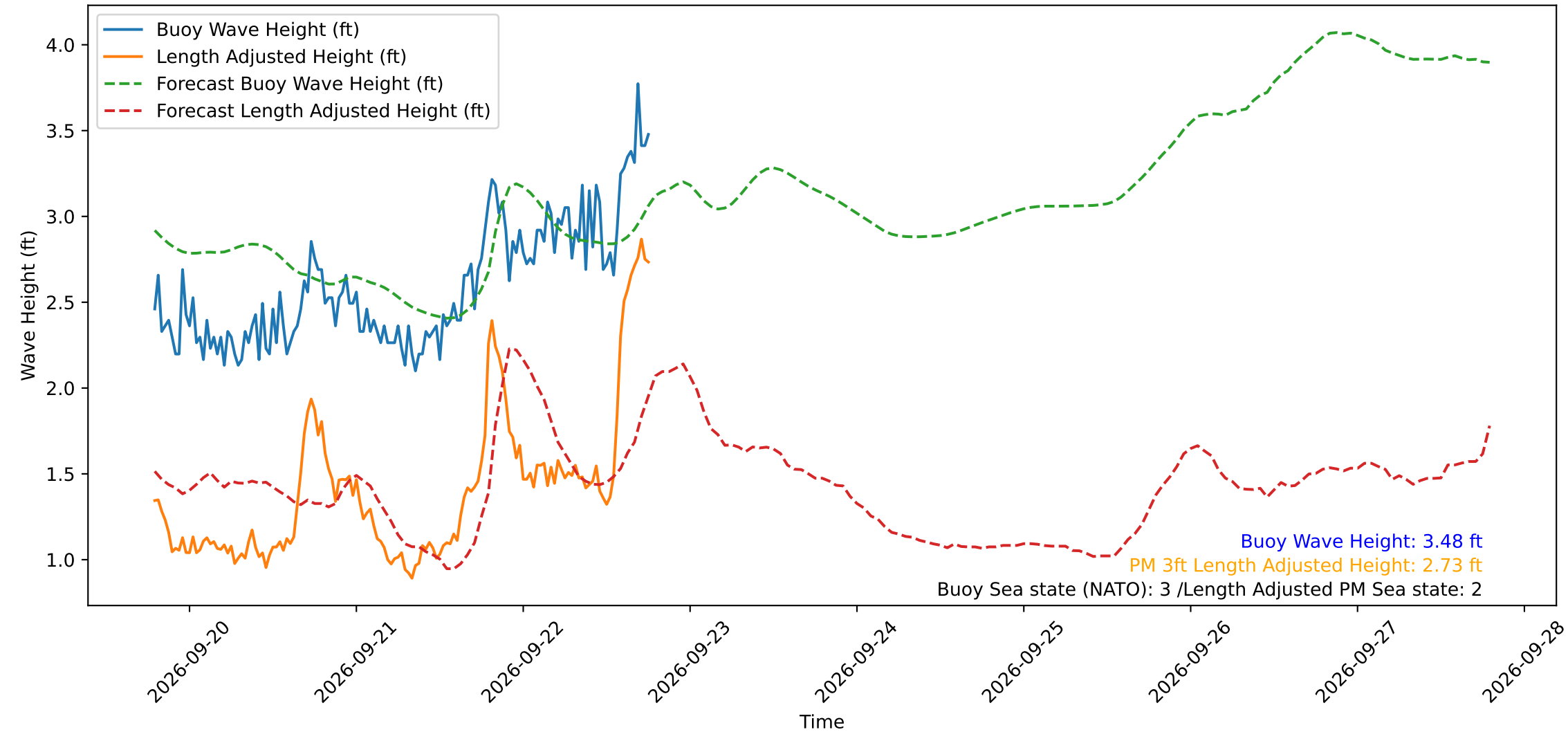
Wave Heights over Time for Oceanside Harbor at 2026-09-22 18:50:30
