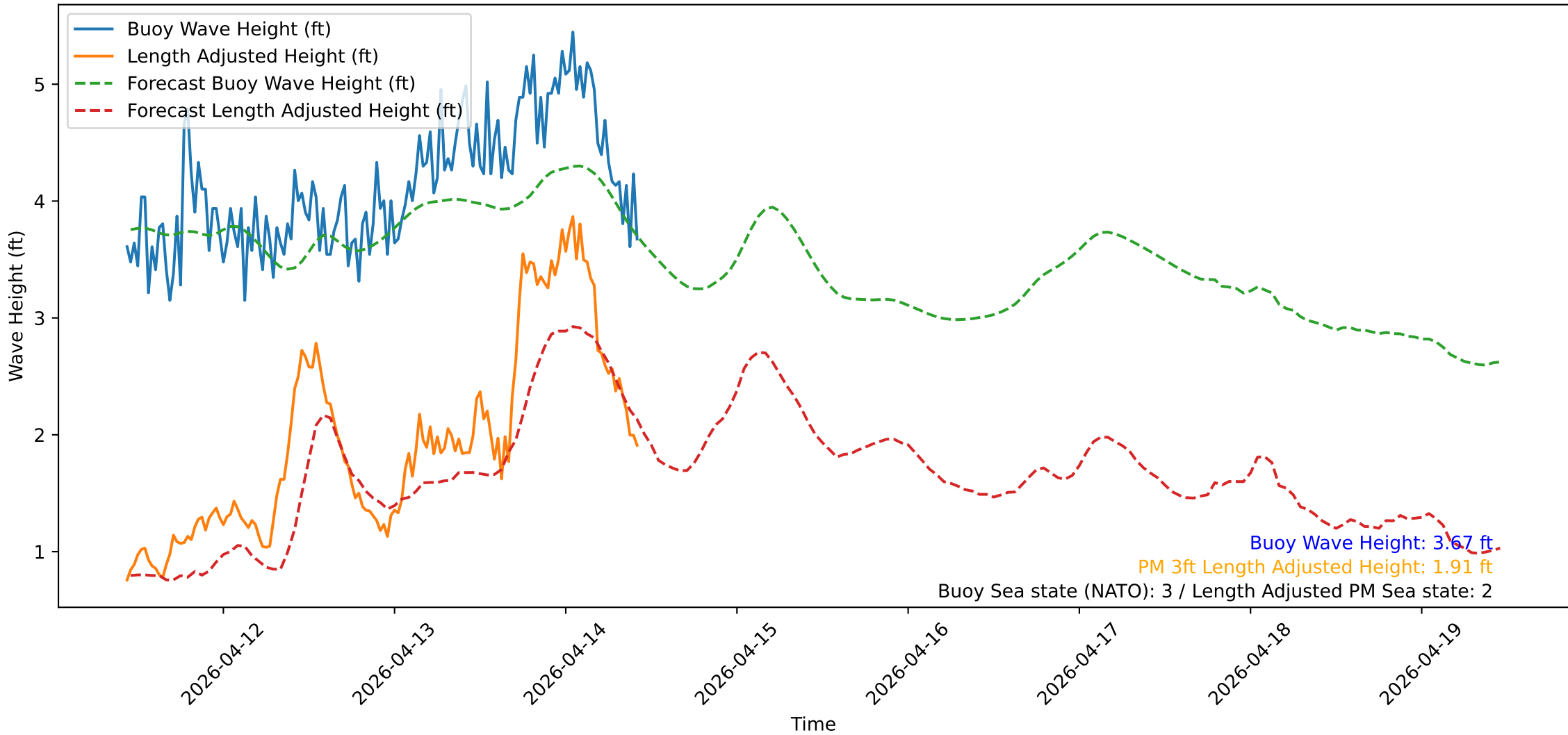
Wave Heights over Time for Oceanside Harbor at 2026-04-14 10:30:32
