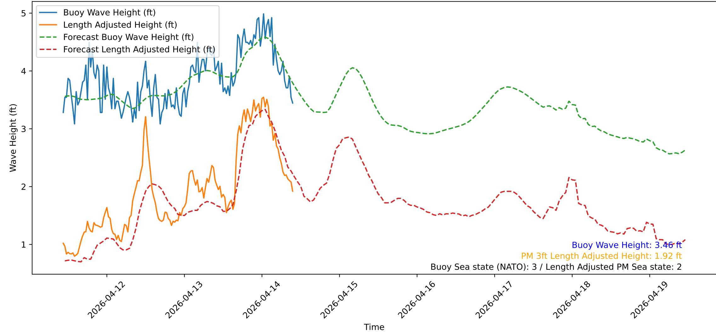
Wave Heights over Time for Green Beach at 2026-04-14 10:31:13
