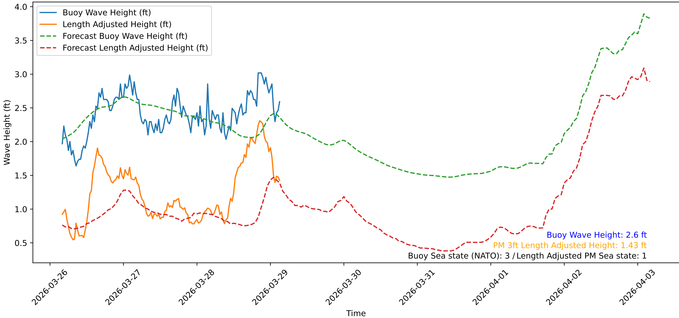
Wave Heights over Time for Red Beach at 2026-03-29 03:40:47
