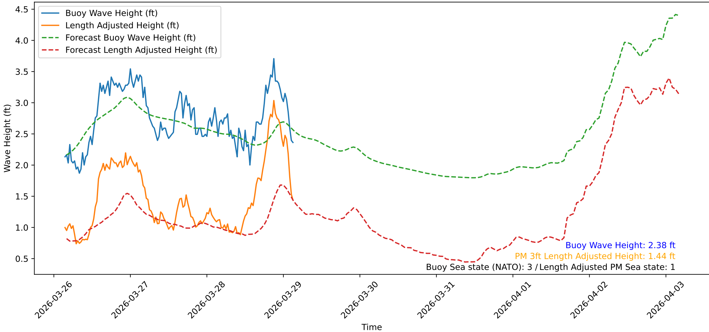
Wave Heights over Time for Green Beach at 2026-03-29 03:41:10
