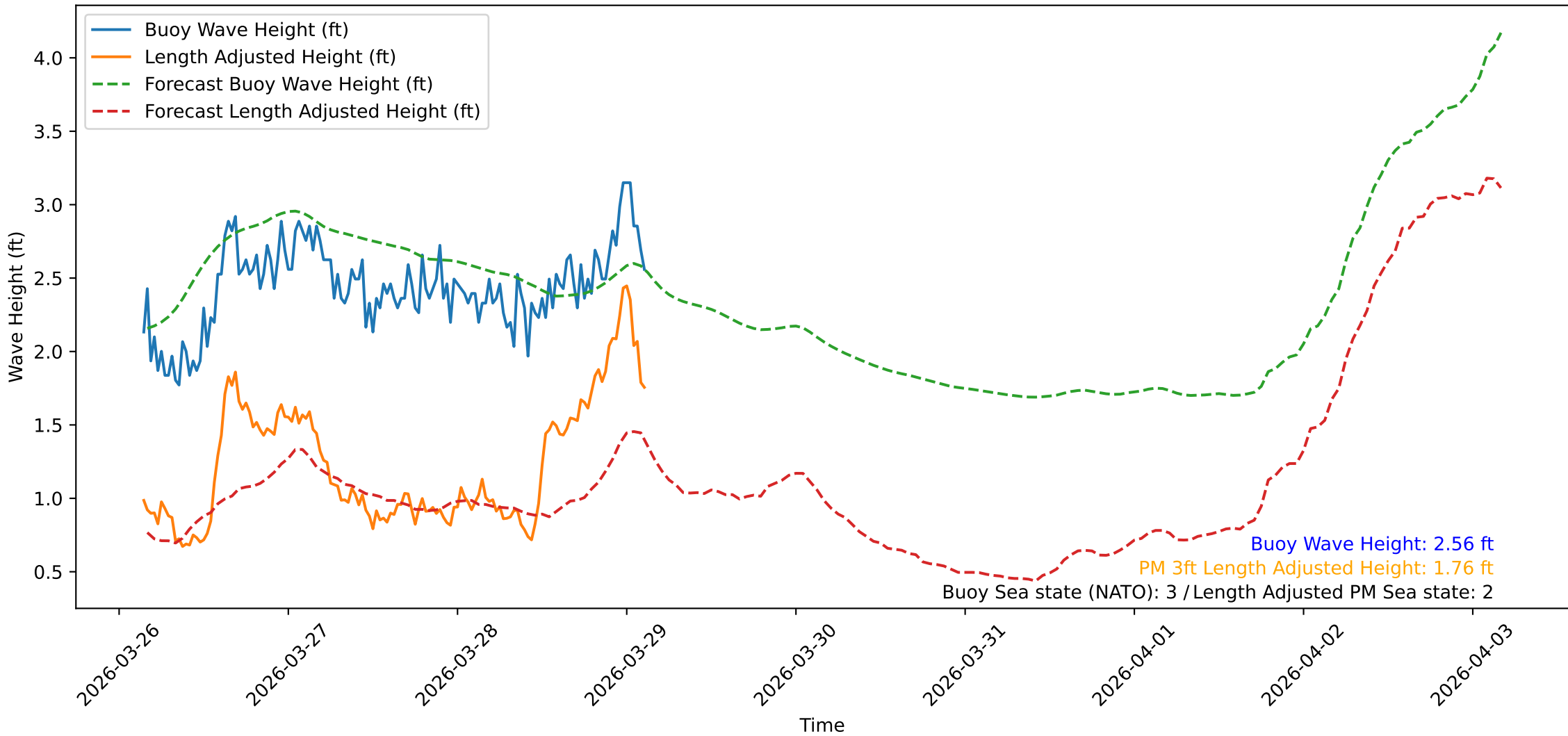
Wave Heights over Time for Oceanside Harbor at 2026-03-29 03:40:31
