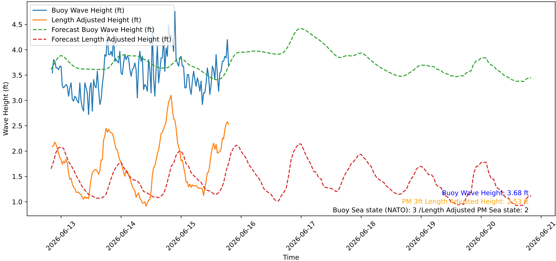
Wave Heights over Time for Red Beach at 2026-06-15 20:00:45
