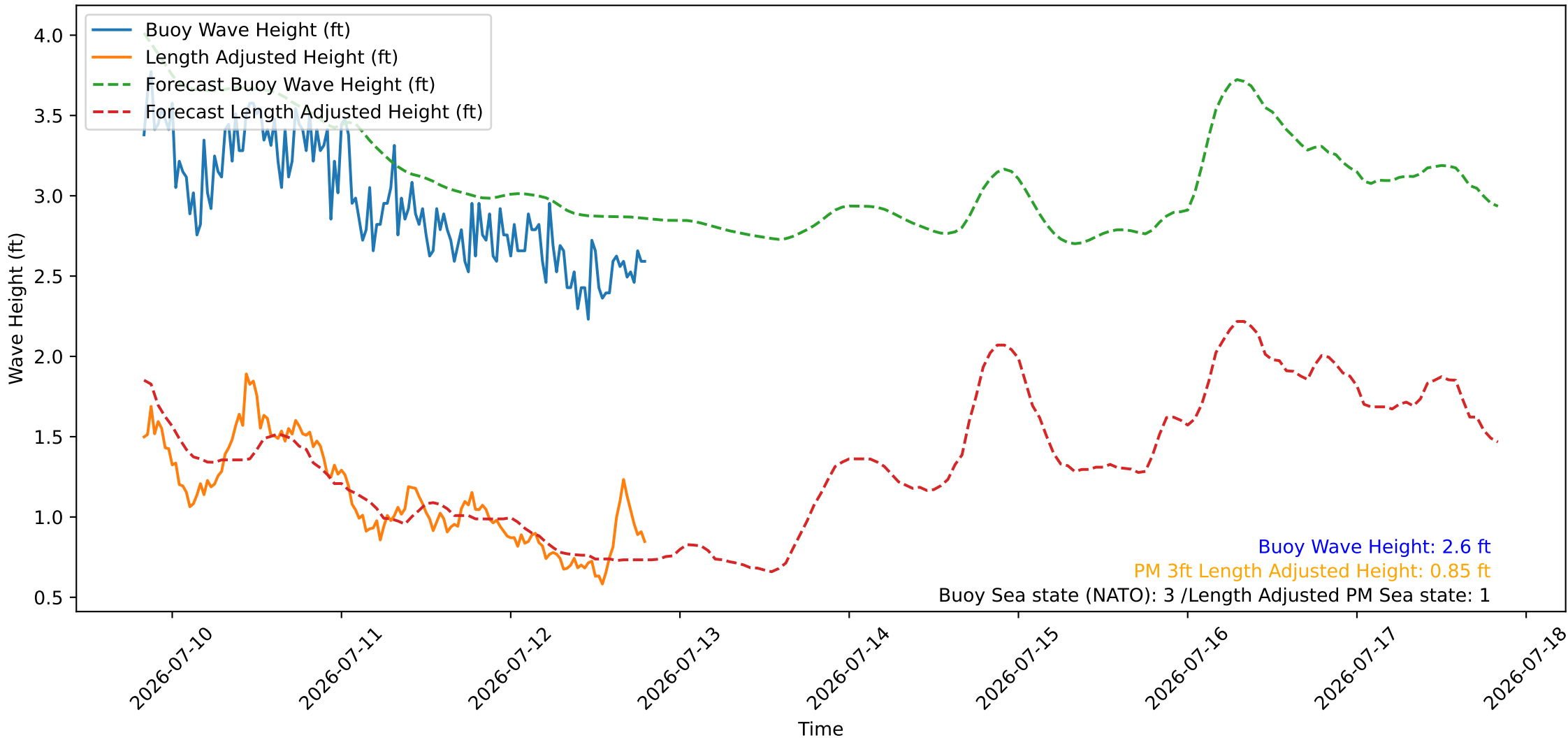
Wave Heights over Time for Green Beach at 2026-07-12 19:51:10
