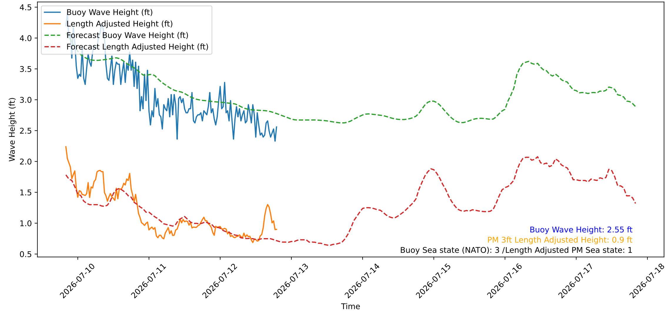
Wave Heights over Time for Oceanside Harbor at 2026-07-12 19:50:26
