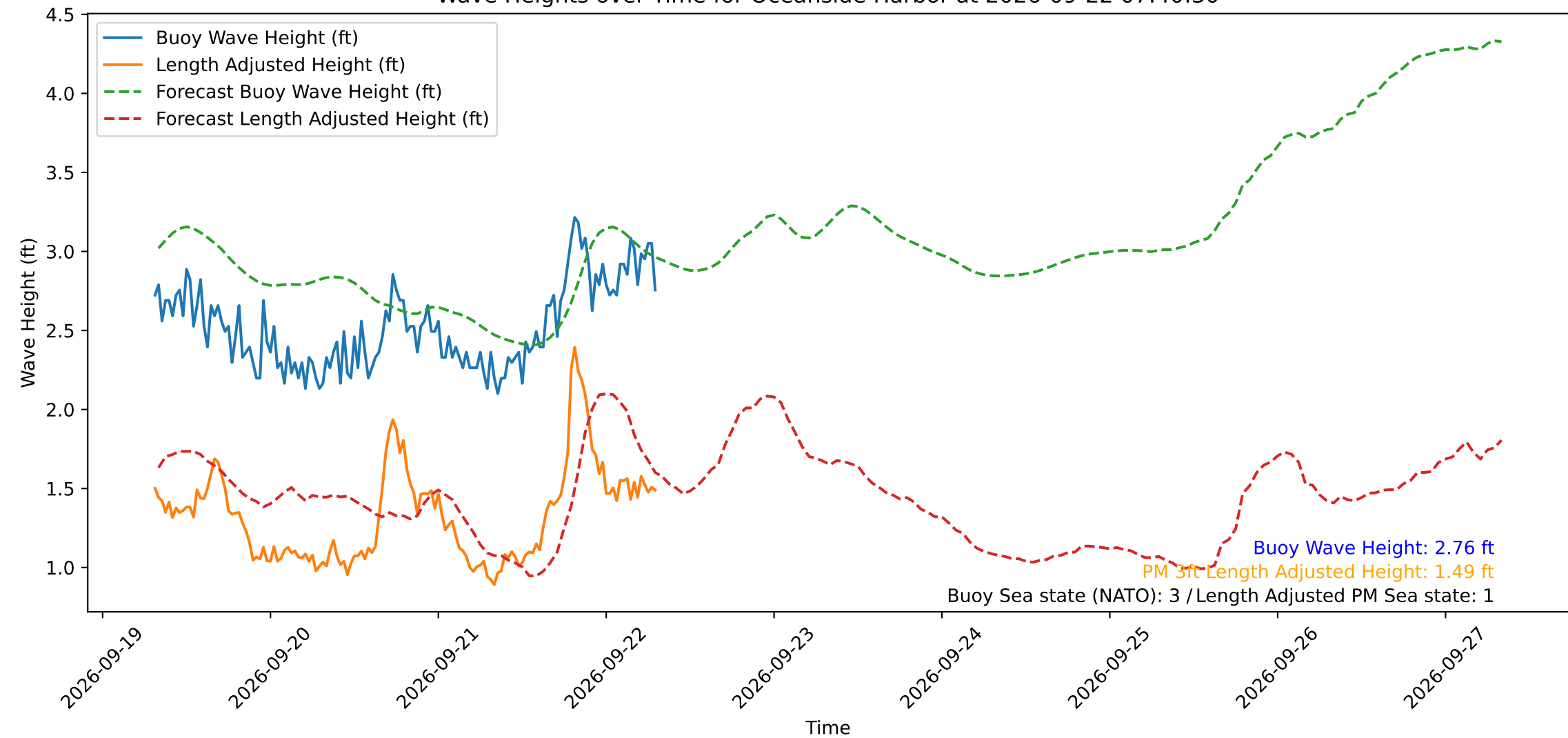
Wave Heights over Time for Oceanside Harbor at 2026-09-22 07:40:30
