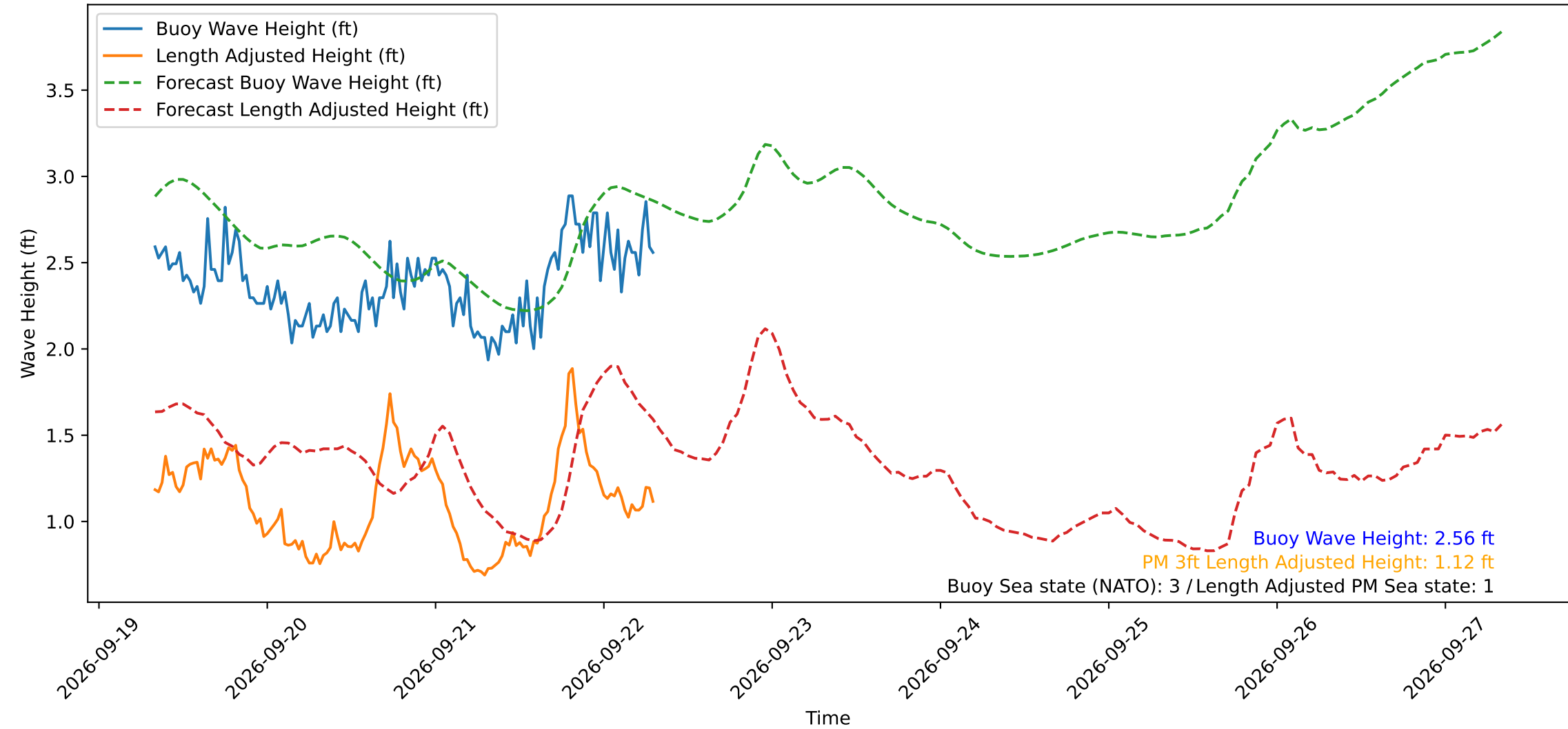
Wave Heights over Time for Red Beach at 2026-09-22 07:40:49
