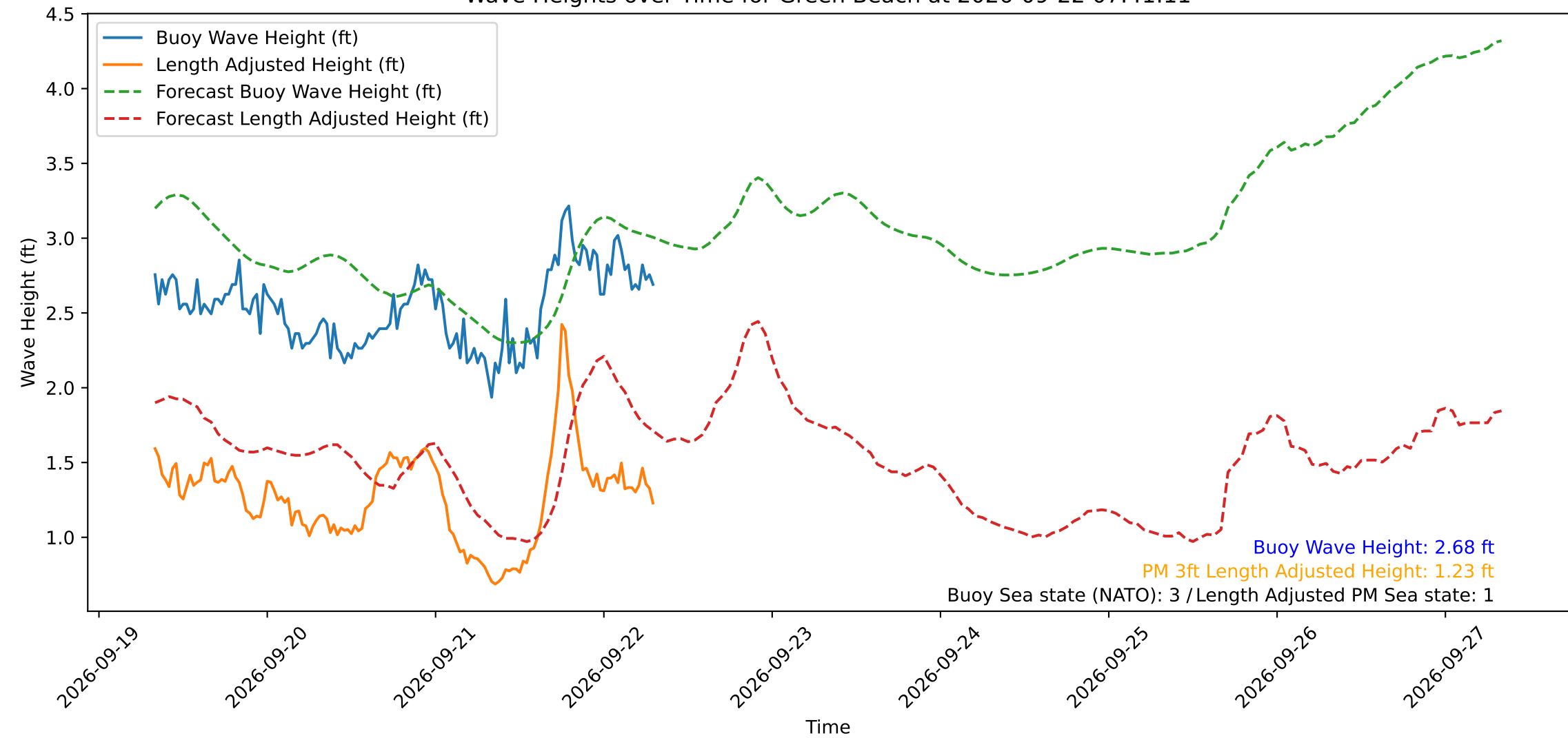
Wave Heights over Time for Green Beach at 2026-09-22 07:41:11
