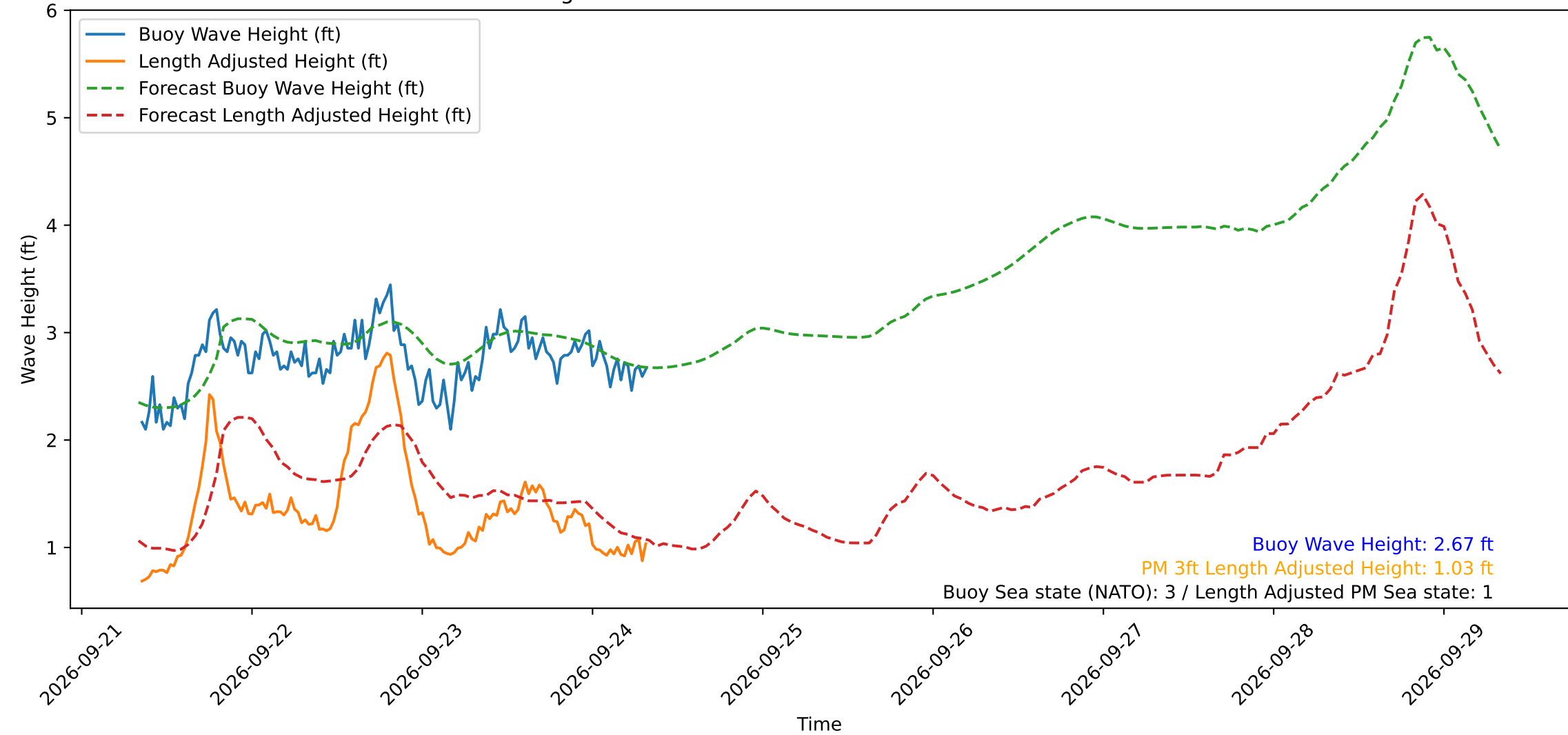
Wave Heights over Time for Green Beach at 2026-09-24 08:21:13
