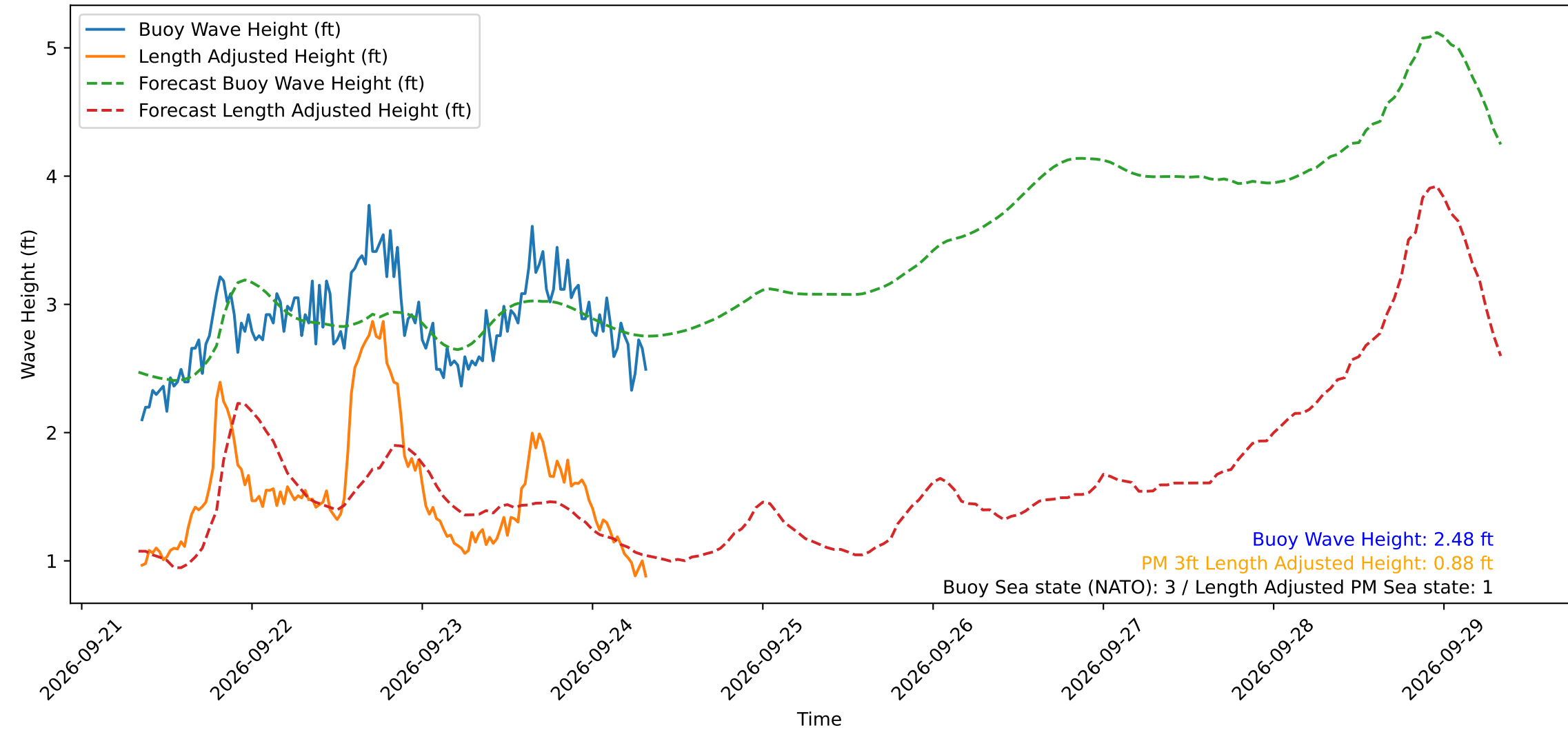
Wave Heights over Time for Oceanside Harbor at 2026-09-24 08:20:29
