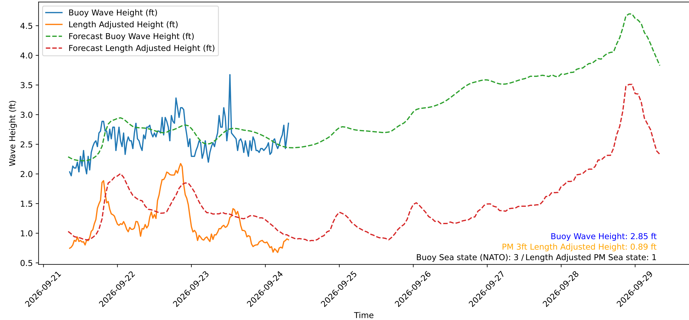
Wave Heights over Time for Red Beach at 2026-09-24 08:20:50
