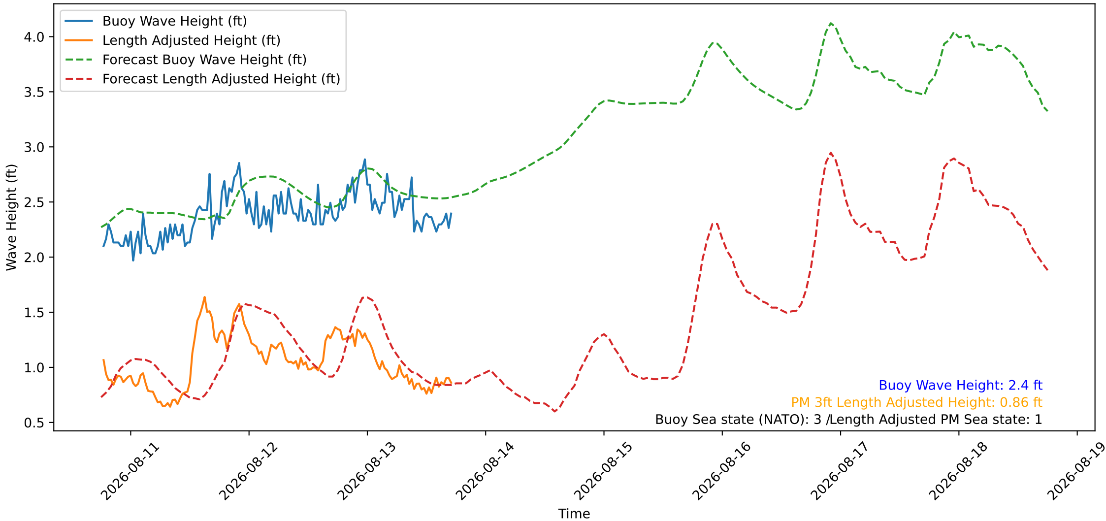
Wave Heights over Time for Red Beach at 2026-08-13 18:20:47
