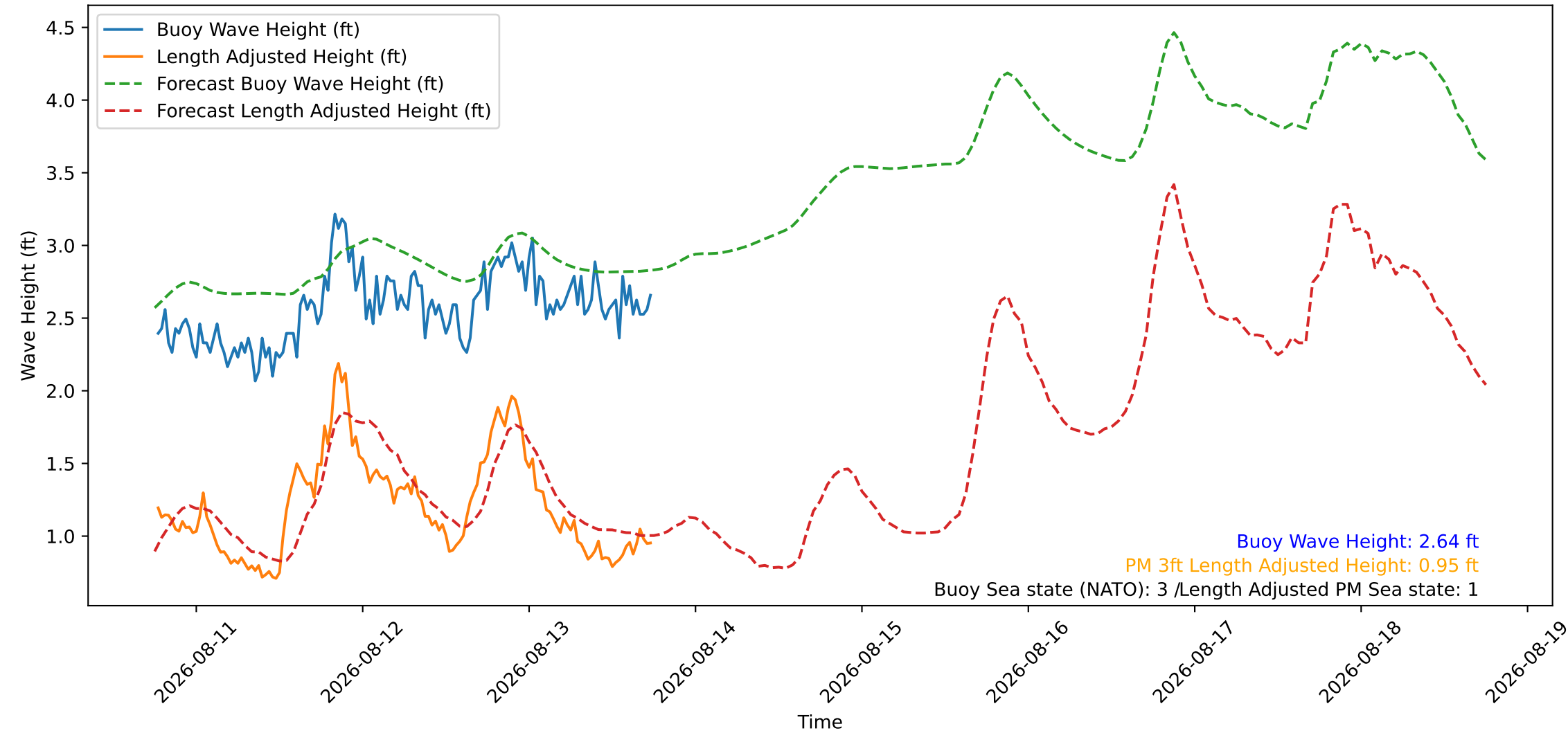
Wave Heights over Time for Green Beach at 2026-08-13 18:21:09
