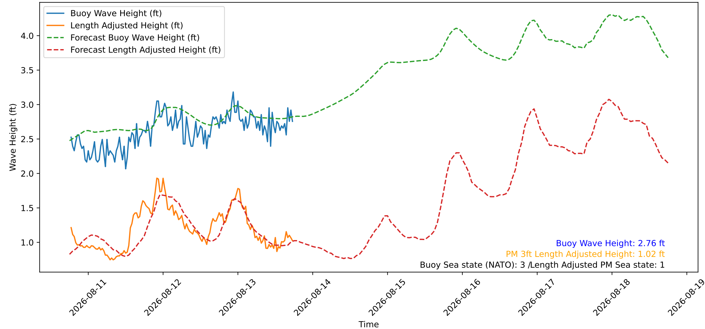
Wave Heights over Time for Oceanside Harbor at 2026-08-13 18:20:26
