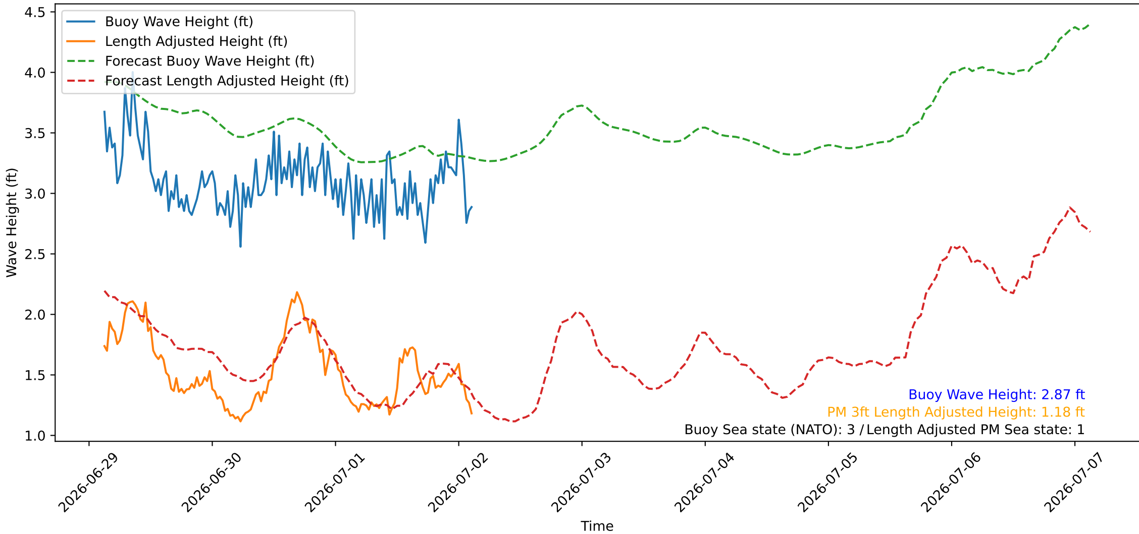
Wave Heights over Time for Oceanside Harbor at 2026-07-02 03:10:26
