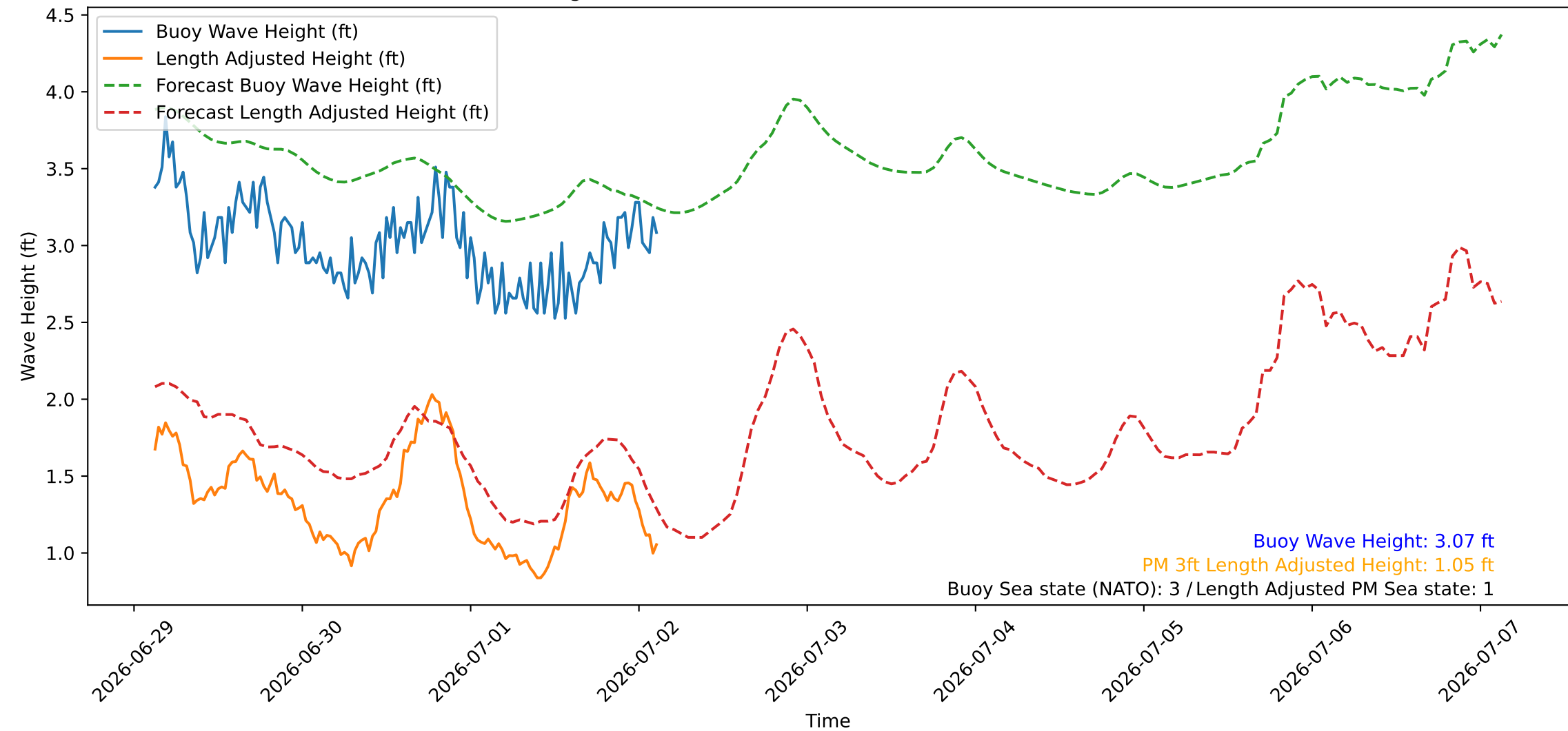
Wave Heights over Time for Green Beach at 2026-07-02 03:11:07
