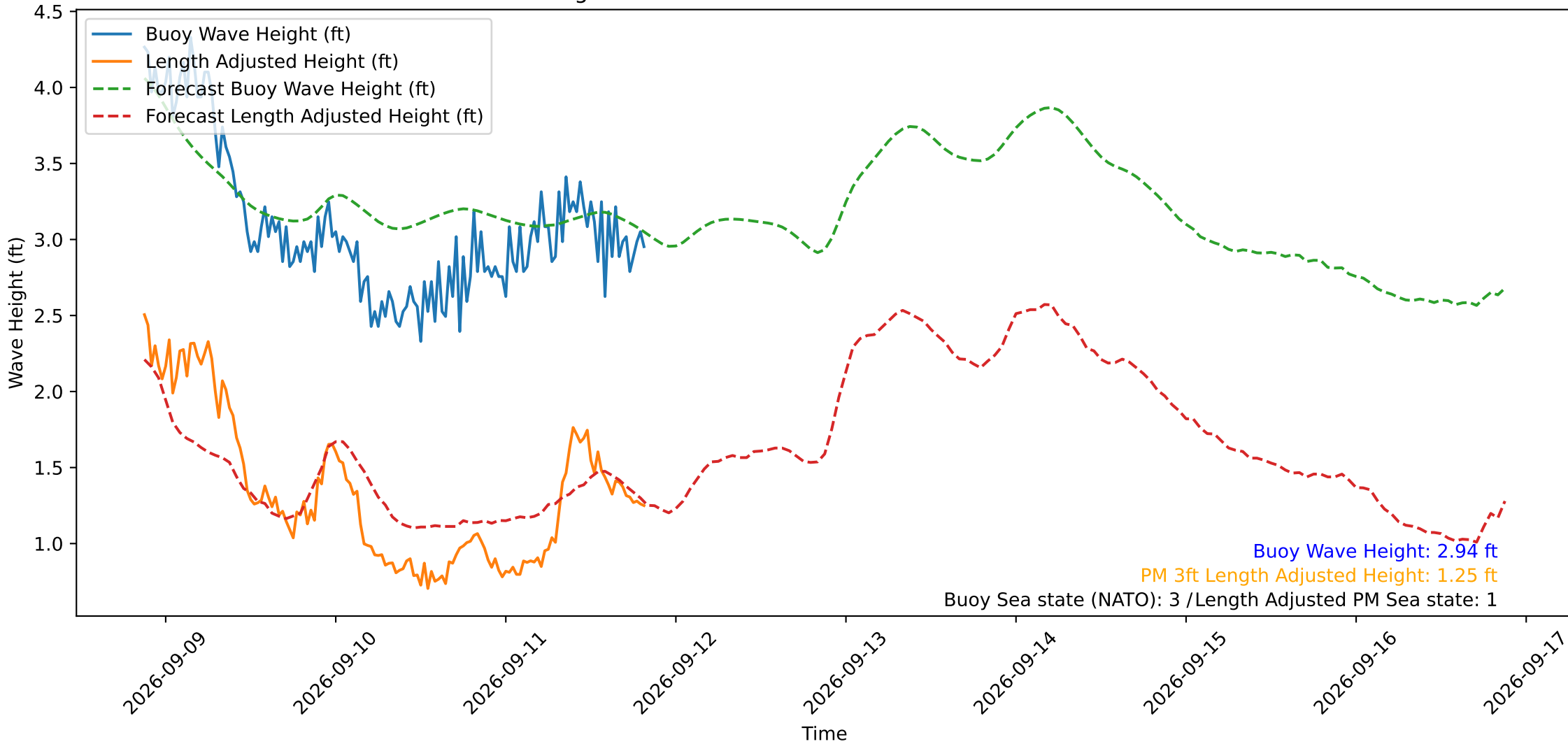
Wave Heights over Time for Red Beach at 2026-09-11 20:30:49
