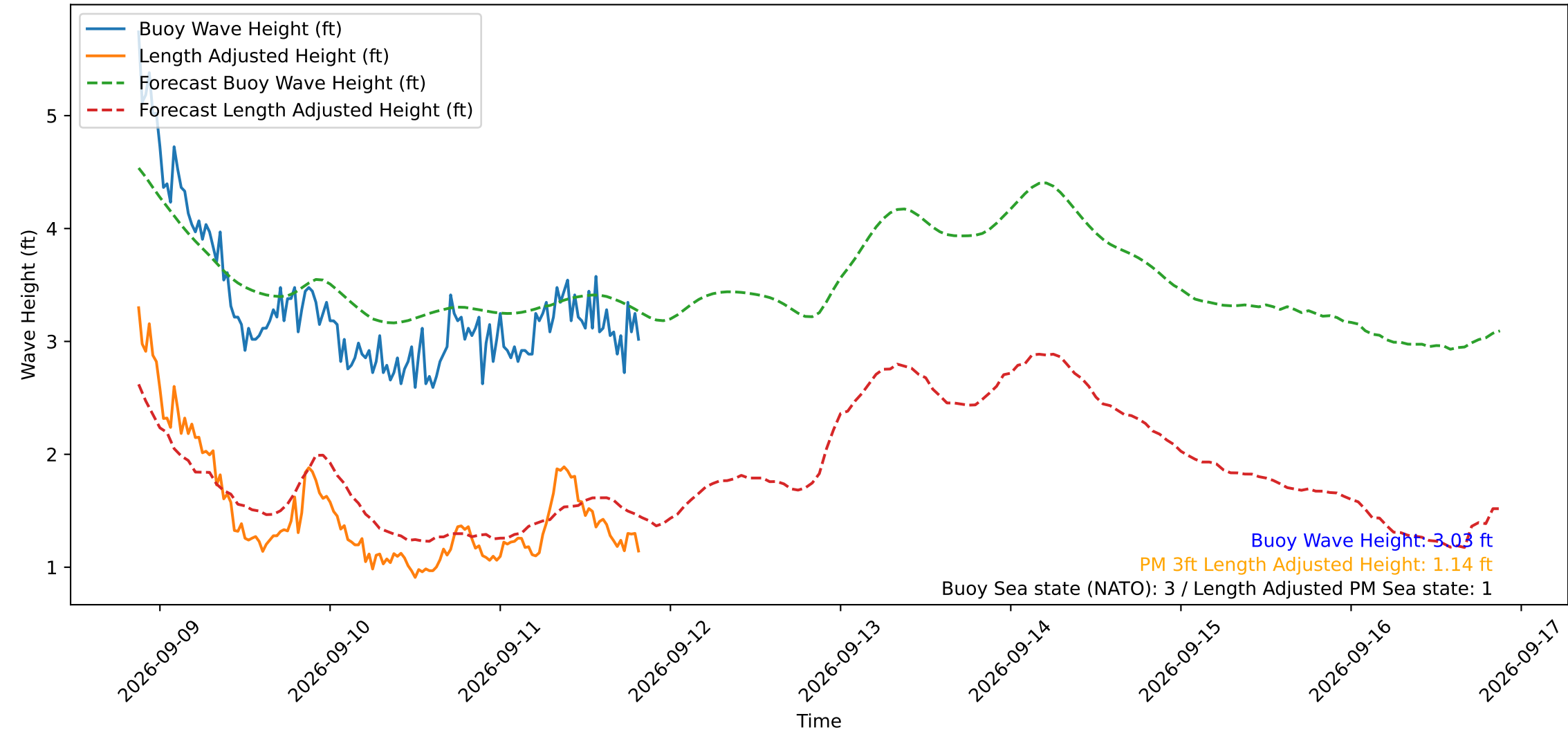
Wave Heights over Time for Green Beach at 2026-09-11 20:31:12
