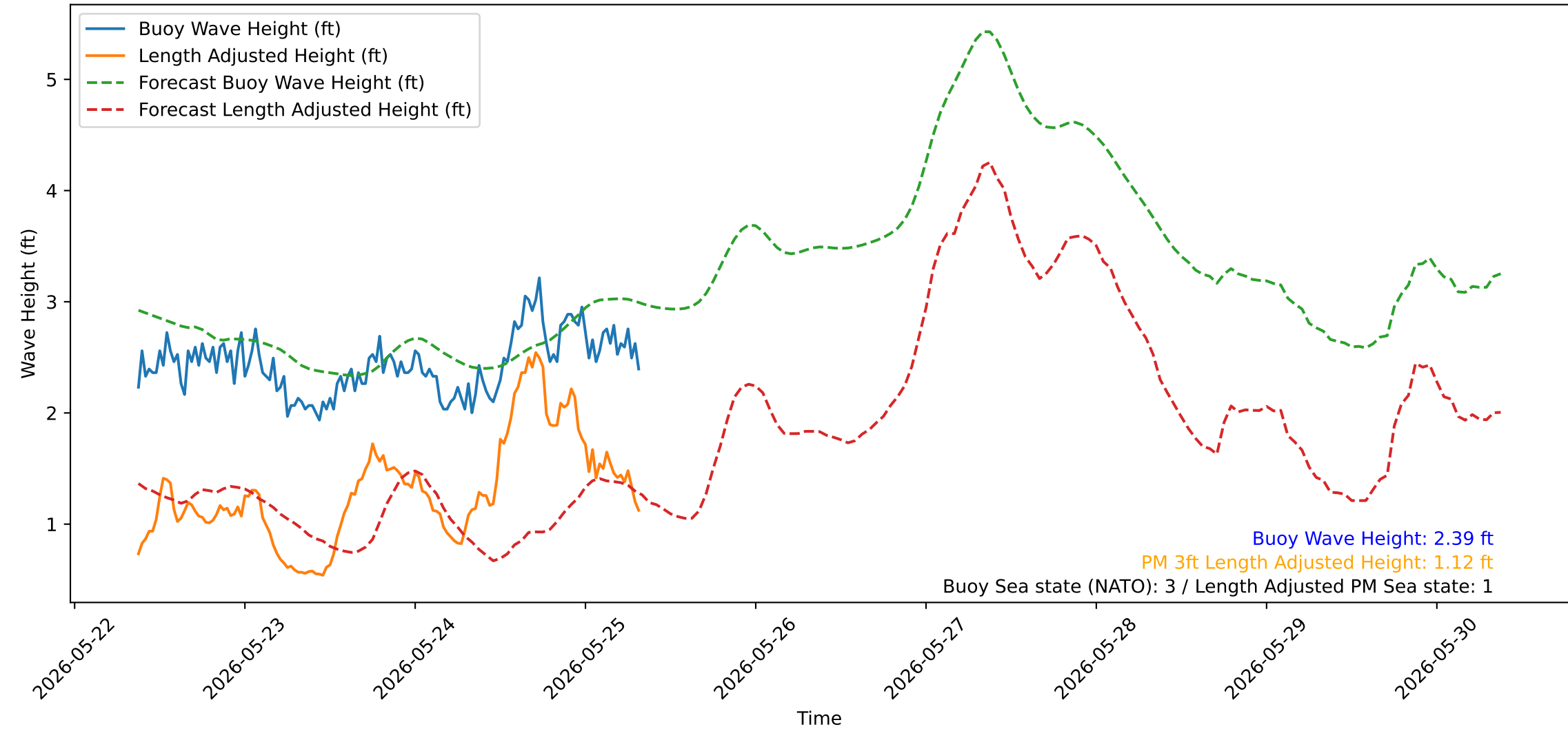
Wave Heights over Time for Red Beach at 2026-05-25 08:30:50
