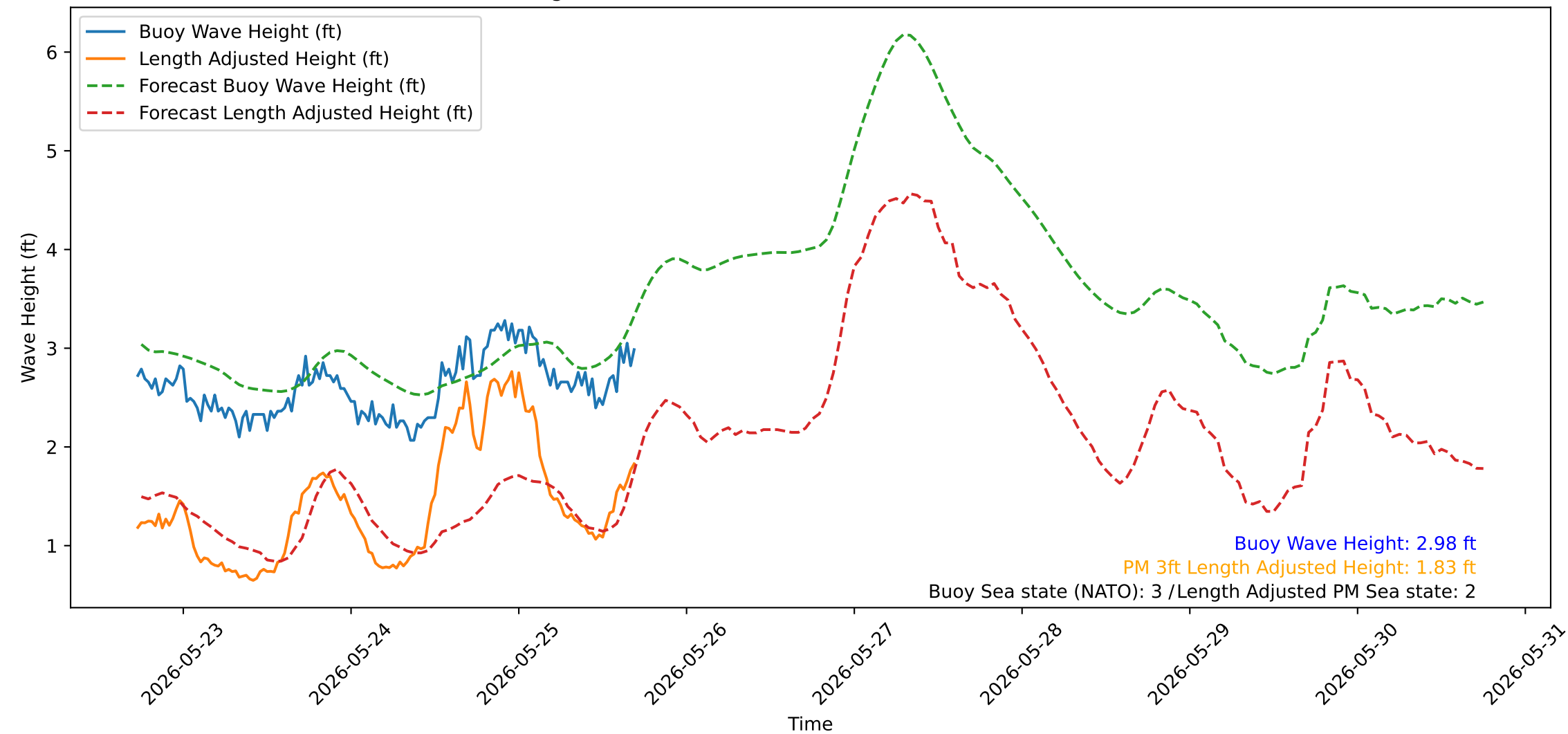
Wave Heights over Time for Green Beach at 2026-05-25 17:31:11
