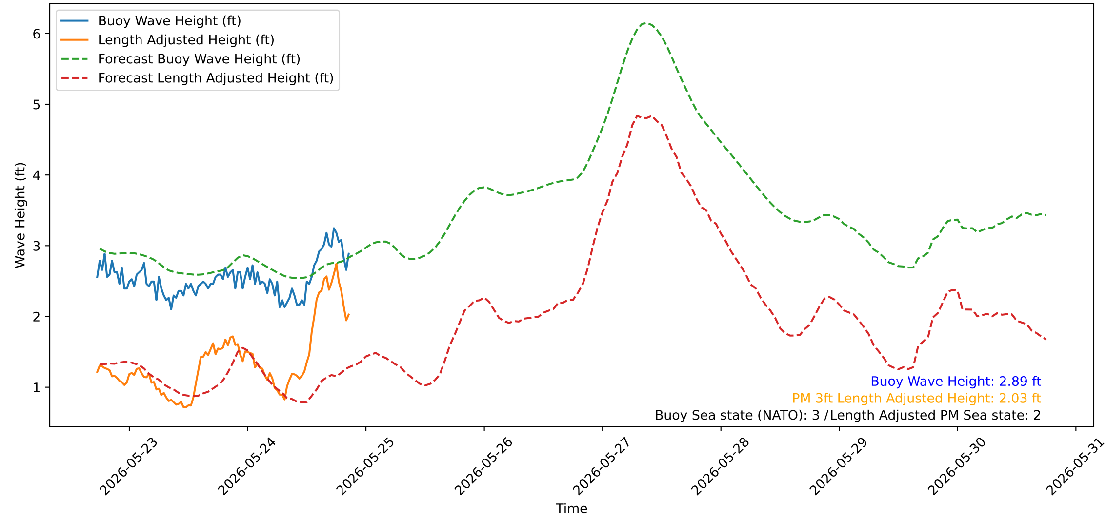
Wave Heights over Time for Oceanside Harbor at 2026-05-25 17:30:30
