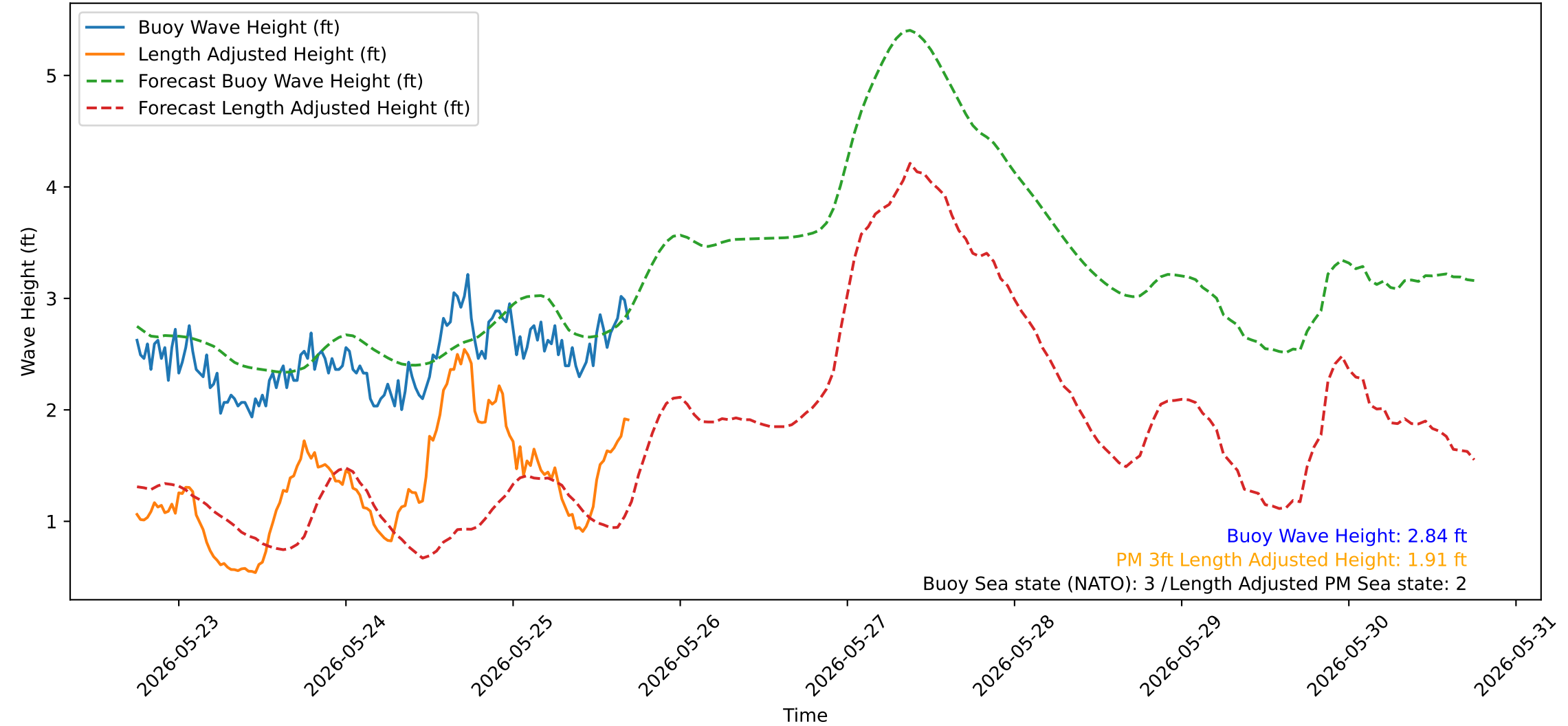
Wave Heights over Time for Red Beach at 2026-05-25 17:30:49
