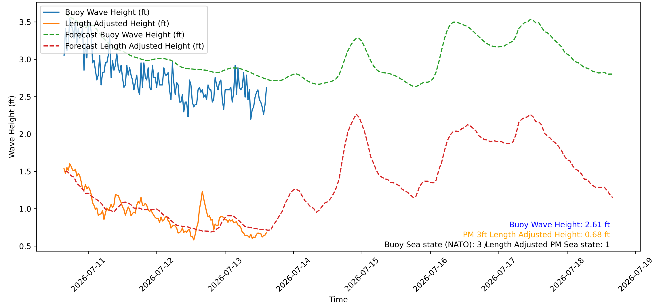
Wave Heights over Time for Green Beach at 2026-07-13 15:31:08
