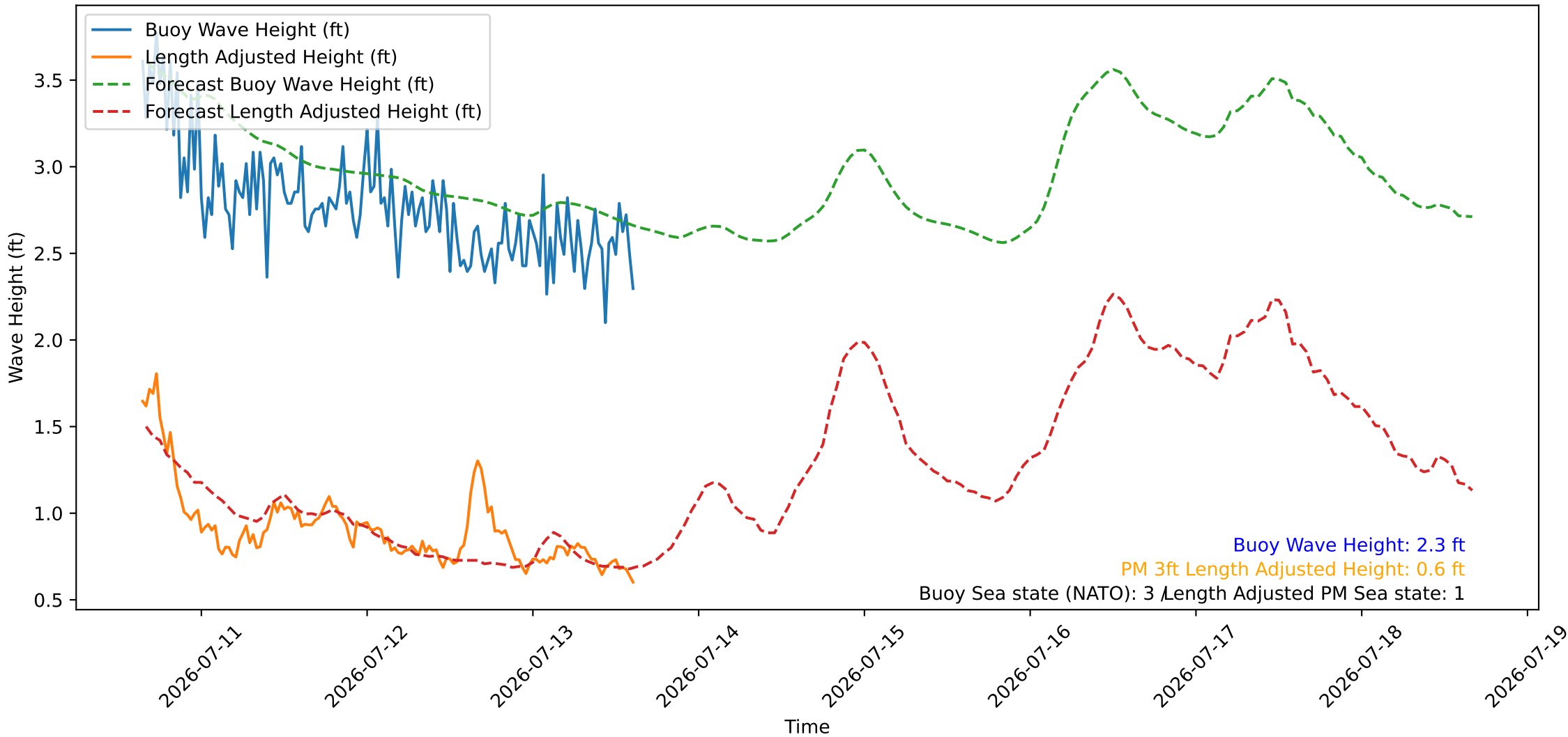
Wave Heights over Time for Oceanside Harbor at 2026-07-13 15:30:27
