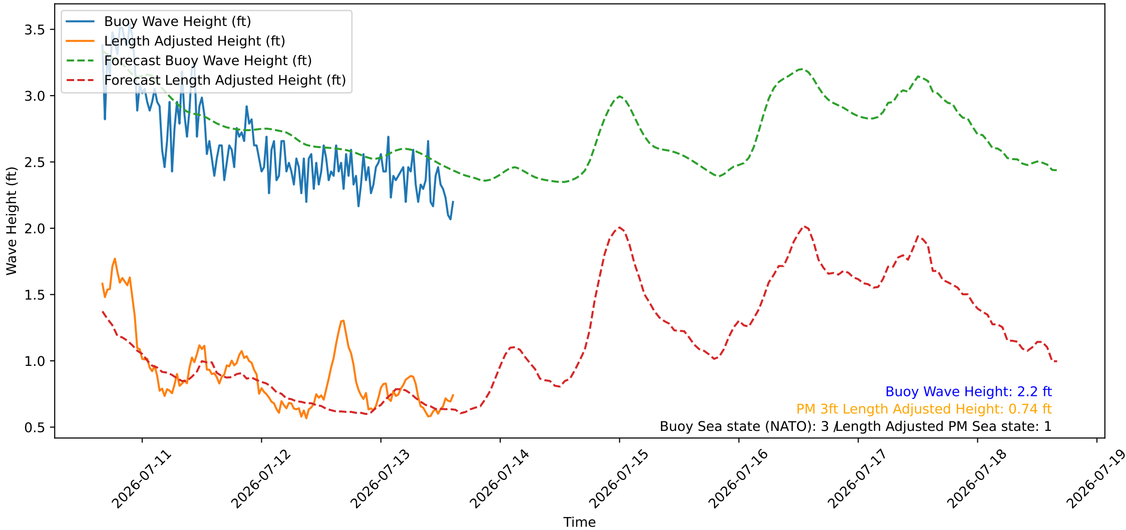
Wave Heights over Time for Red Beach at 2026-07-13 15:30:45
