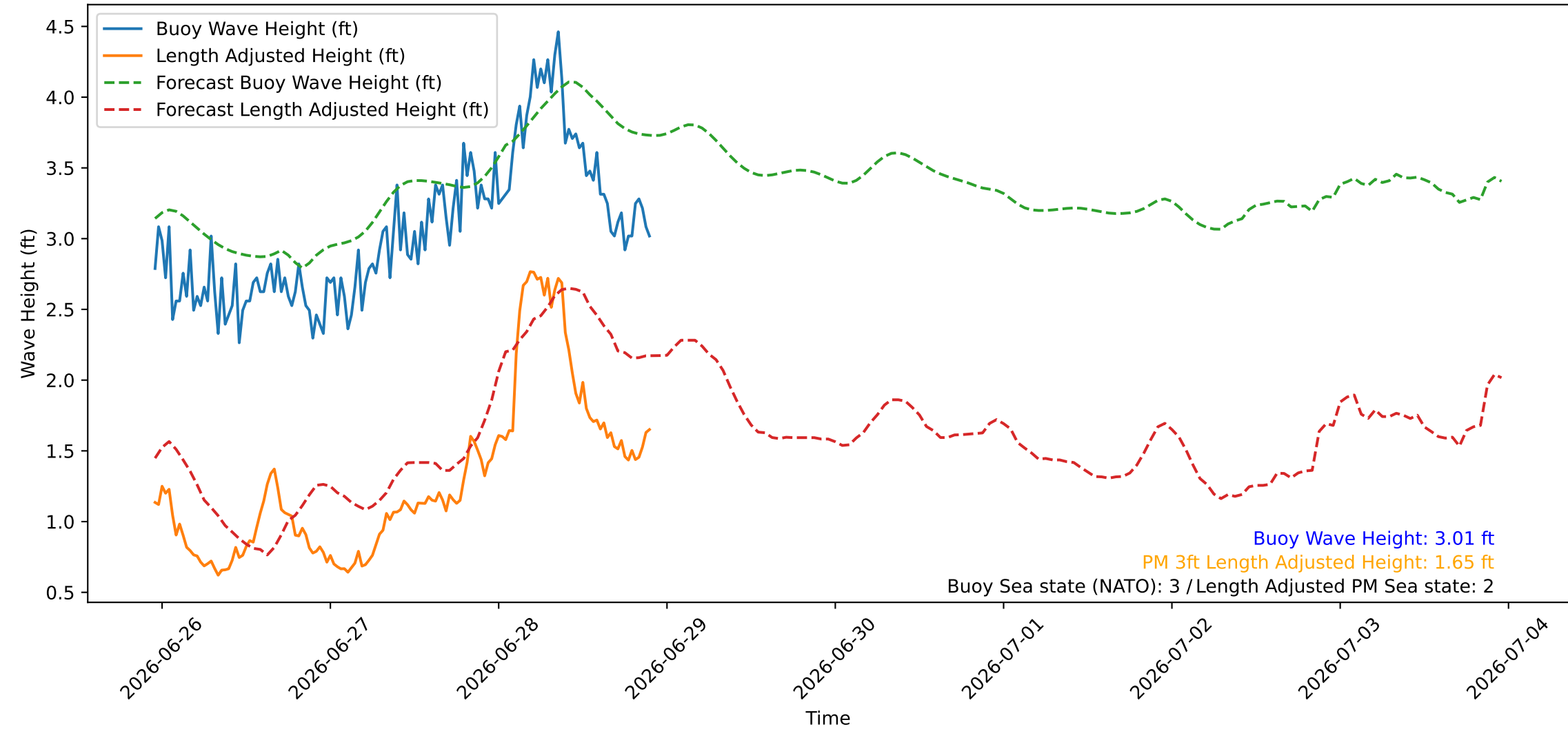
Wave Heights over Time for Red Beach at 2026-06-28 22:30:45
