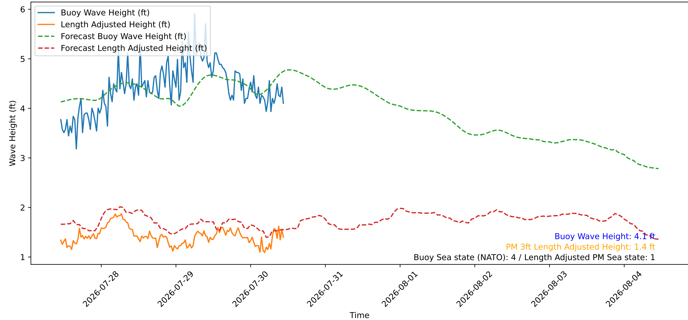
Wave Heights over Time for Oceanside Harbor at 2026-07-30 11:10:27
