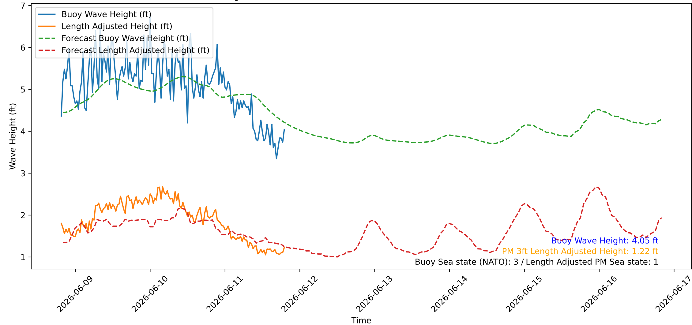
Wave Heights over Time for Oceanside Harbor at 2026-06-11 19:40:26
