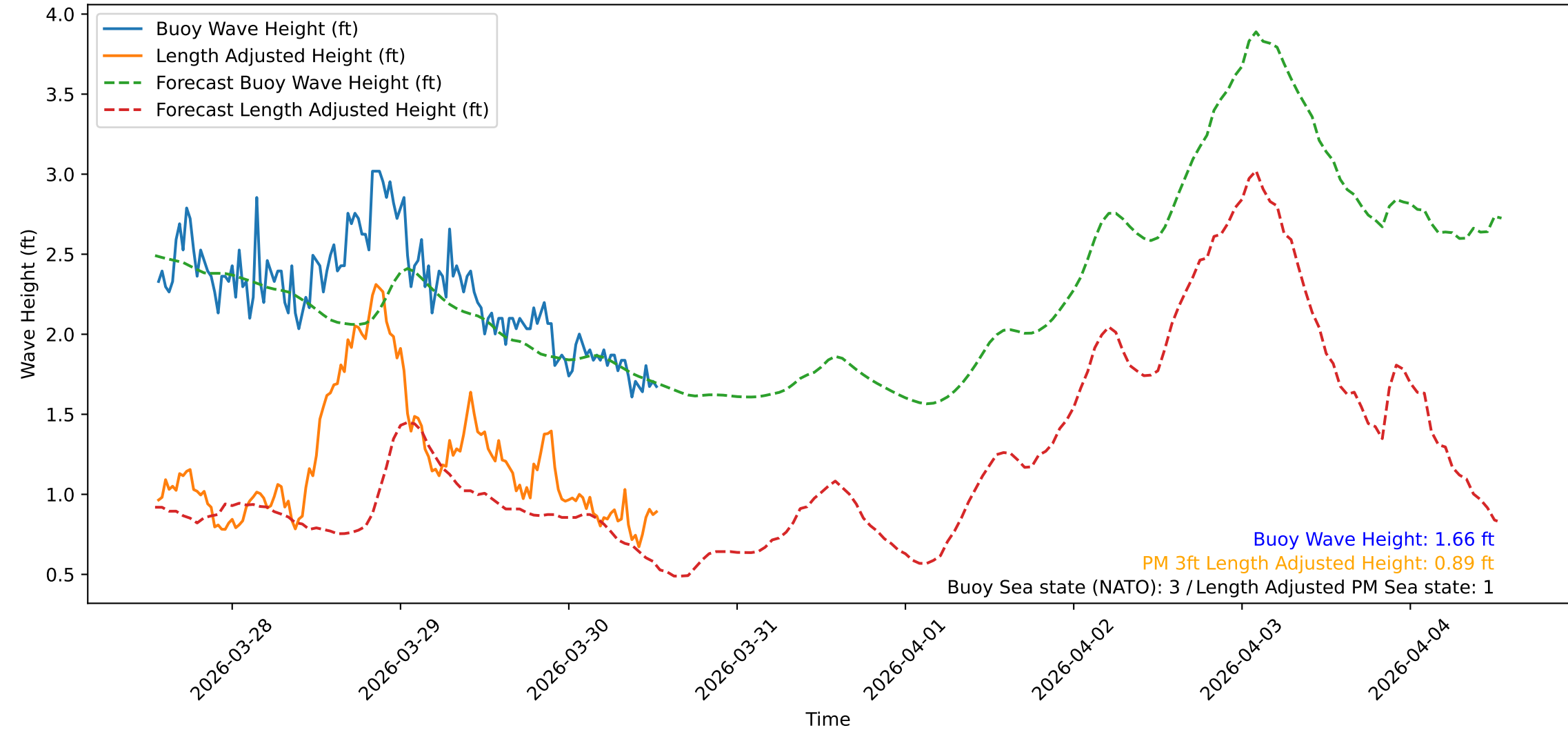
Wave Heights over Time for Red Beach at 2026-03-30 13:20:47
