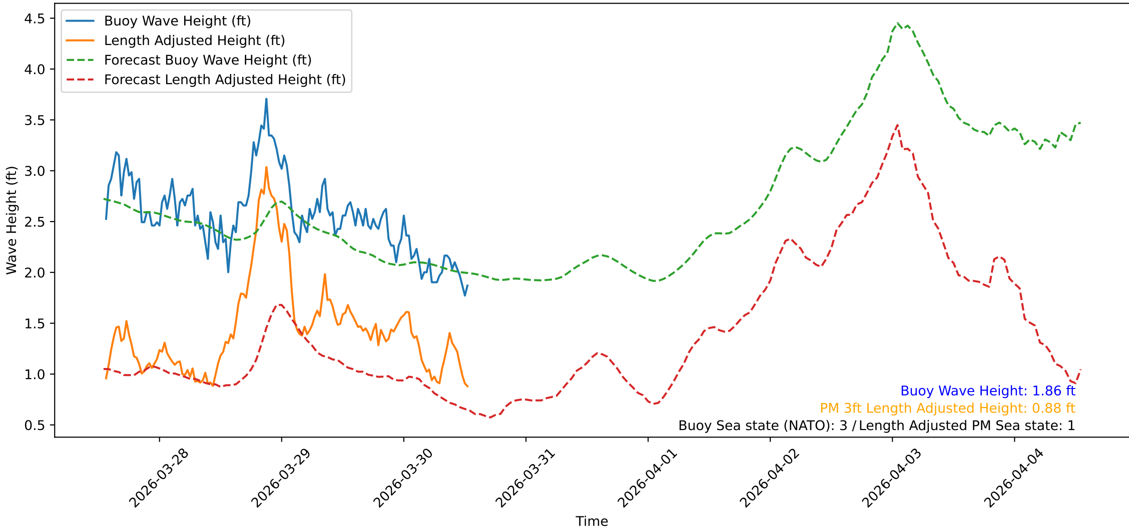
Wave Heights over Time for Green Beach at 2026-03-30 13:21:09
